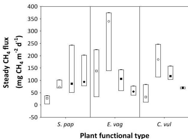
Figure 3.3. Box plot of seasonal steady CH 4 fluxes from the three plant functional types: S. papillosum , E. vaginatum , and C. vulgaris . Median is represented by the symbol (open square = spring, open circle = summer, closed square = autumn, closed circle = winter), with the box representing the inter-quartile range and the whiskers indicating the full range. Data for S1 cores only.
