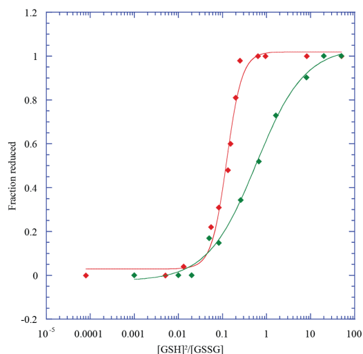
Fig. 2 Two fits shown using the Hill equation, PDI a , lysine 14 (green) with a redox potential of -144.43 \pm 0.34 \text{ mV} and DsbA serine 43 (red) with a redox potential of -124.63 \pm 0.98 \text{ mV} .
