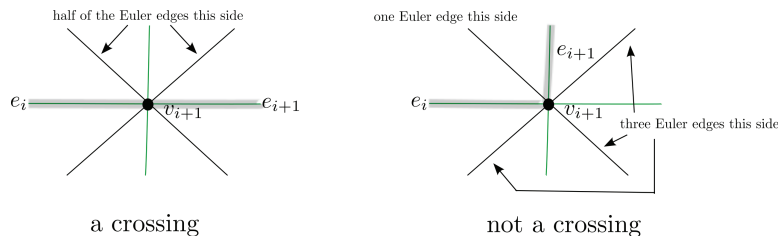
Figure 19: Detecting crossings.
