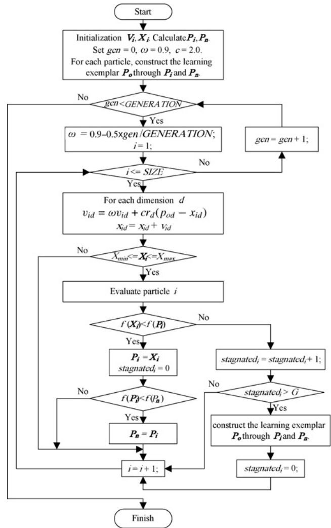
Fig. 2. Flowchart of an OLPSO algorithm.
