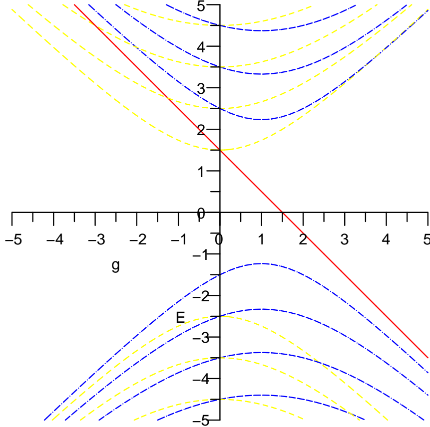
Figure 1: The energy E as a function of the coupling constant g for E_0 (solid red curve), E_{asym}^{\pm}(n) (dotted blue curves) and E_{sym}^{\pm}(n) (dashed yellow curves).
