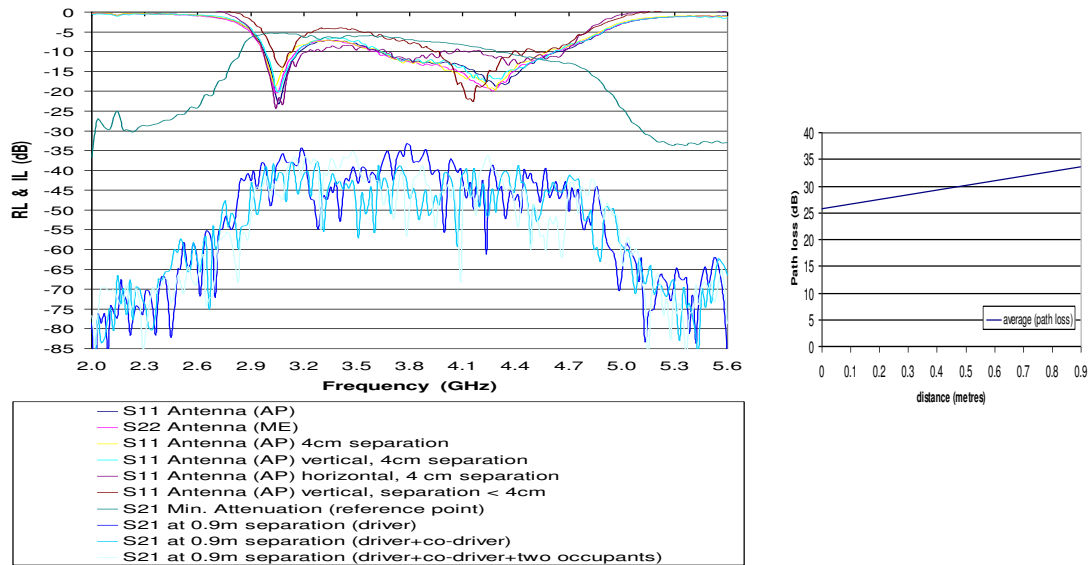
Figure 3 - a) Antenna matching (RL) and channel path loss (IL) b) path loss
