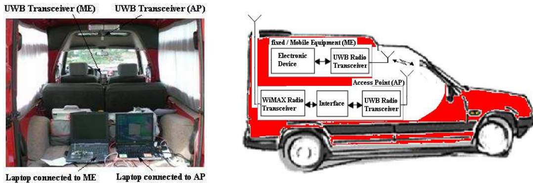
Figure 1 - The experimental set up in a typical in-car wireless channel
