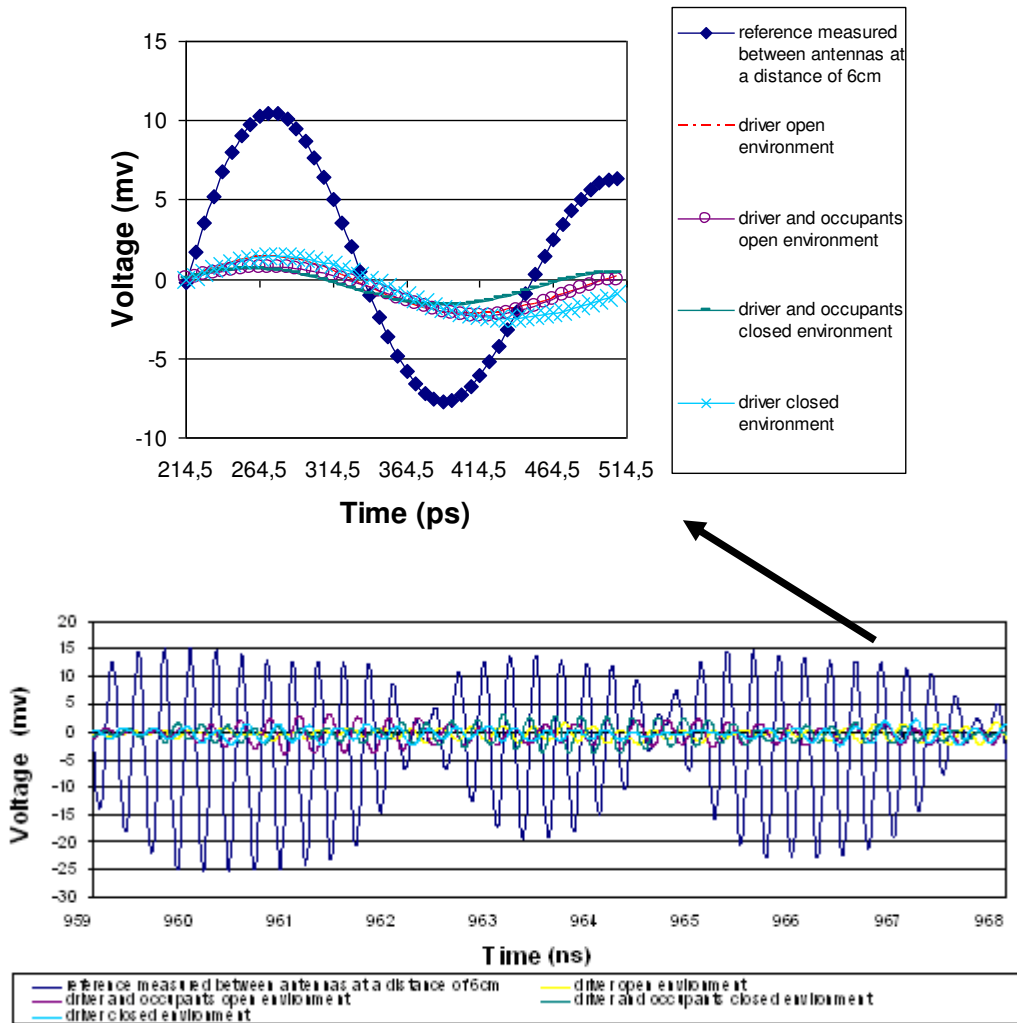
Figure: 5 Transmitted and received UWB pulse over an in-car wireless channel, (top) over a time 214-515ps and (bottom) in wider observation over 959-968ns.
