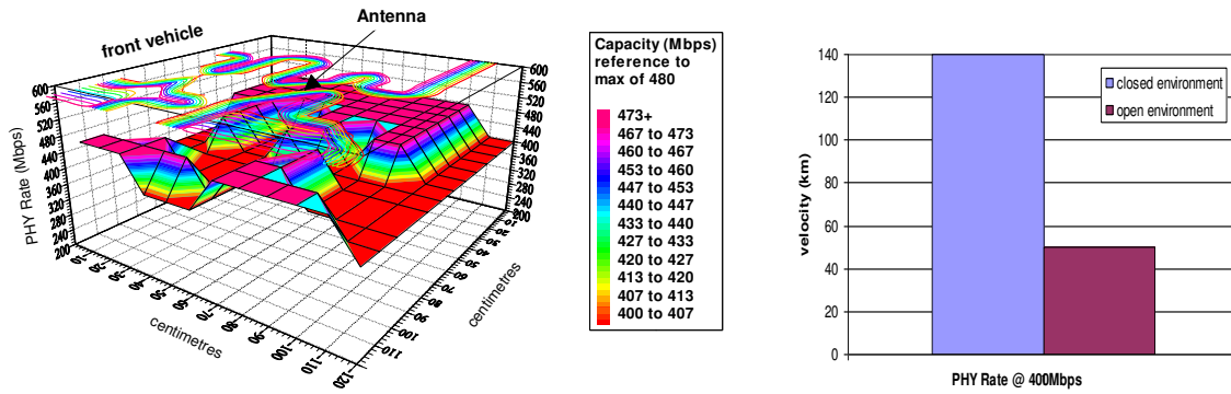
Figure 9 –The PHY Rate achievable a) in a closed environment and b) according to velocity.
