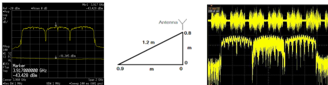
Figure 2 – a) Spectrum Analyzer PSD b) AP location c) Oscilloscope waveform
