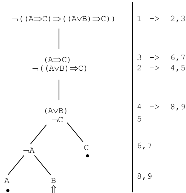
Figure 1: Semantic Tableau Example
