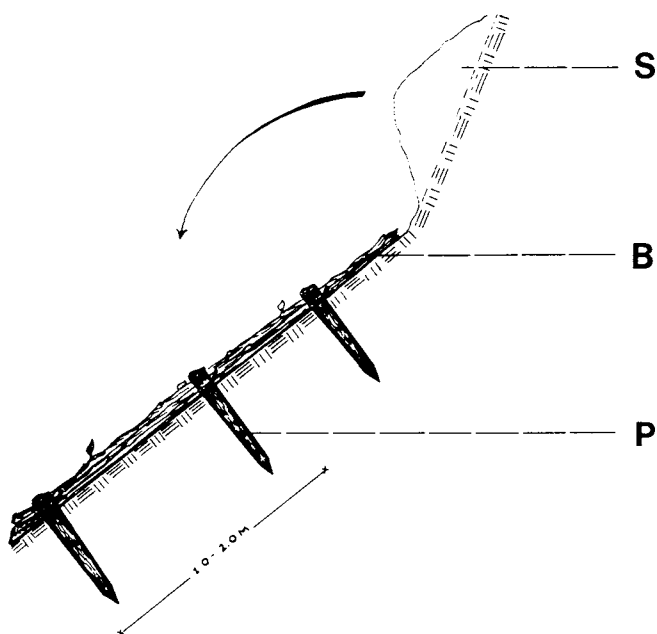
Figure 31. The brush matting technique. S = soil; B = brushwood; P = peg. (Weidelt 1975)
