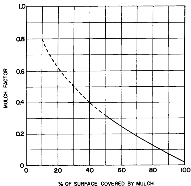
Figure 29. Effect of plant residue mulch on soil loss. Mulch factor is the ratio of encountered soil loss to corresponding loss without mulch. (Wischmeier 1973)
