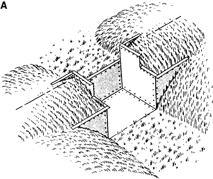
Prefabricated metal
