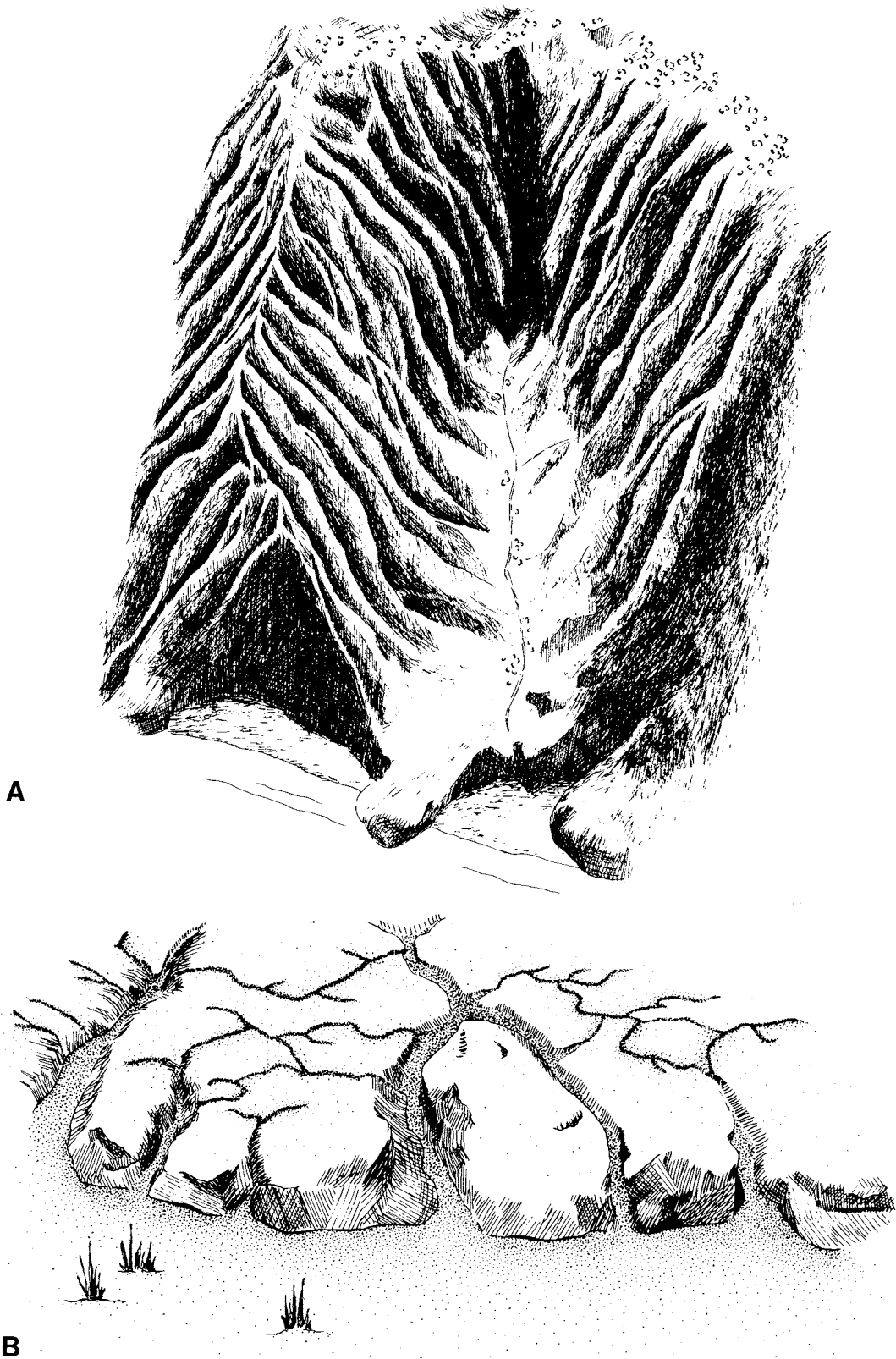
Figure 1. Schematic illustrations of major forms of erosion by water. A. Gully erosion (Scale: 1 cm = 10 or more meters); B. Rill and interrill erosion (Scale: 1 cm = 1 m); C. Tunnel erosion (Scale: 1 cm = 1 m); D. Pedestal erosion (Scale: 1 cm = 10 cm).
