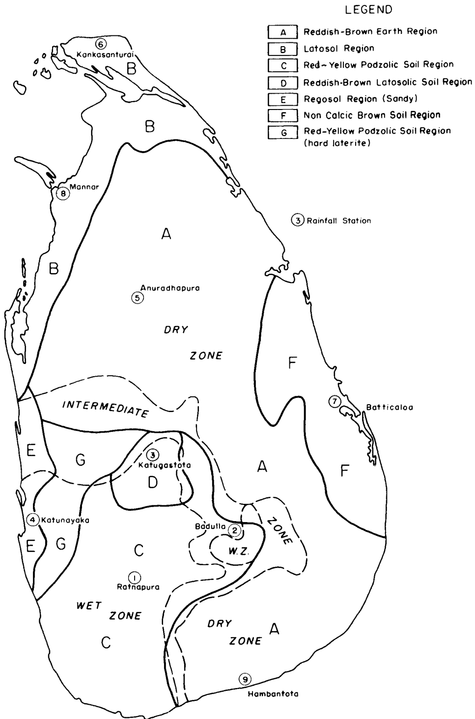
Map 9. Agroclimatic zones and major soil regions in Sri Lanka. (After Joshua 1977)
