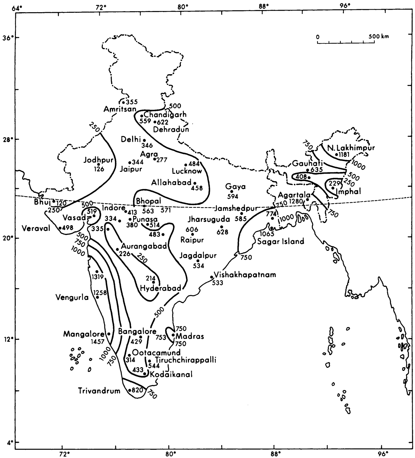
Map 26. Isoerodent map of India. (CSWCRTI 1977)
