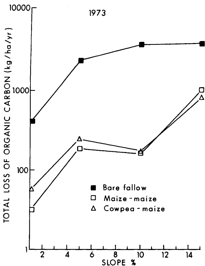
Figure 14. Total loss of organic carbon in eroded sediments, 1973. (Lal 1976d)
