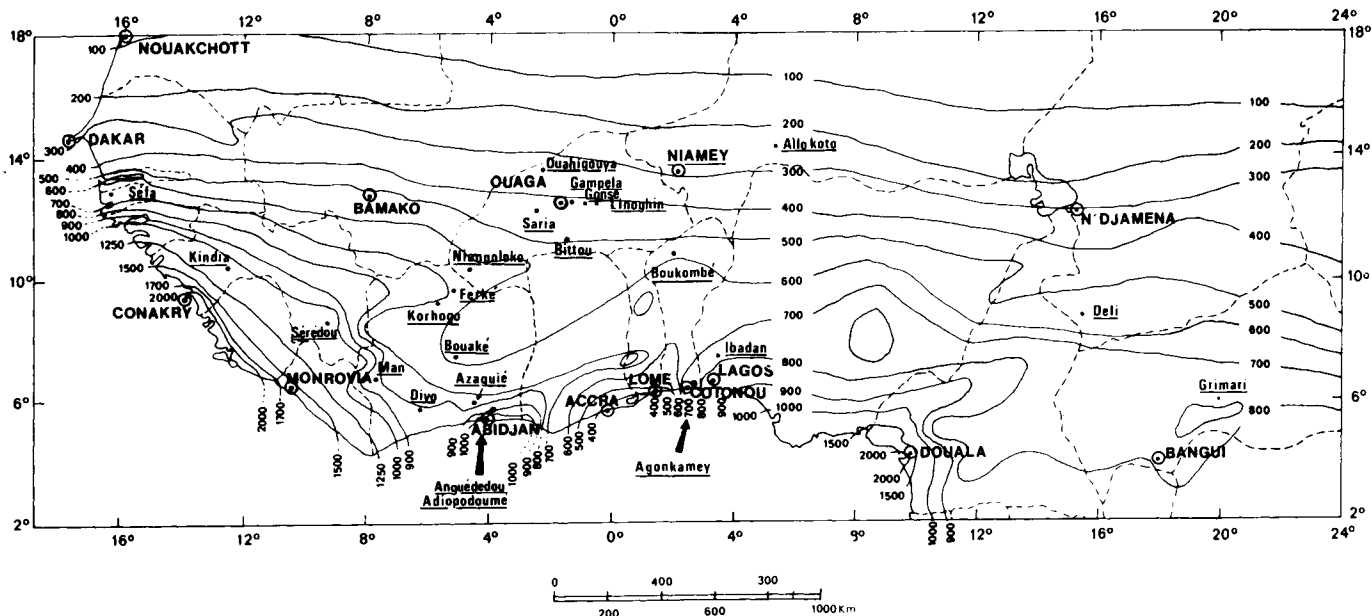
Map 27. Isoerodent map of west and central Africa. (Roose 1977c)
