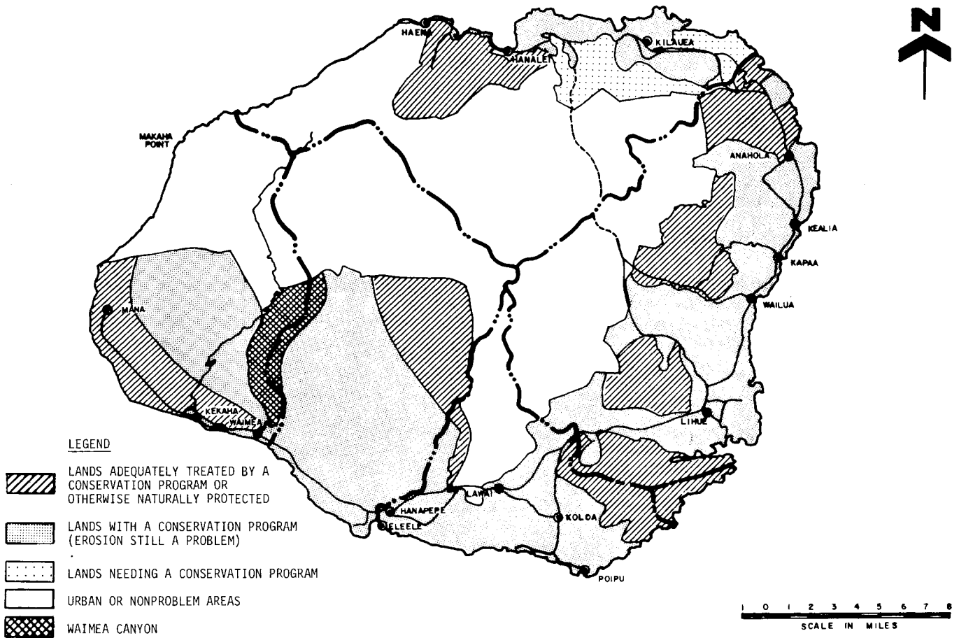
Map 13. Estimated erosion status of the island of Kauai, Hawaii. (Technical Committee on Nonpoint Source Pollution Control 1978)
