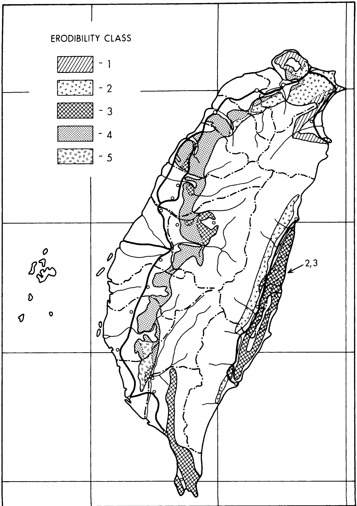
Map 29. Relative erodibility of Taiwan slopeland soils. Classes 1-5 are in increasing order of erodibility. (JCRR-MARDB 1977)
