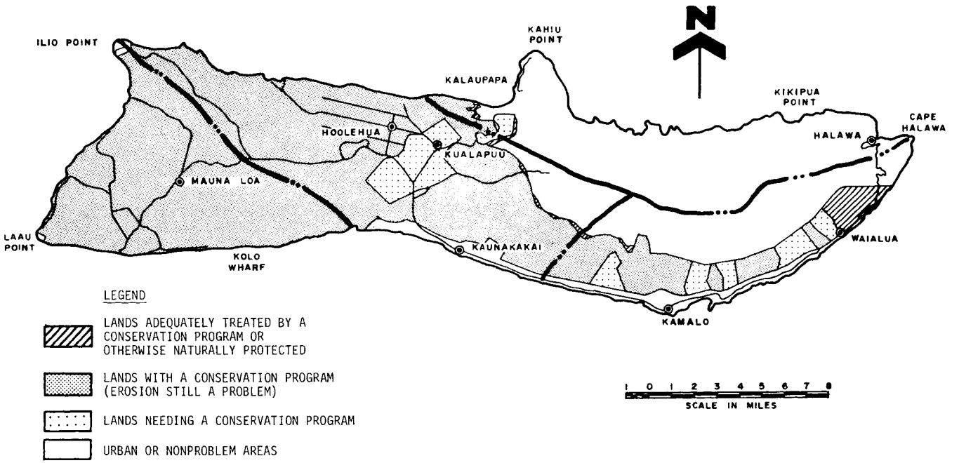
Map 15. Estimated erosion status of the island of Molokai, Hawaii. (Technical Committee on Nonpoint Source Pollution Control 1978)
