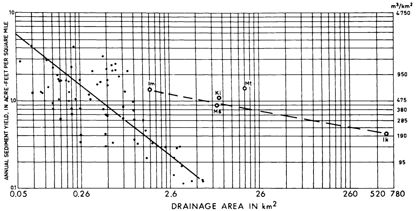
Figure 4. Relation of mean annual sediment yield to drainage area for the five catchment basins in Tanzania (open circles) compared to seventy-three semiarid basins (dots) in eastern Wyoming, U.S.A. Ik = Ikowa watershed; Im = Imagi watershed; Ki = Kisongo watershed; Ms = Msalatu watershed; Mt = Matumbulu watershed. (Rapp 1977a)
