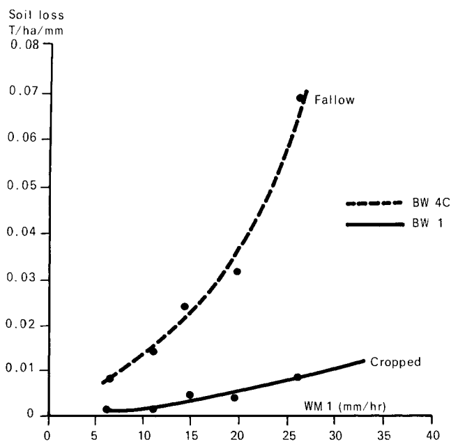
Figure 26. Comparative soil erosion from cropped and fallow Vertisols during the rainy season. (Krantz et al. 1978)
