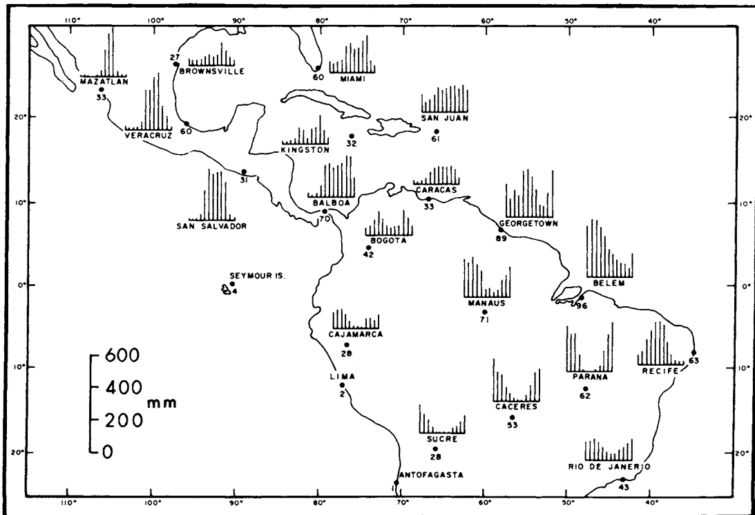
Map 21. Mean monthly rainfall for selected stations in the Americas. Numbers indicate mean annual rainfall in inches. (Atkinson 1971)
