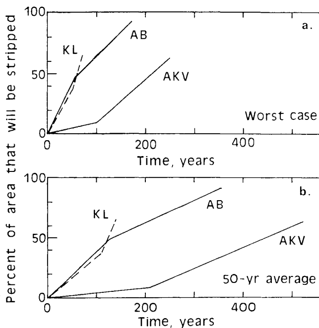
Figure 8. Extent of land that will have its soil cover removed completely within various periods of time in three study areas in Kenya: (a) assumes the "worst case" conditions of erosion rates from the past 15 years continuing into the future; (b) assumes the continuation of the average erosion rate from the past 50 years. AKV = the area of volcanic rocks on the Athi-Kapiti Plains; AB = basement schists and gneisses around Amboseli; KL = hillslopes on the Kilimanjaro lavas. (After Dunne et al. 1978b)
