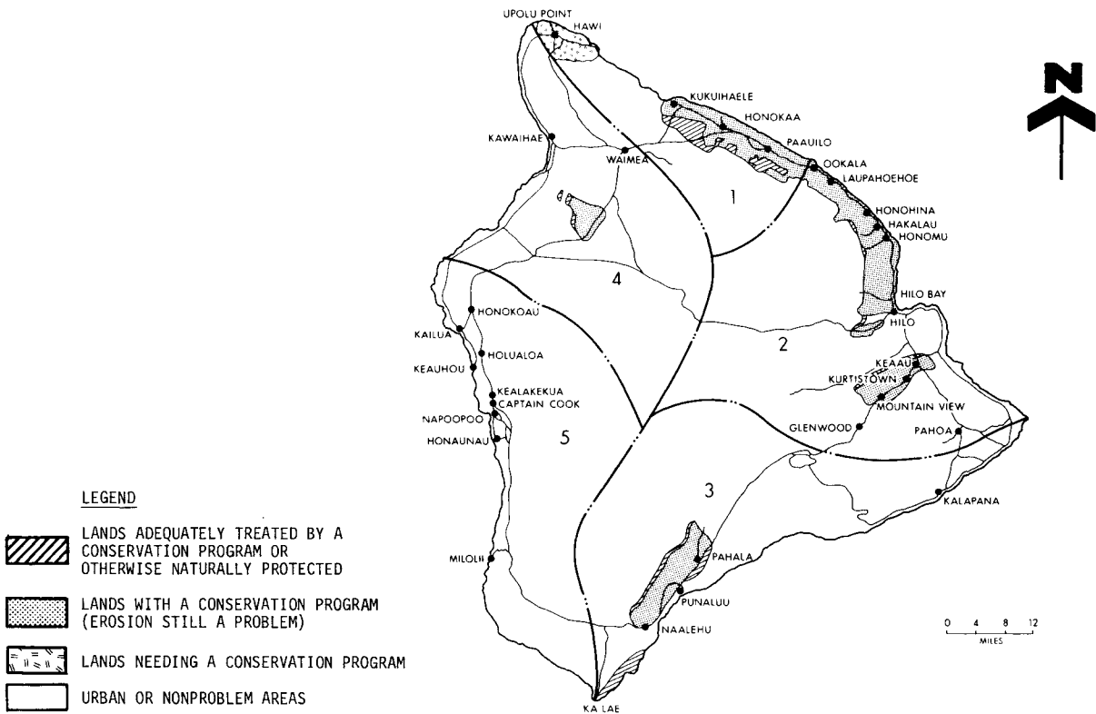
Map 18. Estimated erosion status of the island of Hawaii. (Technical Committee on Nonpoint Source Pollution Control 1978)
