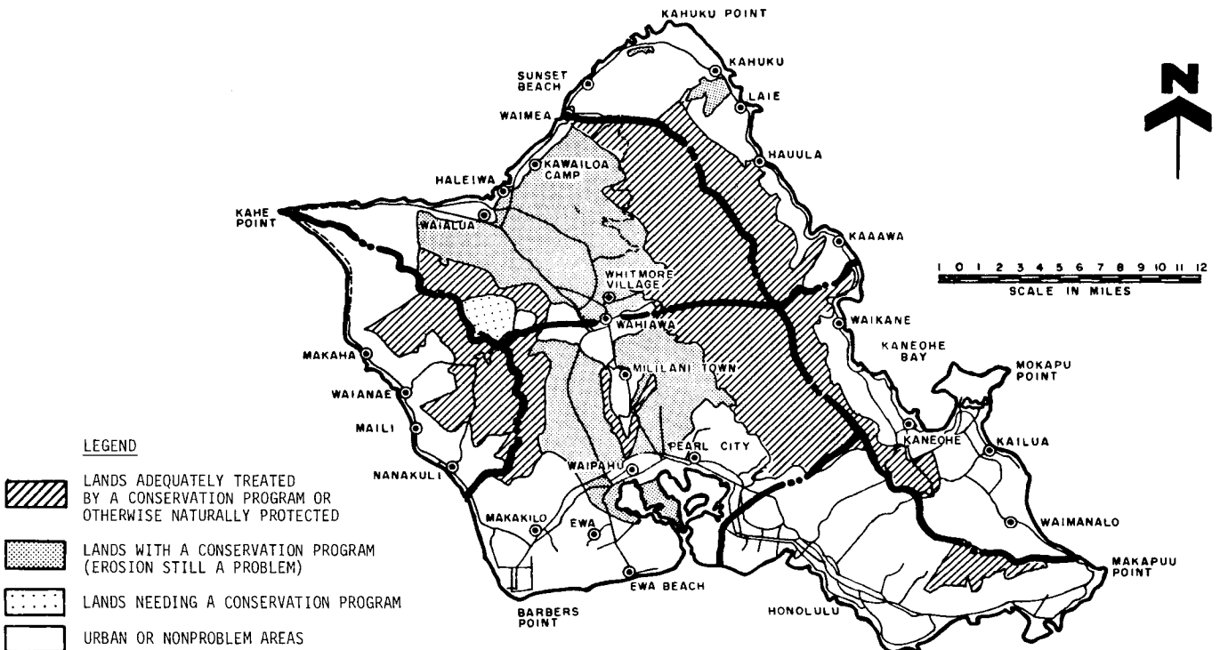
Map 14. Estimated erosion status of the island of Oahu, Hawaii. (Technical Committee on Nonpoint Source Pollution Control 1978)
