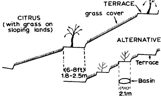
Figure 34. Major types of terraces. (Sheng 1977a)
