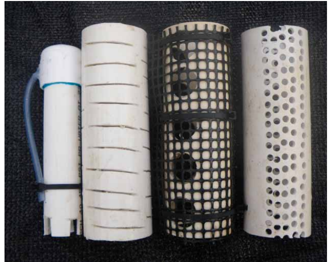
15. Different styles of gravel guard.
