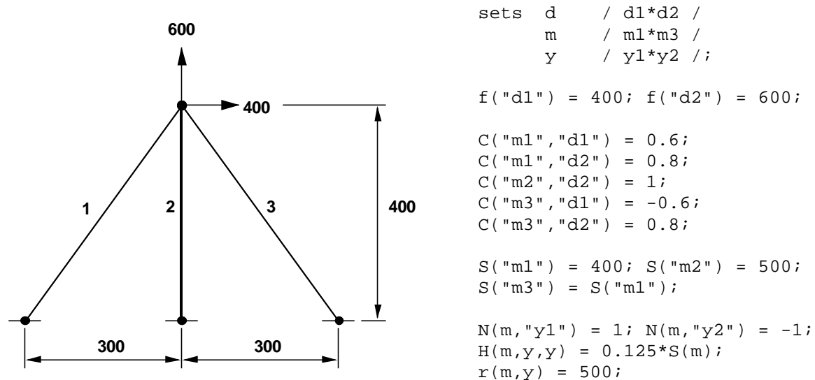
Figure 2: Three-bar truss and associated state.dat input
