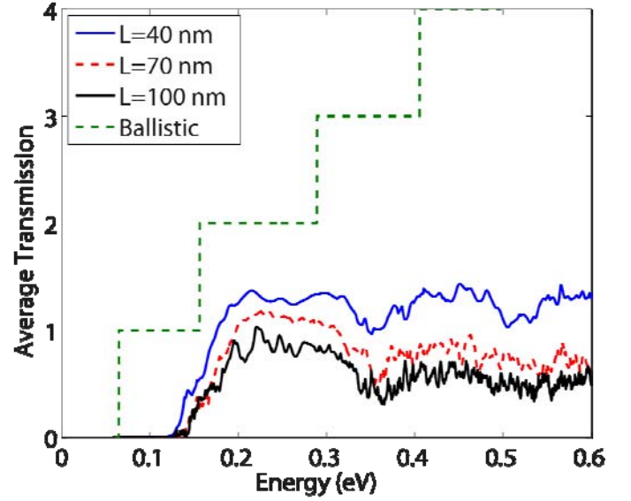
Figure 6: Transmission of 8 nm wide rippled graphene nanoribbons of various lengths. For reference, the transmission of a perfectly flat 8 nm nanoribbon is included (“ballistic”).
