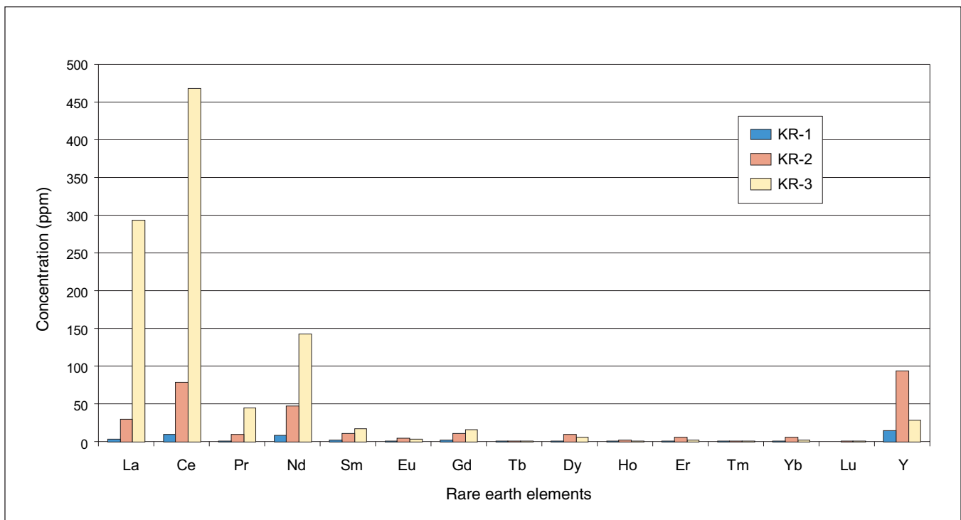
Figure 1 Rare earth element concentrations.
