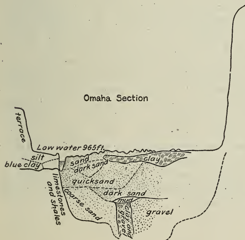
FIG. 4. Diagram to show the heterogeneous character of alluvial deposits. [After Todd. Republished by the courtesy of the U. S. Geological Survey.]
