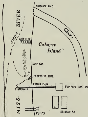
FIG. 5. Cabaret Island and Granite City pumping station of the city water company
