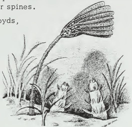
Ordovician Crinoid
