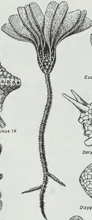
Glyptocrinus 1X
