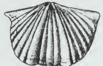
Platystrophia 2/3 X
