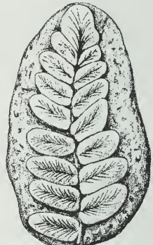
Neuropteris 1/2X
