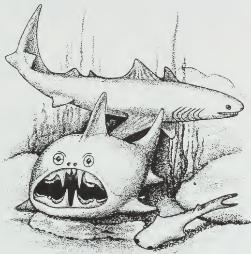
Devonian Fish
