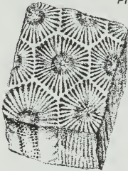
Hexagonaria 1 X
