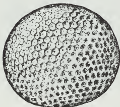
Sphaerospongia 2/3 X
