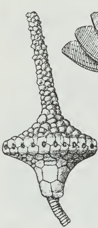
Eutrochocrinus 1X
