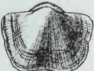
Hebertella 1/2 X
