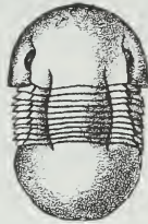
Illaenus 1X
