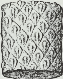
Lepidodendron 2/5X
