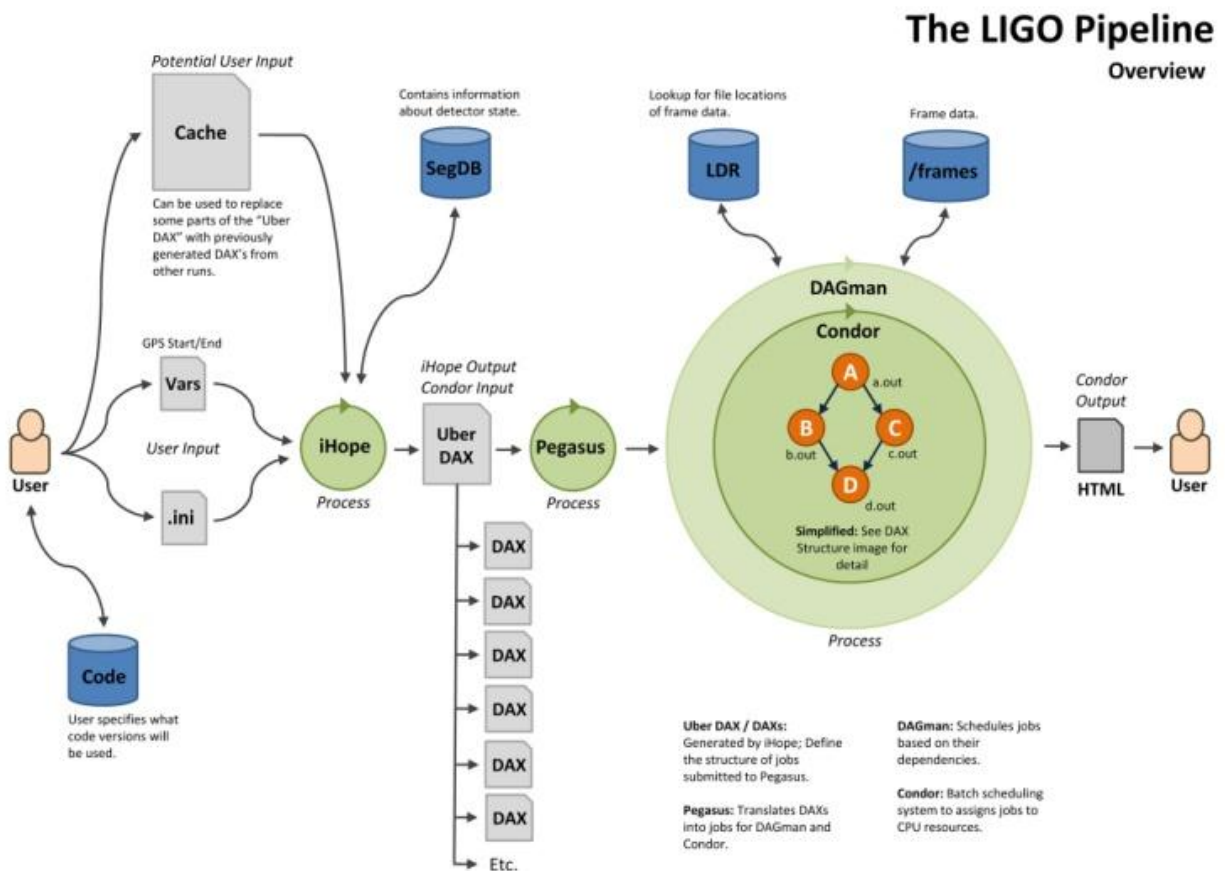
Figure 4. The final LIGO pipeline overview visualization.
