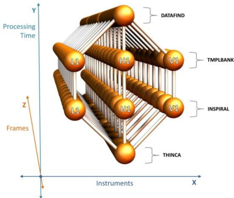
Figure 7. The pipeline in three dimensions: frame, instrument, and processing time.
