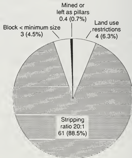
Figure 36 Factors restricting the availability of surface minable coal in the Middletown Quadrangle (millions of tons and percentage of original resources that are surface minable).
