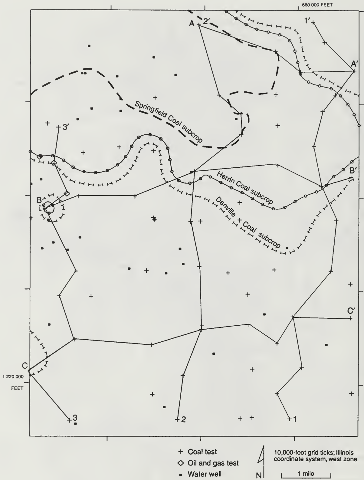
Figure 10 Distribution of data points and cross section lines used in this study.
