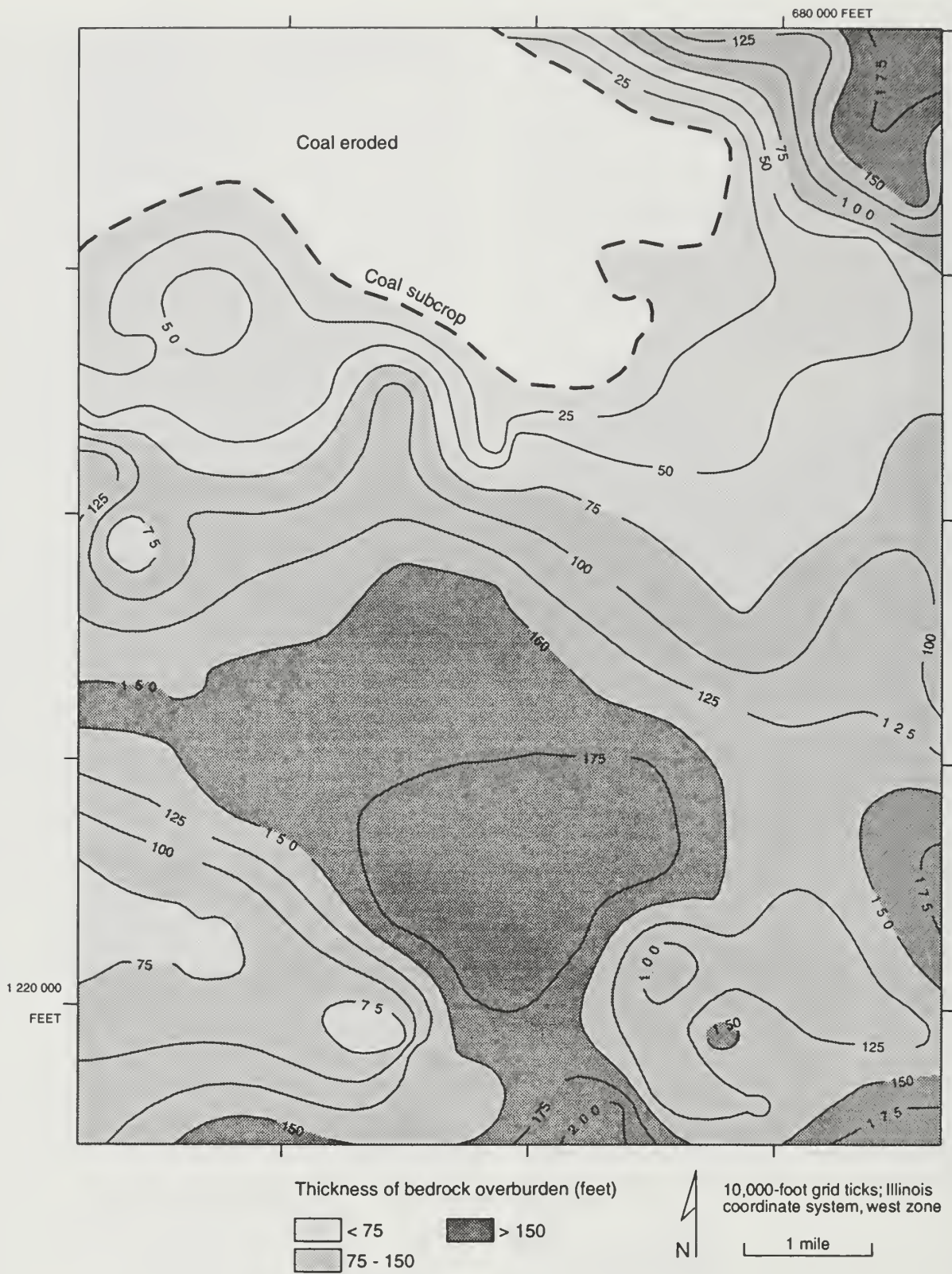
Figure 34 Thickness of bedrock cover over the Springfield Coal in the Middletown Quadrangle. Contour interval is 25 feet.
