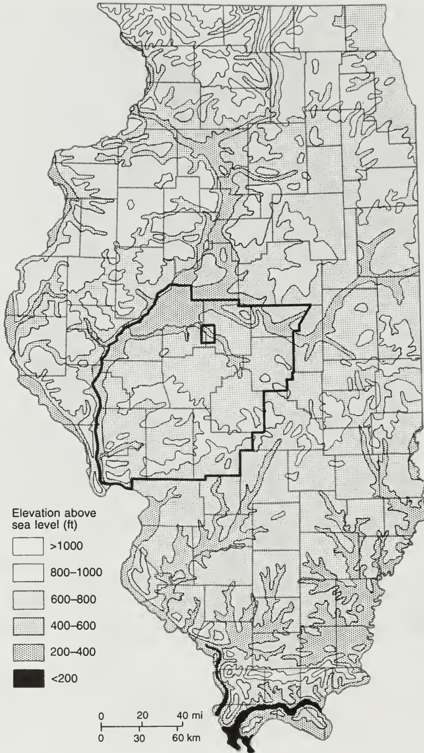
Figure 6 Topography of the bedrock surface in Illinois (from Willman and Frye 1970). Region 3 and the Middletown Quadrangle are outlined.
