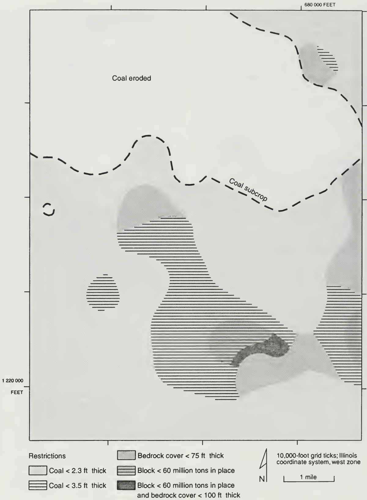
Figure 39 Availability of Herrin Coal resources for deep mining.
