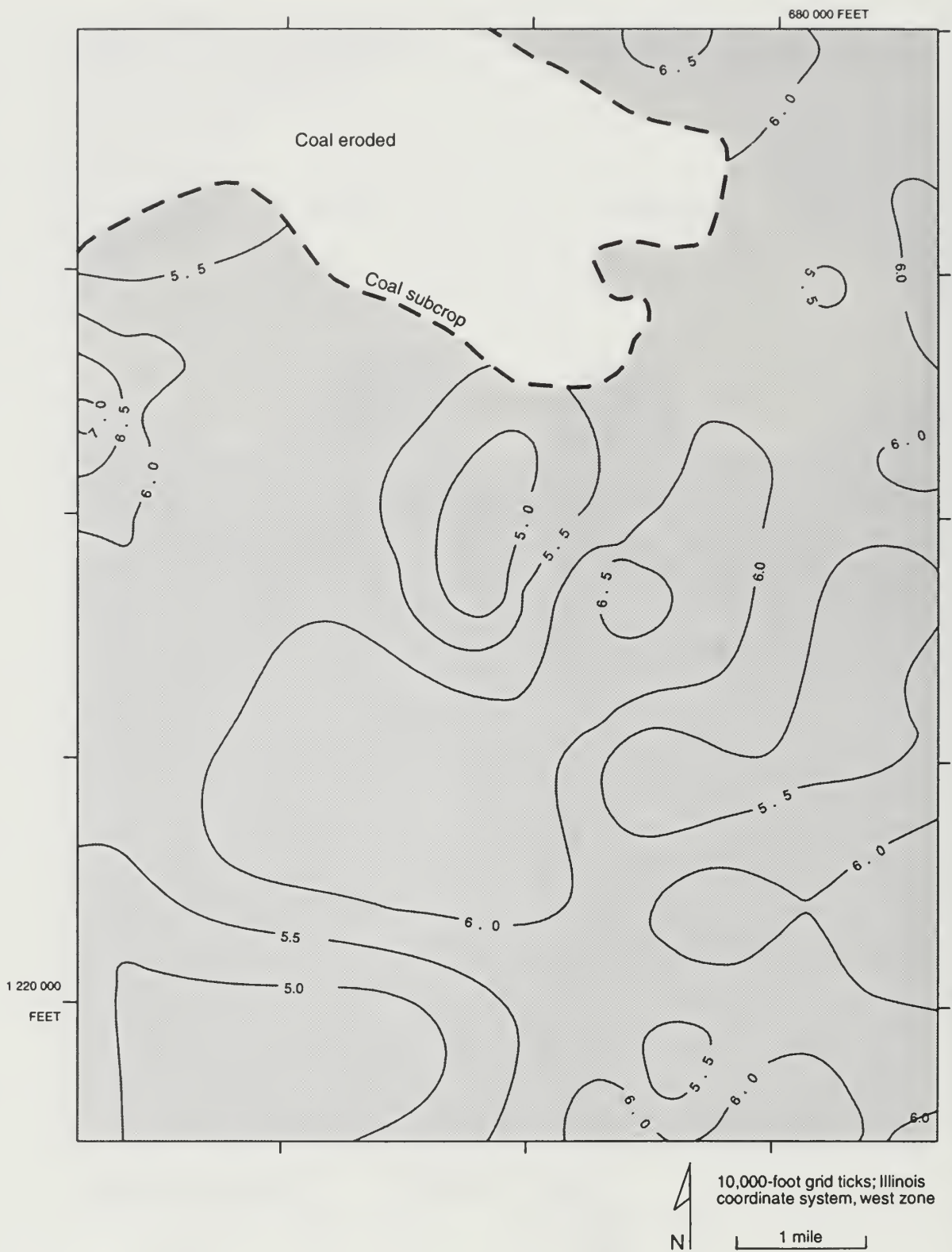
Figure 27 Thickness of the Springfield Coal in the Middletown Quadrangle. Contour interval is 0.5 feet.
