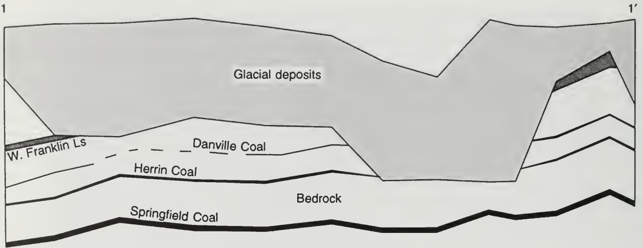
Figure 14 Cross section 1-1'. See figure 10 for location.
