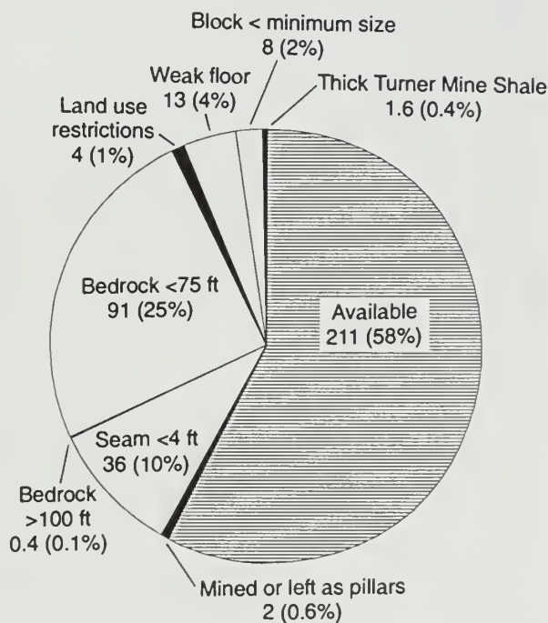
Figure 37 Factors restricting the availability of deep minable coal in the Middletown Quadrangle (millions of tons and percentage of original resources that are deep minable).
