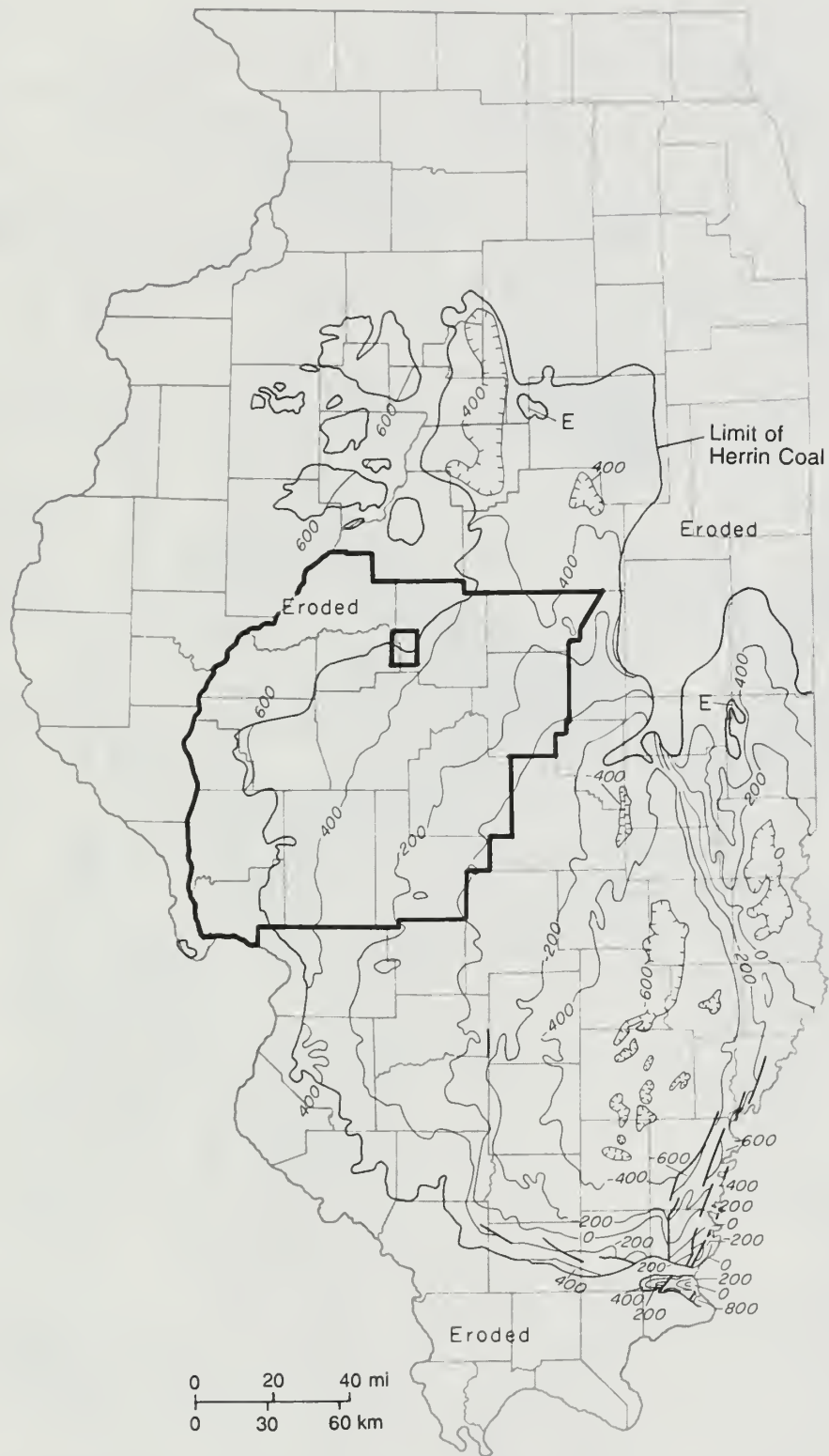
Figure 7 Elevation of the top of the Herrin Coal (from Willman et al. 1975). Contour interval is 200 feet. Region 3 and the Middletown Quadrangle are outlined.
