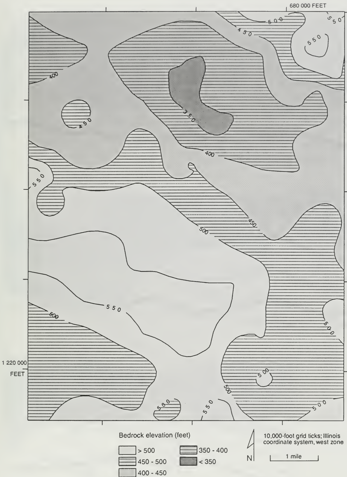
Figure 13 Elevation of the bedrock surface in the Middletown Quadrangle. Contour interval is 50 feet.
