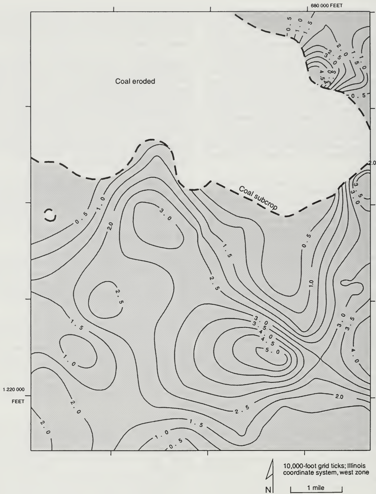
Figure 25 Thickness of the Herrin Coal in the Middletown Quadrangle. Contour interval is 0.5 feet.
