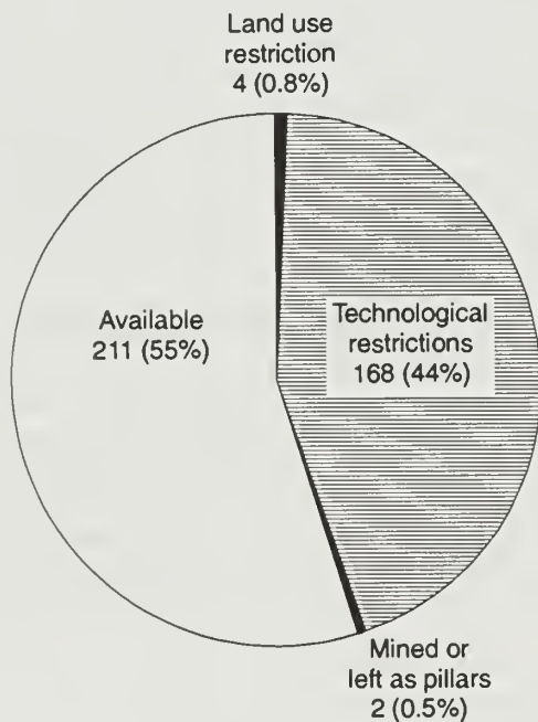
Figure 35 Availability of coal resources in the Middletown Quadrangle (millions of tons and percentage of original resources).
