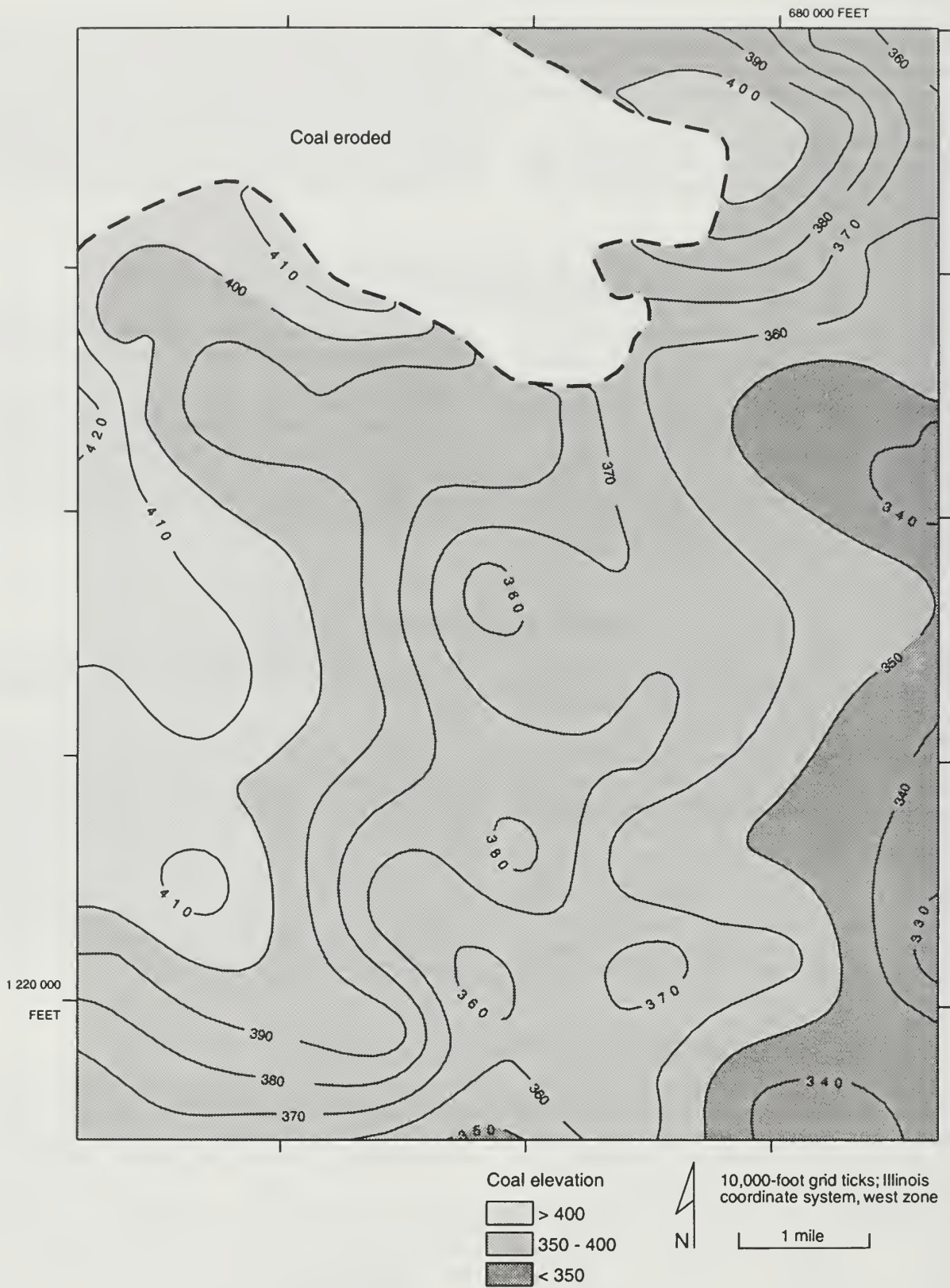
Figure 31 Elevation of the top of the Springfield Coal in the Middletown Quadrangle. Contour interval is 10 feet.
