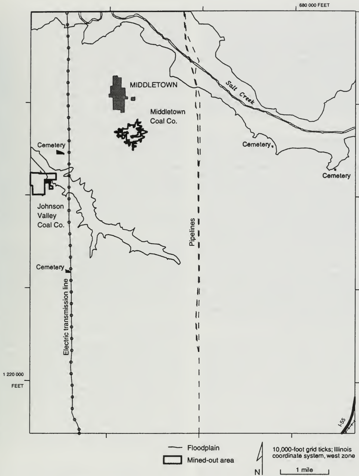
Figure 32 Selected features of the Middletown Quadrangle.
