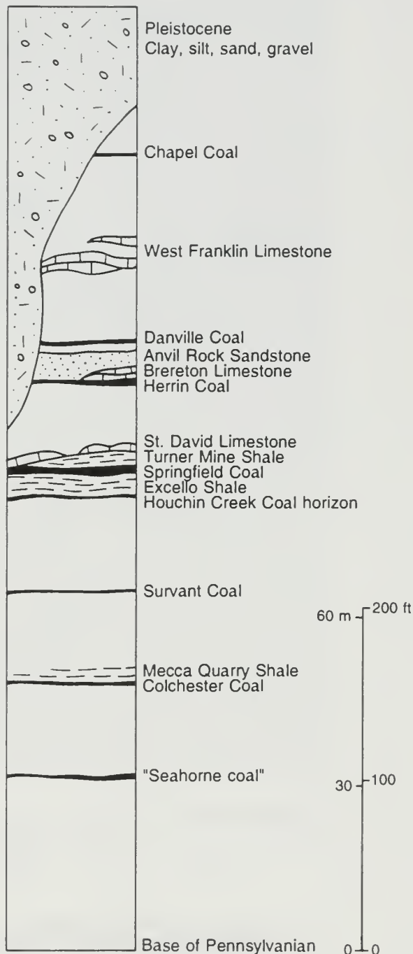
Figure 11 Selected stratigraphic units present in the Middletown Quadrangle. Vertical scale: 1 inch equals approximately 70 feet.
