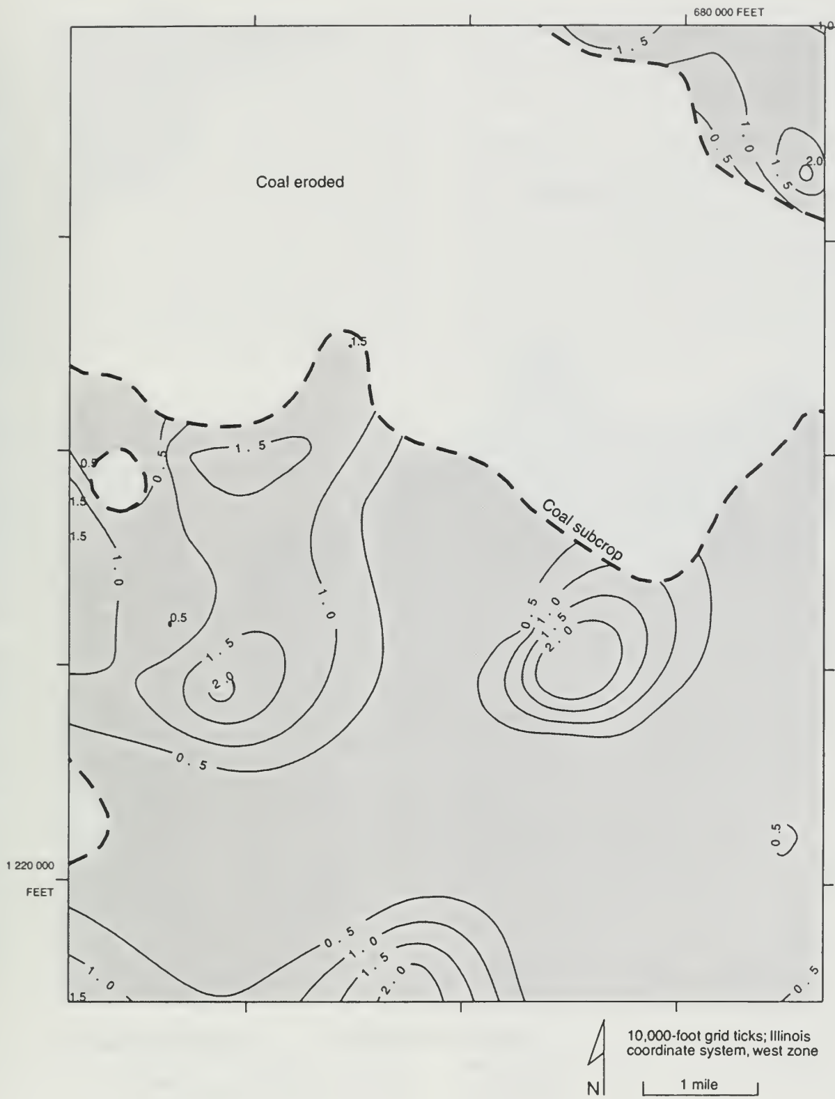
Figure 23 Thickness of the Danville Coal in the Middletown Quadrangle. Contour interval is 0.5 feet.
