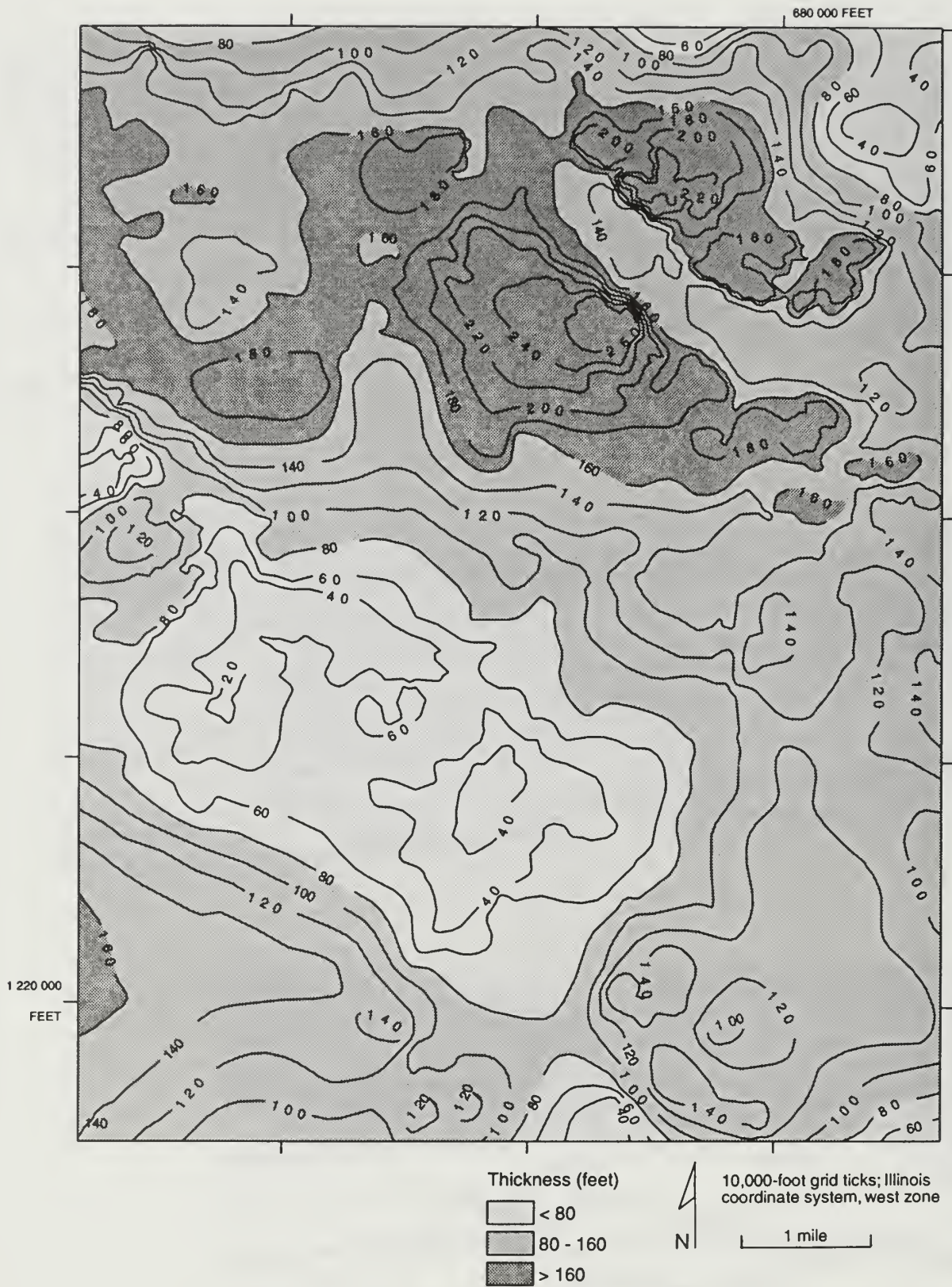
Figure 20 Thickness of glacial sediments in the Middletown Quadrangle. Contour interval is 20 feet.
