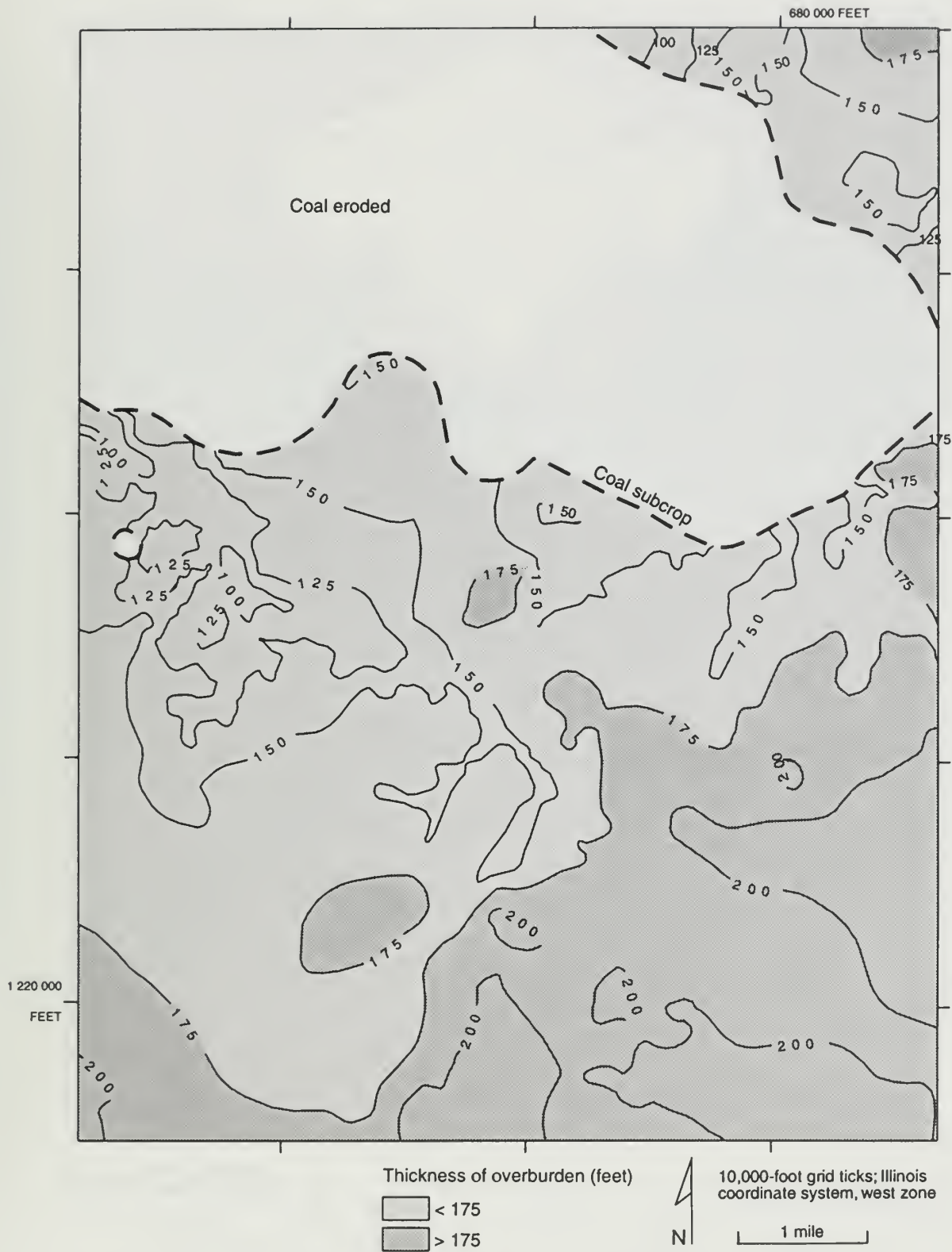
Figure 26 Thickness of overburden of the Herrin Coal in the Middletown Quadrangle. Contour interval is 25 feet.
