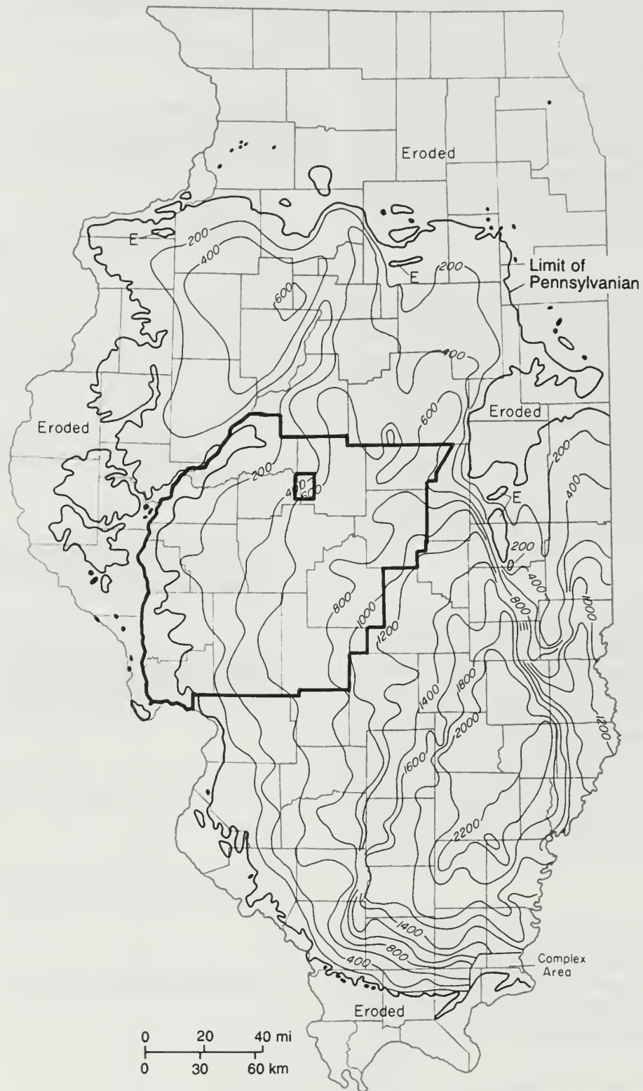
Figure 12 Thickness of Pennsylvanian System in Illinois (from Willman et al. 1975). Contour interval is 200 feet. Region 3 and the Middletown Quadrangle are outlined.
