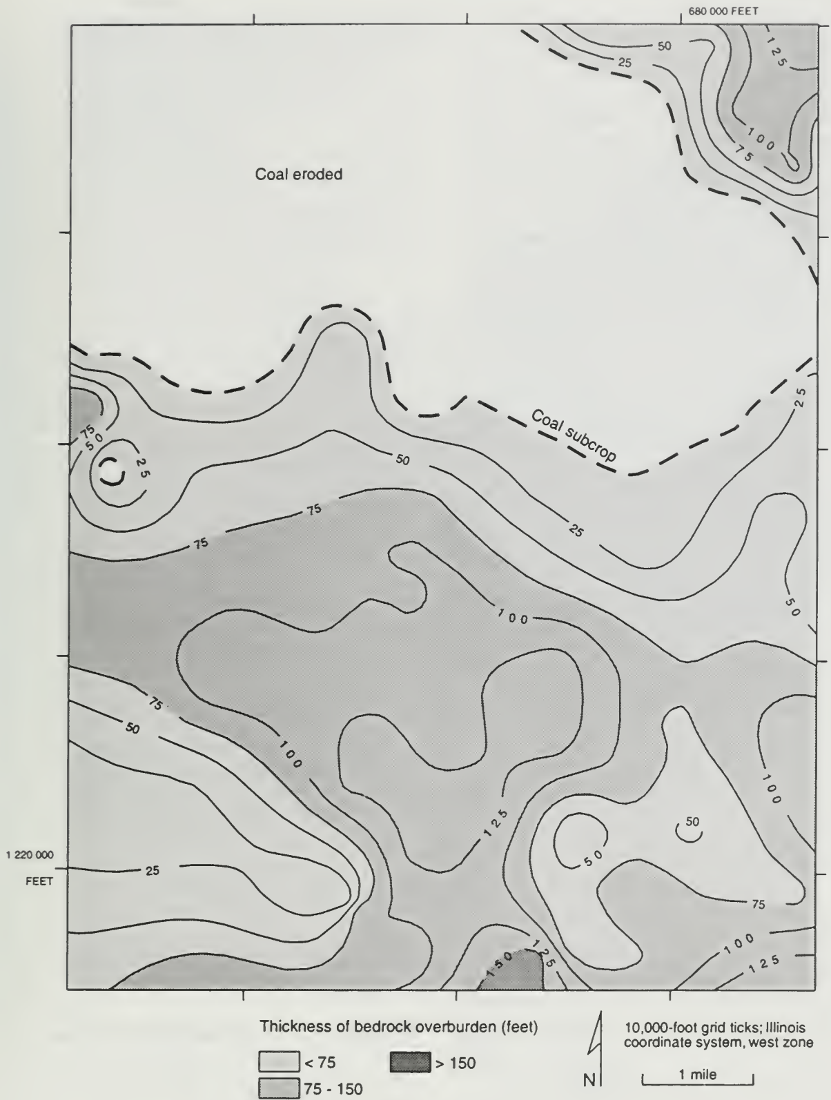
Figure 33 Thickness of bedrock cover over the Herrin Coal in the Middletown Quadrangle. Contour interval is 25 feet.
