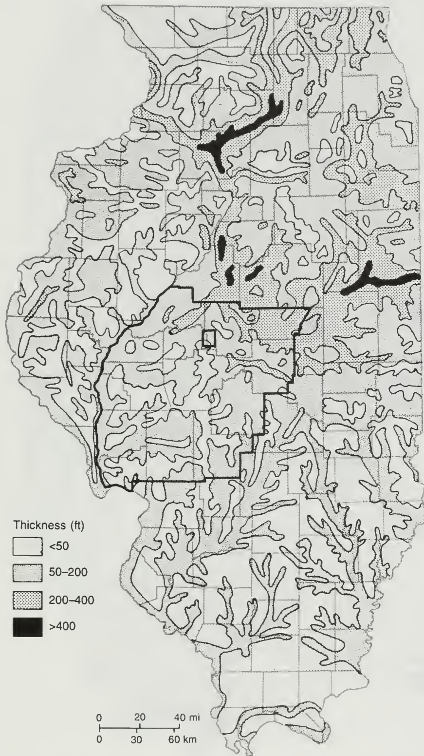
Figure 5 Thickness of Pleistocene deposits in Illinois (from Willman and Frye 1970). Region 3 and the Middletown Quadrangle are outlined.
