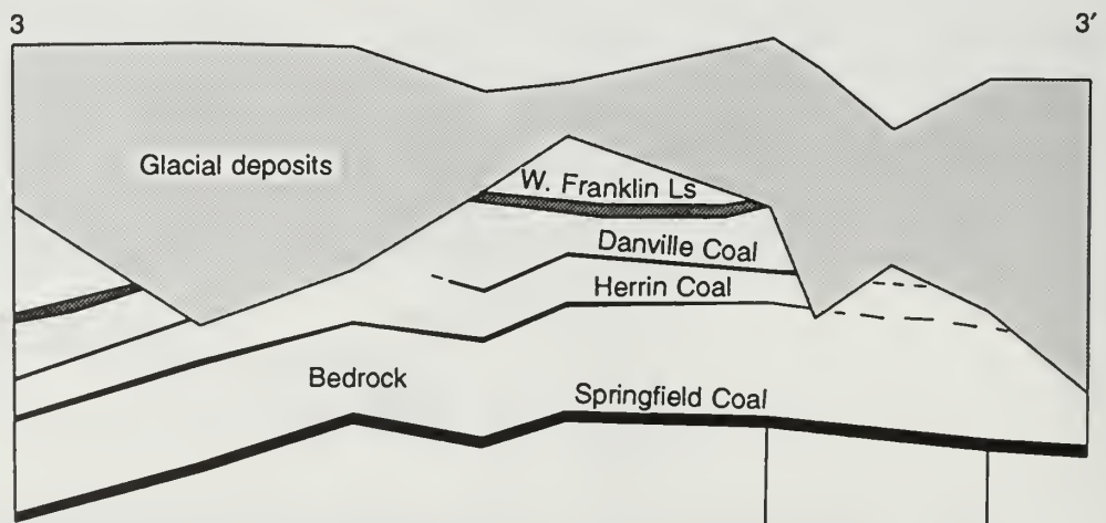
Figure 16 Cross section 3-3'.
