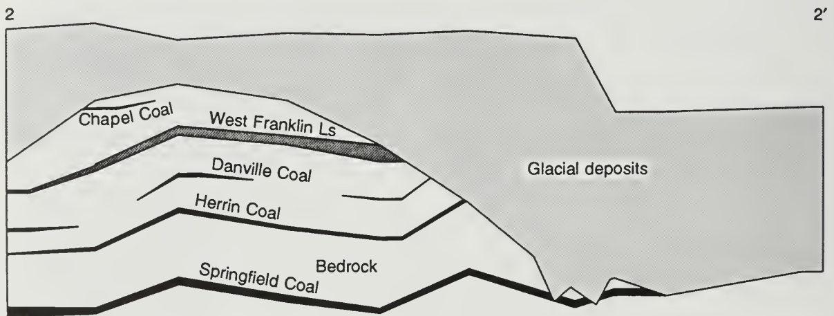
Figure 15 Cross section 2-2'.
