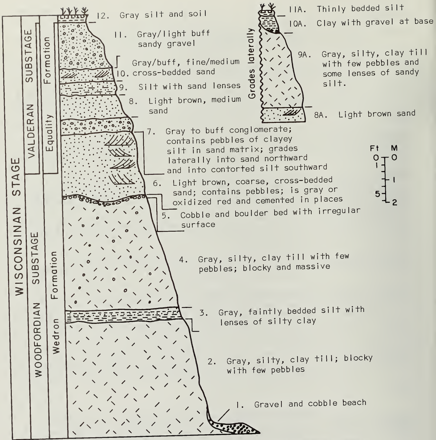
Fig. 6 - Stratigraphic section just south of Lake Bluff sewage disposal plant. SE \frac{1}{4} NE \frac{1}{4} , Sec. 21, T. 44 N., R. 12 E., Lake County, Waukegan Quadrangle.
