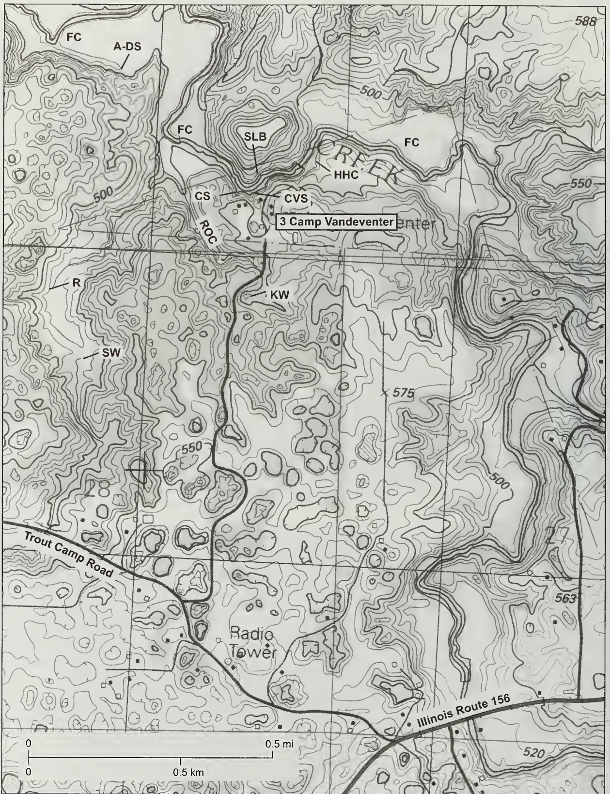
Figure 27 Topographic Map of Camp Vandeventer area (Stop 3) showing various karst features. Abbreviations: FC, Fountain Creek; A-DS, Annabriar-Dual Spring; SLB, St. Louis bluff; HHC, Hidden Hand Cave; CVS, Camp Vandeventer Spring; CS, unnamed cave spring; ROC = resurgence overflow channel; R = resurgence; SW = swallow hole; KW = karst window. The sinking and rising sites on Fountain Creek are not shown.
