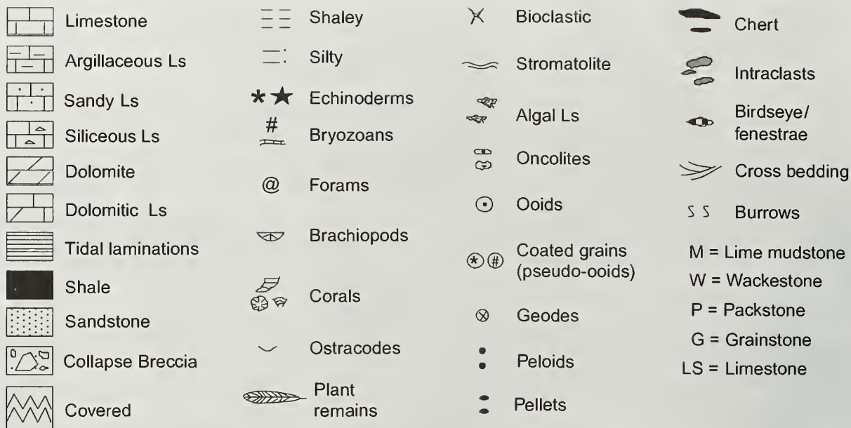
Figure 20 Key to figures 19, 32, and 37.
