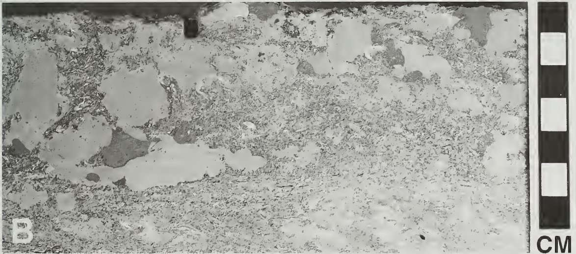
Figure 2 A. Lower and upper Warsaw Formation, Beltrees Road section, NE NE SW Sec. 13, T6N, R11W, Jersey County, Illinois, Elsah 7.5-minute Quadrangle. B. The intraclastic, pyritic, and phosphatic horizon that marks the lower-upper Warsaw boundary (dashed line in A).
