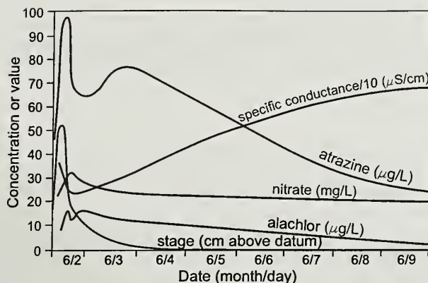
Figure 16 Graph showing discharge and other parameters from Kelly Spring, Monroe County, Illinois, during a 2.7-centimeter (1.05-inch) rainfall event in the spring of 1994. Stage level indicates discharge rate from the spring, showing a characteristic storm pulse. Specific conductance of the water decreased rapidly because of the dilution of the sudden recharge of rainwater. Agricultural concentrations increased rapidly to peak values just after the discharge peaked, probably because they were briefly attenuated by the soil immediately after application. Modified after Panno et al. (1995).
