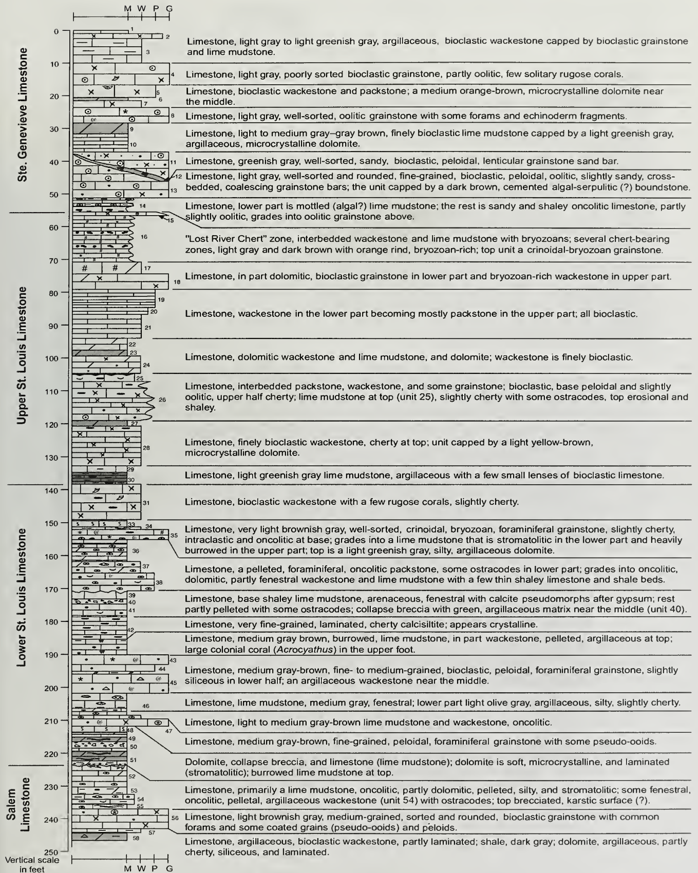
Figure 19 Stratigraphic column of Casper Stolle Quarry. Key for symbols on figure 20.
