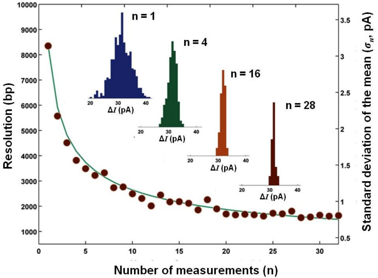
Figure 6. The effect of averaging over multiple measurements on the resolution and standard deviation of the averaged translocation signals. Symbols denote experimental data while the solid line denotes a 1/n fit. Histograms of the translocation signal amplitude ( \Delta I ) corresponding to n=1 and averaging over n=4, 16, and 28 are shown in the inset.
