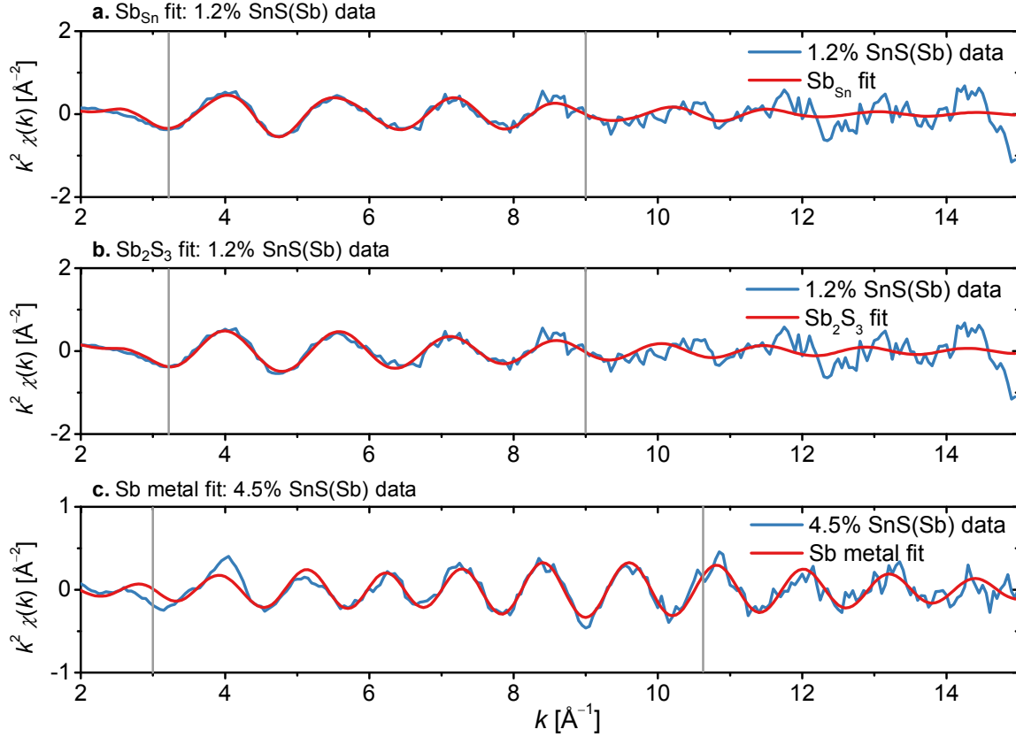
Figure 6. EXAFS data and fits for Sb edge: (a) 1.2% SnS(Sb) data with SnS(Sb Sn ) fit, (b) 1.2% SnS(Sb) data with Sb 2 S 3 fit, and (c) 4.5% SnS(Sb) data with Sb metal fit. The vertical lines denote the range chosen for Fourier transformation.
