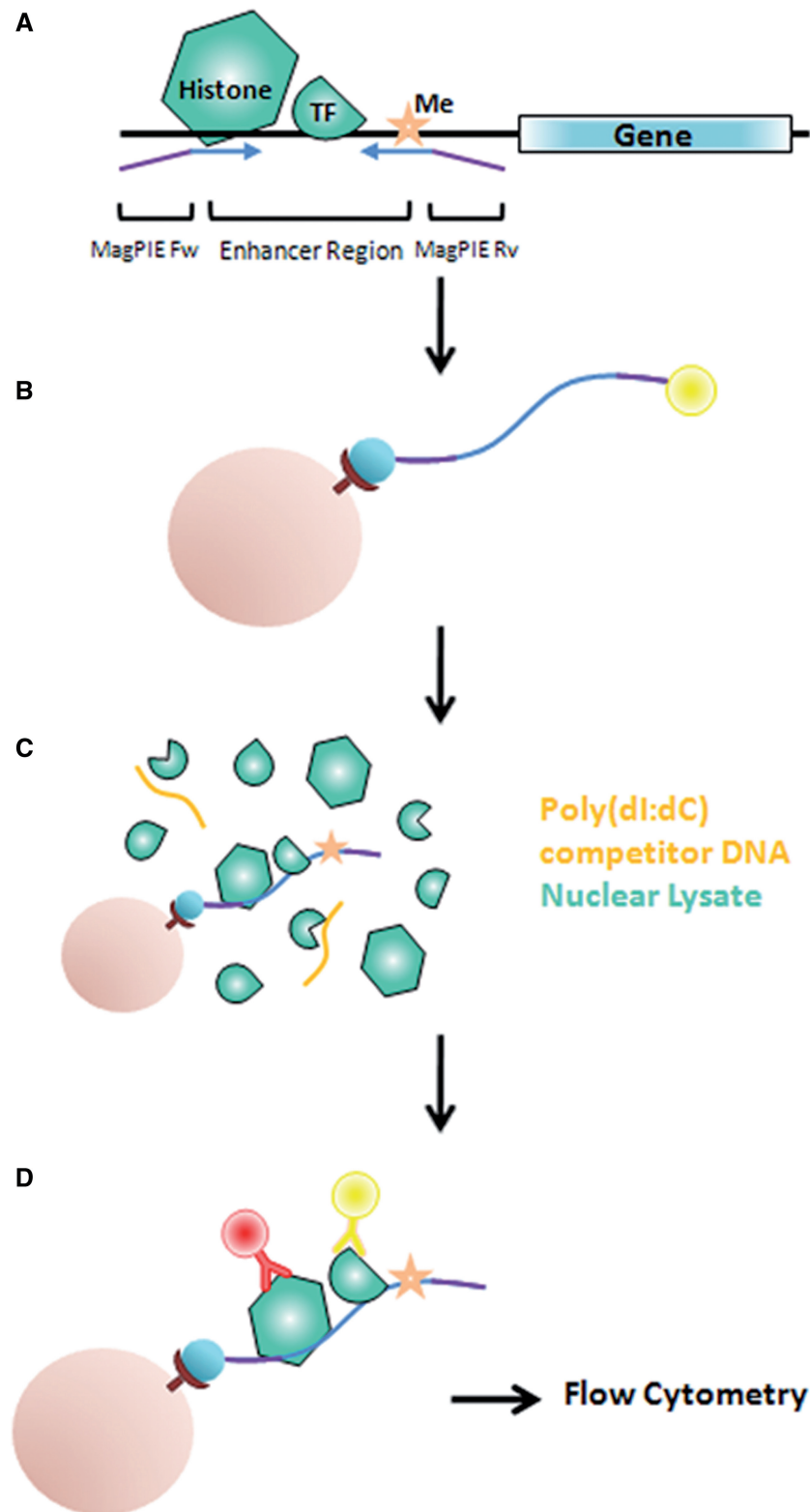
Figure 1. MagPIE experimental flowchart. (A) Genomic regions are amplified by PCR using sequence-specific primers linked to MagPIE primer sequences predicted to have low TF-binding affinity. The DNA is further amplified using a biotinylated MagPIE reverse primer and a MagPIE forward primer that may be tagged with a fluorophore. (B) Biotinylated DNA is captured on SA-coated magnetic beads. (C) Bead-immobilized DNA is incubated with crude nuclear protein lysate in the presence of competitor poly(dI:dC) DNA to pull down sequence-specific nuclear factors in a 10-min binding reaction at 37°C. (D) TFs and other DNA-bound proteins are immunostained with fluorescently tagged antibodies, and fluorescence intensity is analyzed by flow cytometry.
