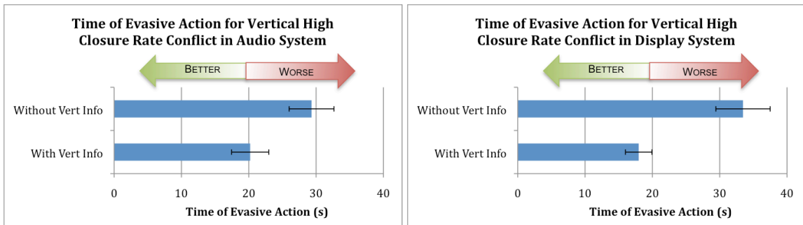
Figure 4-15. Time of Evasive Action for the Vertical High Closure Rate Conflict for the Audio (left) and Display (right) Systems.
