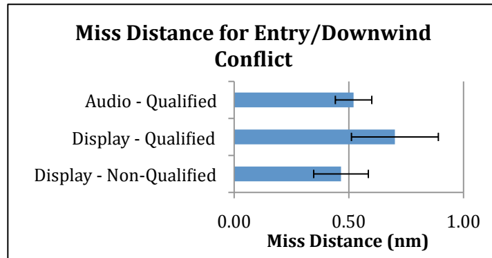
Figure 5-14. Miss Distance for the Entry vs. Downwind Encounter
