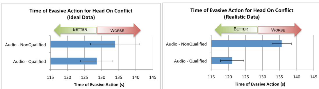
Figure 5-19. Time of Evasive Action for Head-On Conflict – Qualified Comparison (Left- Ideal Data Quality, Right- Realistic Data Quality)
