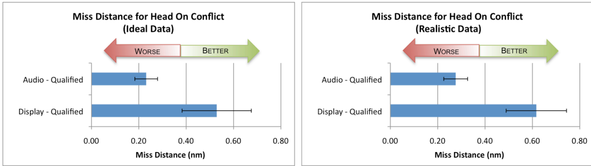
Figure 5-20. Miss Distance for Head-On Conflict (Left- Ideal Data Quality, Right- Realistic Data Quality)
