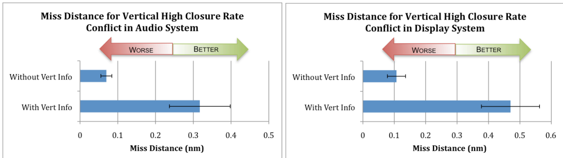
Figure 4-14. Miss Distance for the Vertical High Closure Rate Conflict for the Audio (left) and Display (right) Systems.
