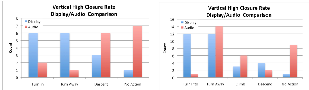
Figure 5-25. Type of Evasive Action for the Vertical High Closure Rate Conflict (Left- Ideal Data Quality, Right- Realistic Data Quality)
