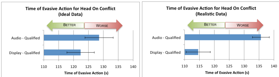
Figure 5-18. Time of Evasive Action for Head-On Conflict (Left- Ideal Data Quality, Right- Realistic Data Quality)
