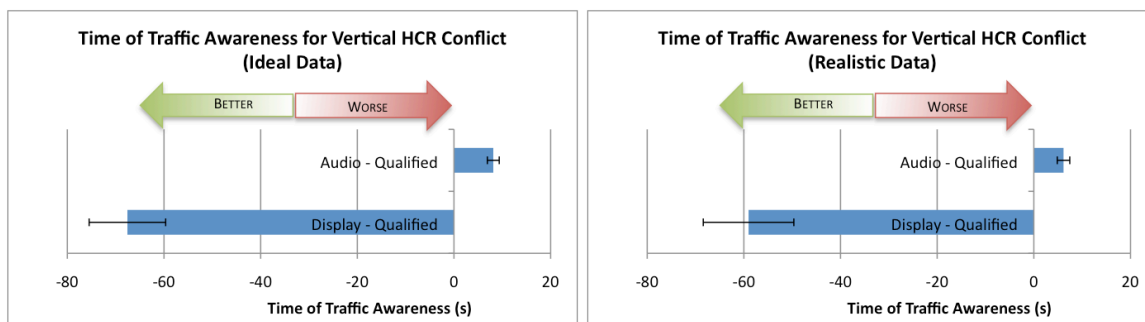
Figure 5-24. Time of Traffic Awareness for Vertical HCR Conflict with Respect to the Time that the Target Began Descending (Left- Ideal Data Quality, Right- Realistic Data Quality)
