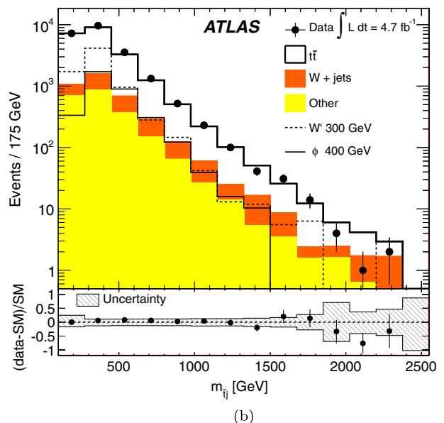
FIG. 4 (color online). Expected and observed distributions of (a) m_{ij} and (b) m_{\bar{i}\bar{j}} in the signal region. The example signal distributions assume unit coupling for the new physics process. The total uncertainty shown on the ratio includes both statistical and systematic effects. The other background category includes single top production, diboson production, and multijet events.
