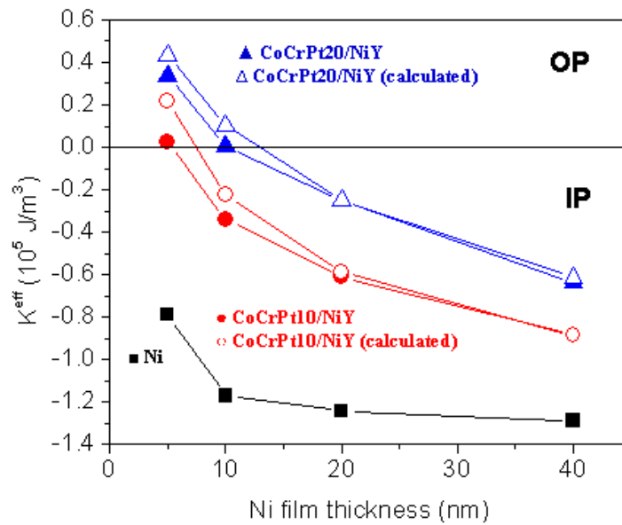
Figure 2. Experimental values from equation (2) for the effective anisotropy energy of Ni (■), t_{\text{CoCrPt}} = 10 nm (●) and t_{\text{CoCrPt}} = 20 nm (▲) composites and predicted values from equation (4) for t_{\text{CoCrPt}} = 10 nm (○) and t_{\text{CoCrPt}} = 20 nm (△) composites as a function of the Ni film thicknesses.
