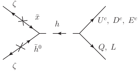
Figure 12. The pseudo-goldstino can annihilate through its higgsino component to SM quarks and leptons. However, this cross section is very small, and the pseudo-goldstino is a cosmologically dangerous hot relic.
