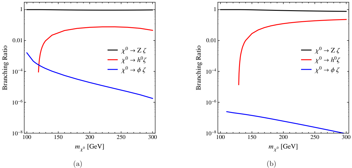
Figure 10. Left: branching ratios for a neutralino LOSP as a function of its mass m_{\chi^0} in the R -violating case. We fix \tilde{m}_{h_u}^2 = \tilde{m}_{h_d}^2 = \tilde{m}_{r_u}^2 = \tilde{m}_{r_d}^2 = (140 \text{ GeV})^2 , \mu_u = 500 \text{ GeV} , B_u = B_d = (70 \text{ GeV})^2 , M_1 = M_2 = 400 \text{ GeV} , \lambda = 1 , \kappa is fixed by m_Z , and all other soft parameters are set to zero. We have traded \mu_d for m_\chi . Right: branching ratios for a neutralino LOSP in the R -symmetric case. We use the same parameters as in the left figure, except we set the Majorana gaugino masses and B -terms equal to zero, and we set the Dirac mass for gauginos m_D = 1 \text{ TeV} . The dominant decay mode for the neutralino LOSP is \chi^0 \rightarrow Z\zeta over much of parameter space.
