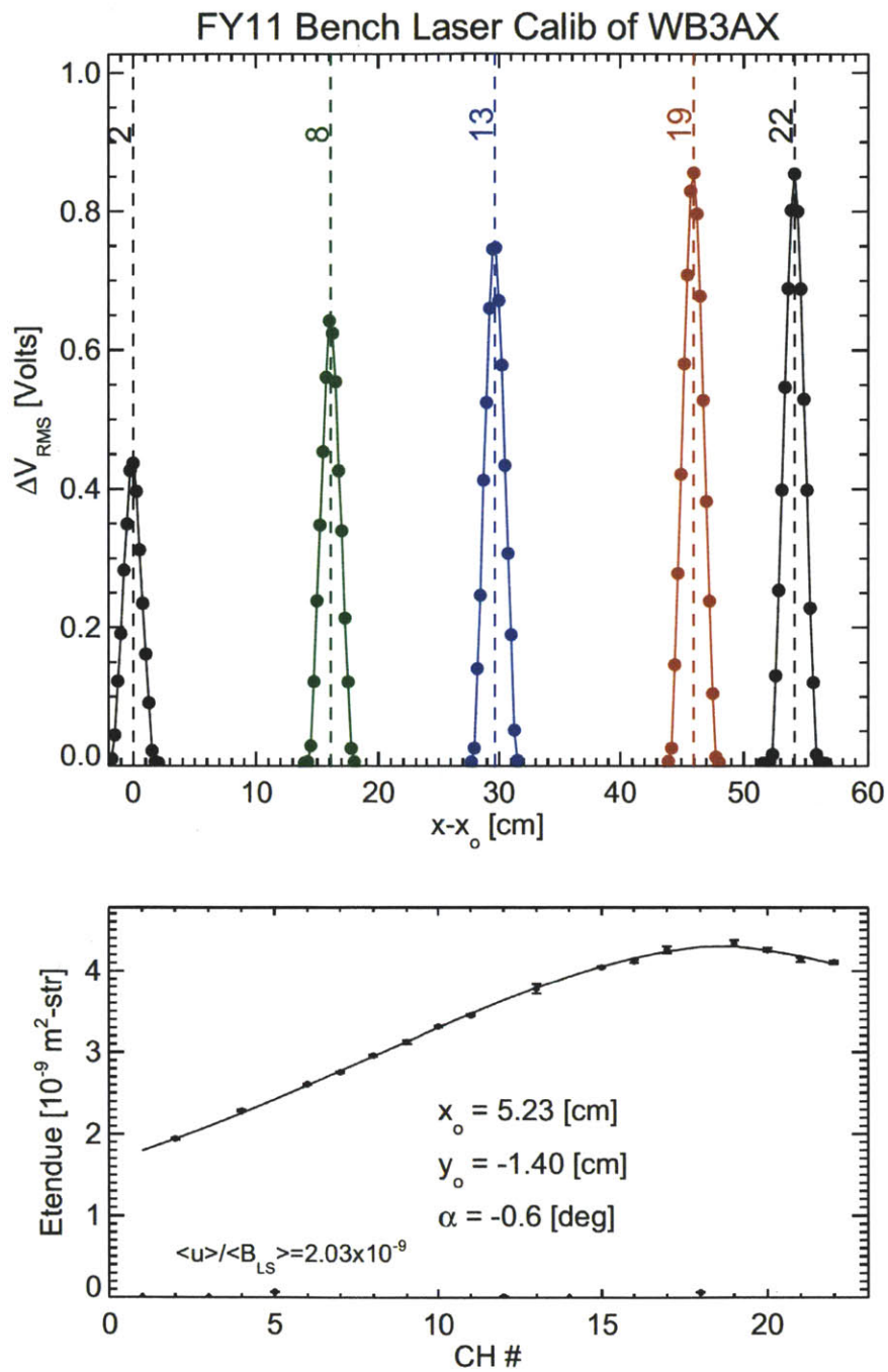
Figure B-18: Results of the WB3AX benchtop laser (top) and Labsphere calibrations (bottom) used to find x_0 , y_0 and \alpha
