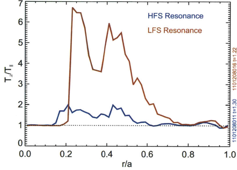
Figure 5-4: The TRANSP-predicted temperature anisotropy of the minority ions for HFS and LFS ICRH heating
