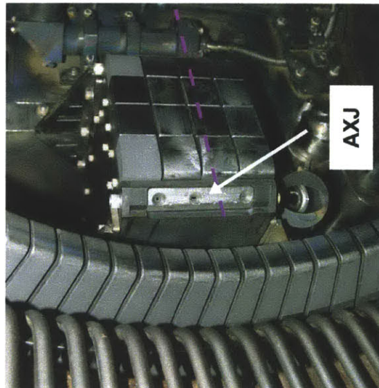
Figure 3-3: Views of the KLIM enclosure inside Alcator C-Mod
