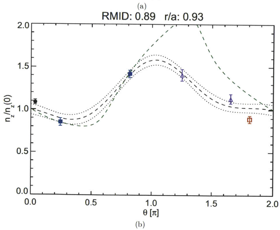
Figure 6-9: Poloidal variation in the impurity density for an EDA H-mode with strong molybdenum radiation; AXA ( \bullet ), AXJ ( \circ ), WB2AX ( \blacksquare ), WB3AX ( \square ) and WB4AX ( \triangle )
