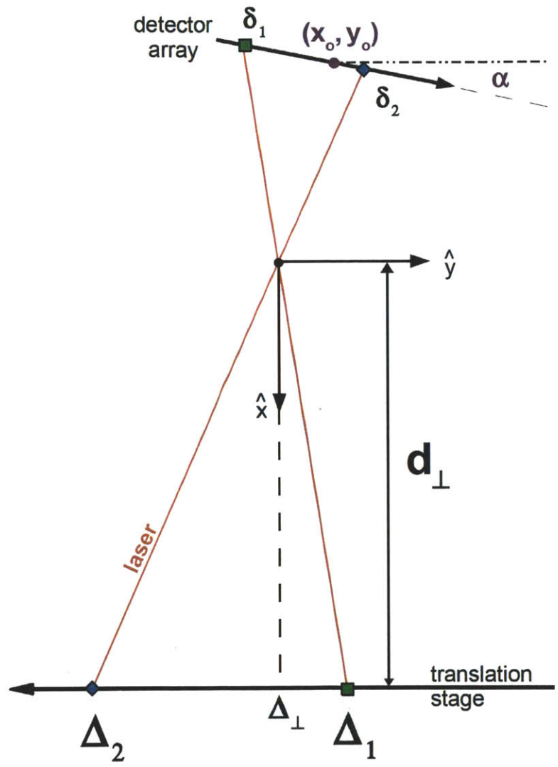
Figure B-1: Sketch showing how the variables measured in the benchtop laser calibration ( \delta_i , \Delta_i and d_{\perp} ) can be used to find x_o , y_o and \alpha of the array
