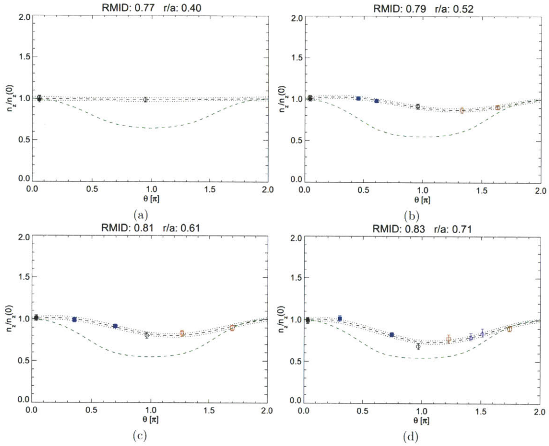
Figure 4-33: Measured poloidal variation of emissivity (symbols) compared to modeling (dashed green) showing significant disagreement for an L-mode plasma; AXA ( \bullet ), AXJ ( \circ ), WB2AX ( \blacksquare ), WB3AX ( \square ) and WB4AX ( \triangle )
