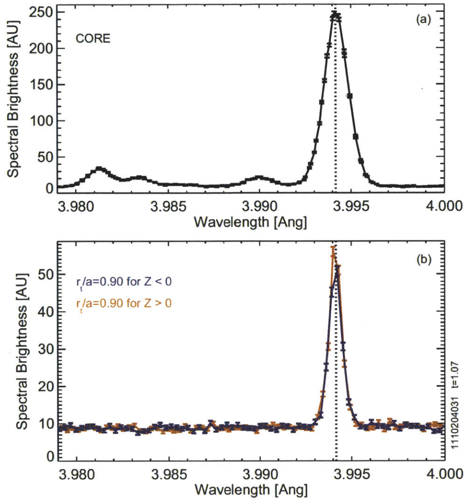
Figure D-7: Spectra for the core and chords at r/a = 0.9 for the up/down symmetric case shown in Figure D-6
