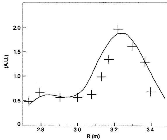
FIG. 4. Ni density derived from the soft x-ray emissivity at t=6.72 s (cross) and calculated Ni density at the same time (line).
