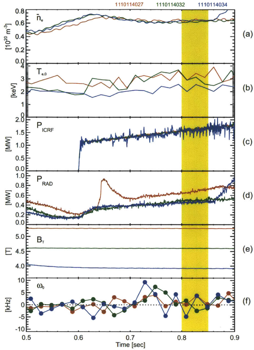
Figure 5-20: Time evolution of relevant plasma parameters for a resonance layer scan with J-ANT at 70 MHz
