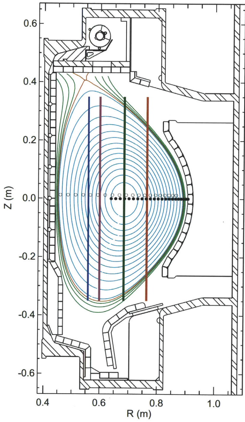
Figure 5-1: EFIT reconstruction of 78-80.5 MHz experiments showing the shot-to-shot scans of the resonance layer and including the AXA ( \bullet ), AXJ ( \circ ) tangency radii
