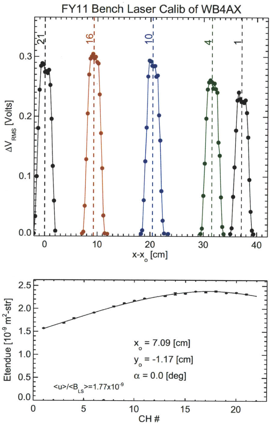
Figure B-19: Results of the WB4AX benchtop laser (top) and Labsphere calibrations (bottom) used to find x_0 , y_0 and \alpha
