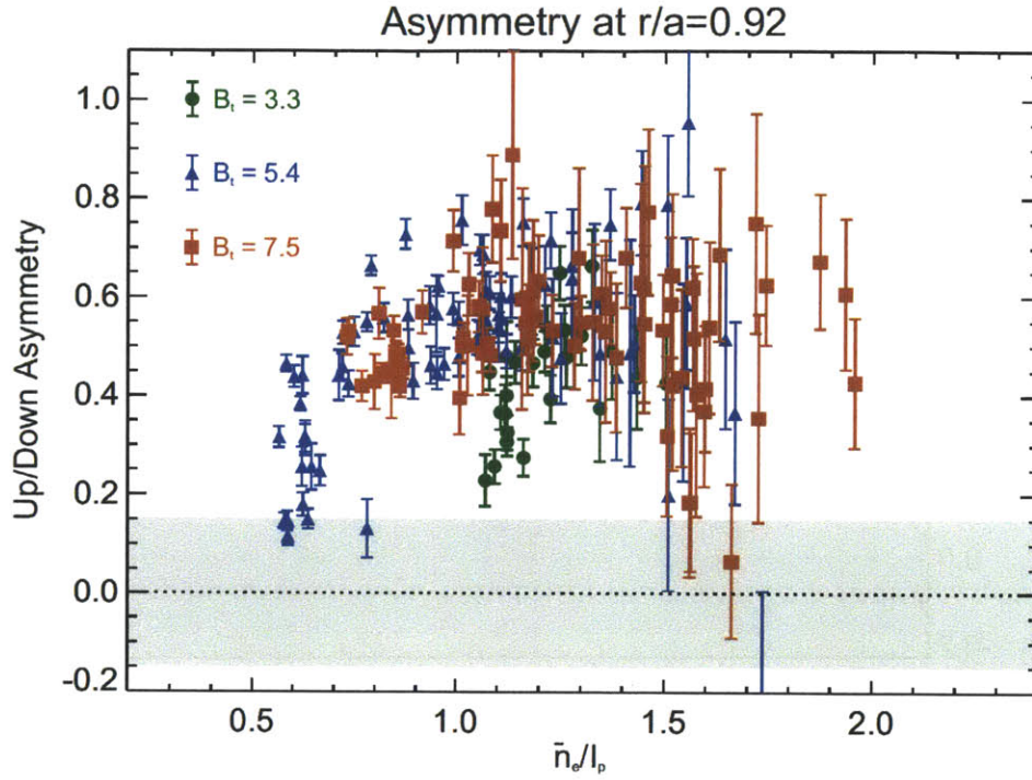
Figure D-12: Up/down asymmetry plotted against \bar{n}_e/I_p for multiple toroidal fields
