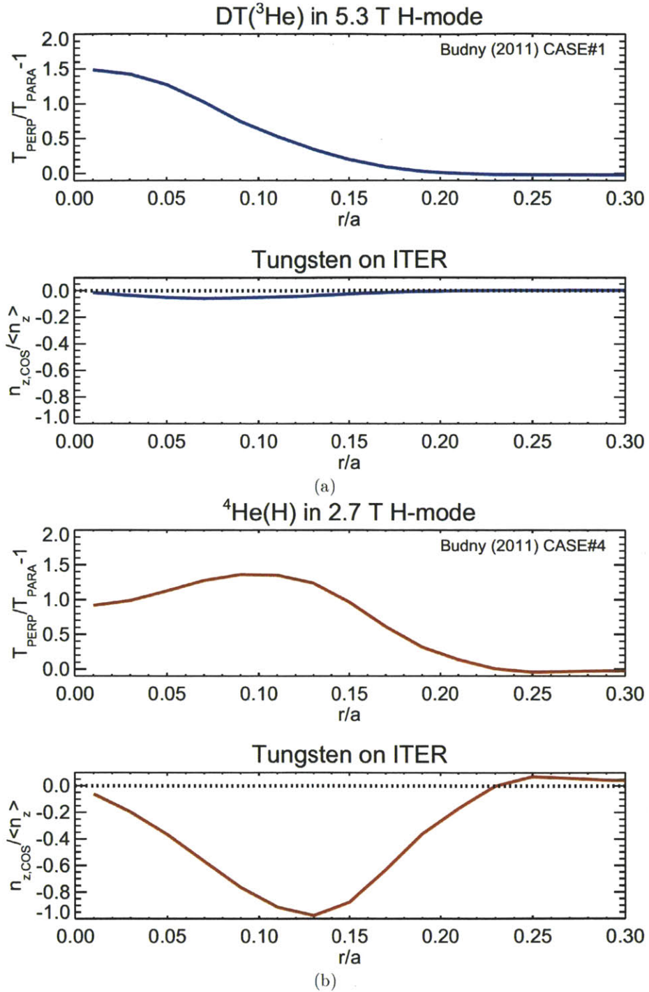
Figure 7-4: Expected asymmetry of tungsten on ITER due to ion cyclotron heating using 3 He minority in a DT plasma (a) and H minority in a 4 He plasma (b) (data from [161])
