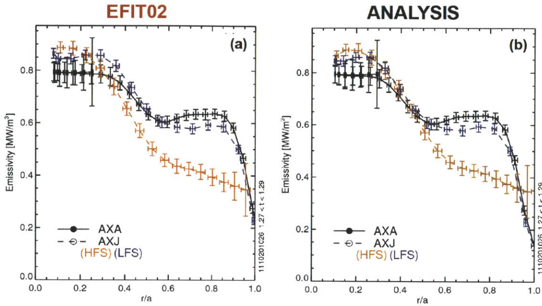
Figure 4-22: Midplane AXUV diode profiles for the 0.7 MA EDA H-mode using a kinetic EFIT (a) and the standard ANALYSIS EFIT (b)
