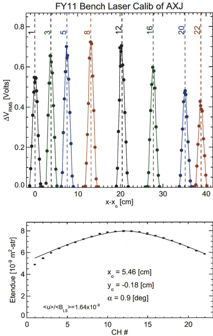
Figure B-16: Results of the AXJ benchtop laser (top) and Labsphere calibrations (bottom) used to find x_0 , y_0 and \alpha
