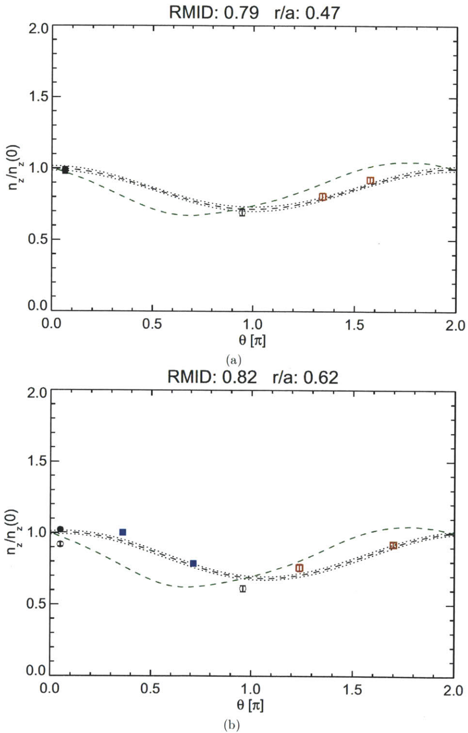
Figure 6-16: Poloidal variation of measured and modeled asymmetries at various r/a for the results shown in Figure 6-15; AXA ( \bullet ), AXJ ( \circ ), WB2AX ( \blacksquare ), WB3AX ( \square ) and WB4AX ( \triangle )
