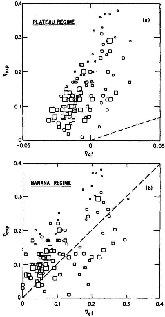
FIG. 7. Experimentally observed values of \eta for C V plotted versus different quantities. (a) Quasi-neoclassical fluid theory scaling, main ions assumed to be in plateau regime: L_T = 10 cm, L_n = 12 cm. (b) same as above, but main ions in banana regime.
