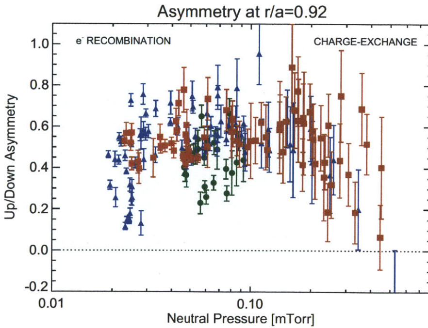
Figure D-13: The up/down symmetry is decreased at large values of main-chamber neutral pressure, p_{neut}
