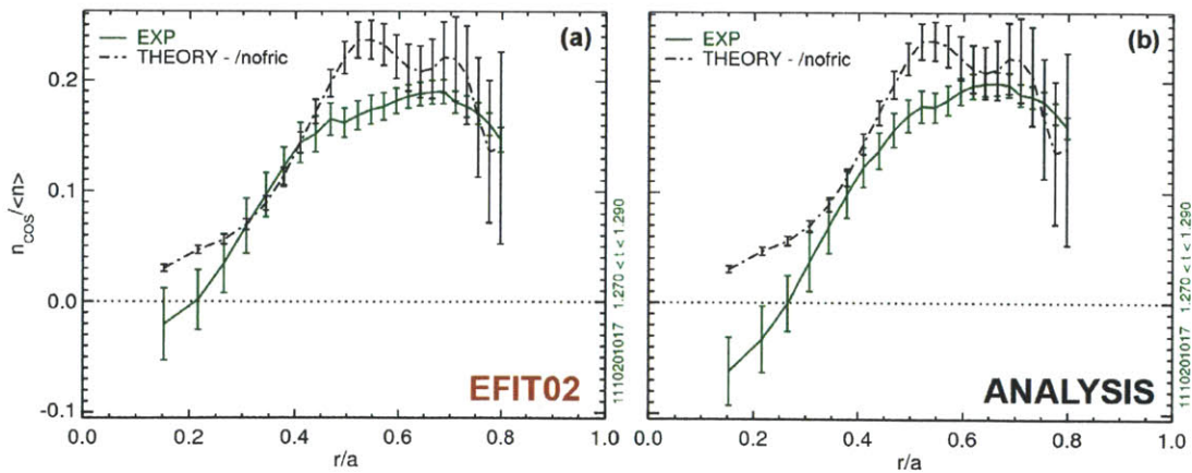
Figure 4-23: Comparison of measured (solid green) and modeled (broken black) radial asymmetry profiles for the 0.9 MA EDA H-mode using a kinetic EFIT (a) and standard ANALYSIS EFIT (b)
