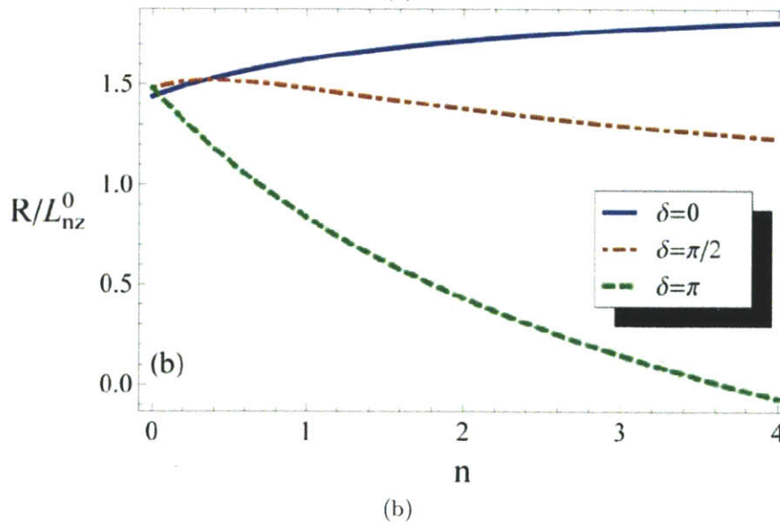
Figure 1-7: Zero flux impurity density scale length sensitivity to magnitude and type of asymmetry (from Fülöp and Moradi [35])
