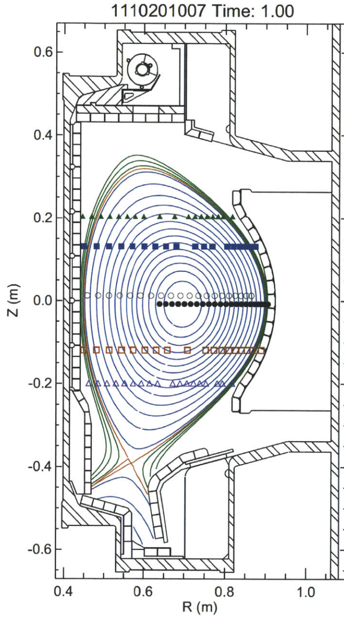
Figure 3-7: The tangency radii of the KLIM and wall box plotted over an H-mode equilibrium reconstruction; AXA ( \bullet ), AXJ ( \circ ), WB1AX ( \blacktriangle ), WB2AX ( \blacksquare ), WB3AX ( \square ) and WB4AX ( \triangle )
