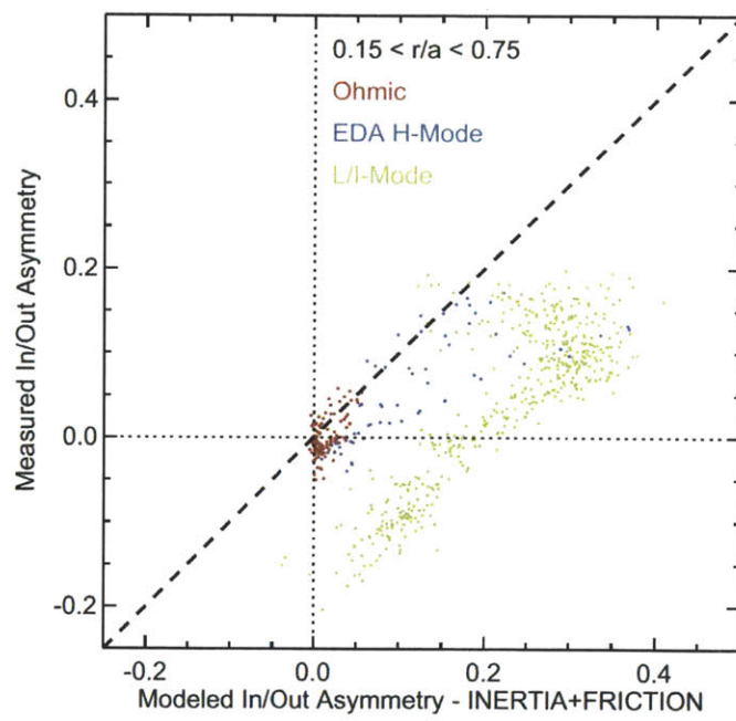
Figure 4-35: Comparison of measured and modeled in/out asymmetries in Ohmic, (low \beta_0 ) EDA H-mode and L/I-mode plasmas including ion-impurity friction, showing little difference from 4-34.
