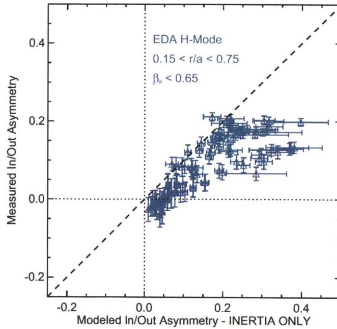
Figure 4-26: Comparison of measured and modeled in/out asymmetry for low \beta_\theta EDA H-mode plasmas (compare with 4-19)
