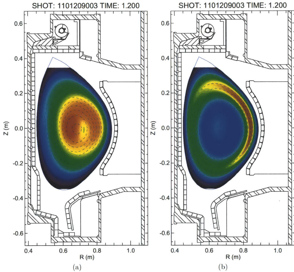
Figure 3-23: 2-D emissivity contour plots for peaked (a) and hollow (b) profiles with specified up/down and in/out asymmetries
