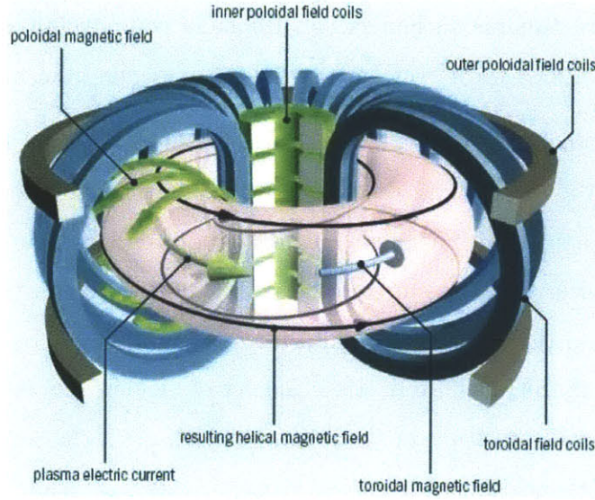
Figure 1-1: Schematic of basic tokamak components ( http://www1.cfi.lu.lv/teor/main.html )
