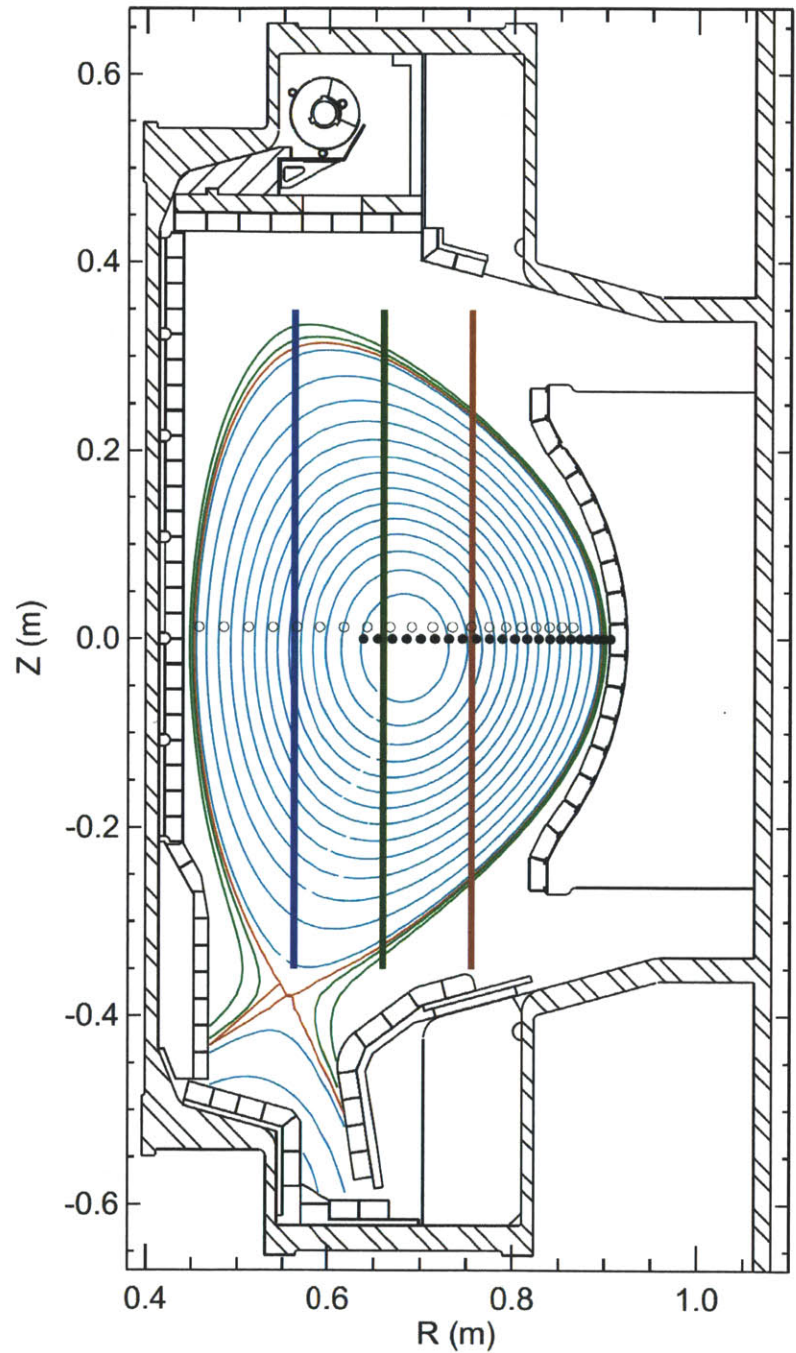
Figure 5-19: Plot of the equilibrium and resonance layer locations for the 70 MHz experiments including the AXA (●), AXJ (○) tangency radii
