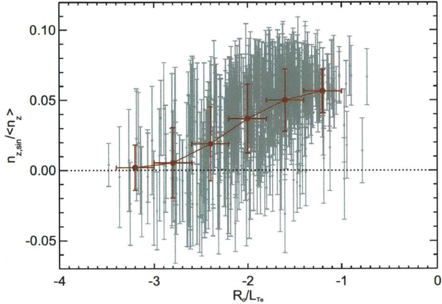
Figure 6-22: Weak correlation of the measured up/down asymmetry with the electron temperature gradient scale length, L_{T_e} = \nabla T_e / T_e , with the full data set (gray) and binned and averaged data (red).
