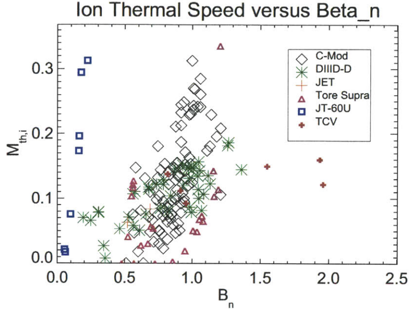
Figure 7-3: Main ion mach number due to intrinsic rotation (from [160])
