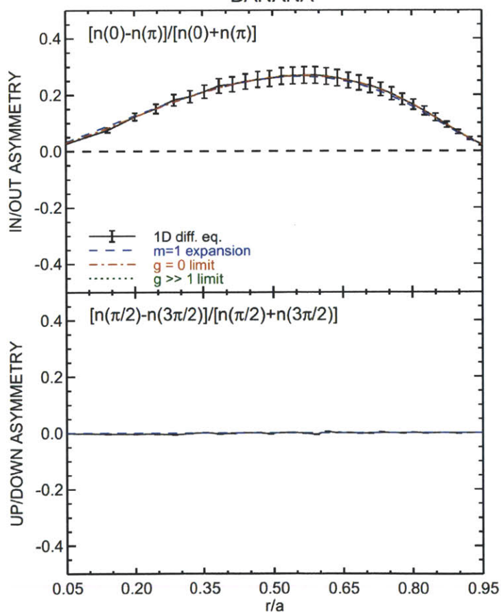
Figure A-5: Comparison of code against analytical limit assuming only toroidal rotation
