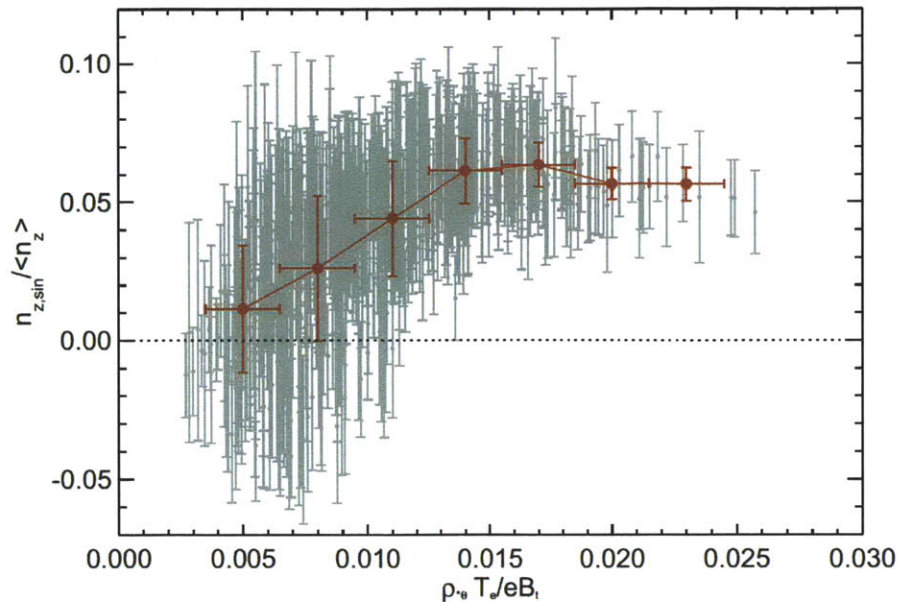
Figure 6-24: Correlation of the measured up/down asymmetry with gyro-Bohm diffusivity, \rho_{*e} T_e / eB_t , with the full data set (gray) and binned and averaged data (red).
