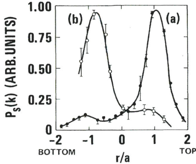
FIG. 2. The spatial distribution of the scattered power ( k_\theta = 9 \text{ cm}^{-1} ) along a vertical chord through plasma center. Curve a I_p, B_T parallel; curve b I_p, B_T antiparallel. Note the large asymmetry which inverts with current reversal.
