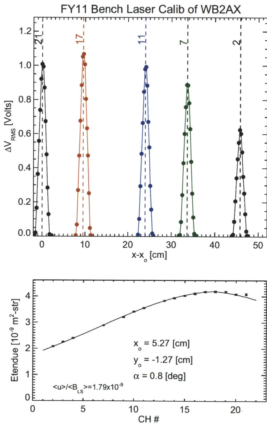
Figure B-17: Results of the WB2AX benchtop laser (top) and Labsphere calibrations (bottom) used to find x_0 , y_0 and \alpha
