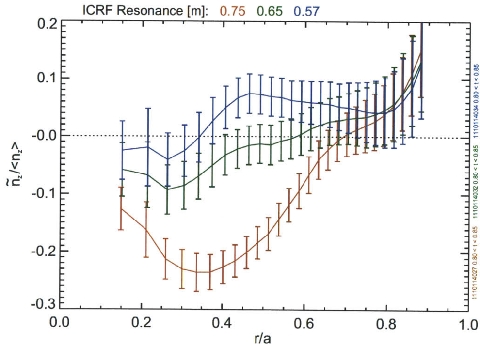
Figure 5-22: Comparison of n_{cos}/\langle n_z \rangle profiles for the resonance layer scan at 70 MHz
