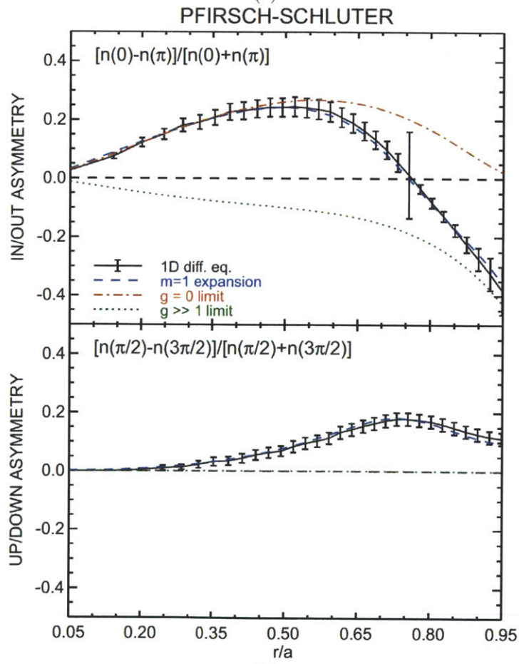
Figure A-9: Comparison of code against Pfirsch-Schlüter-regime theory
