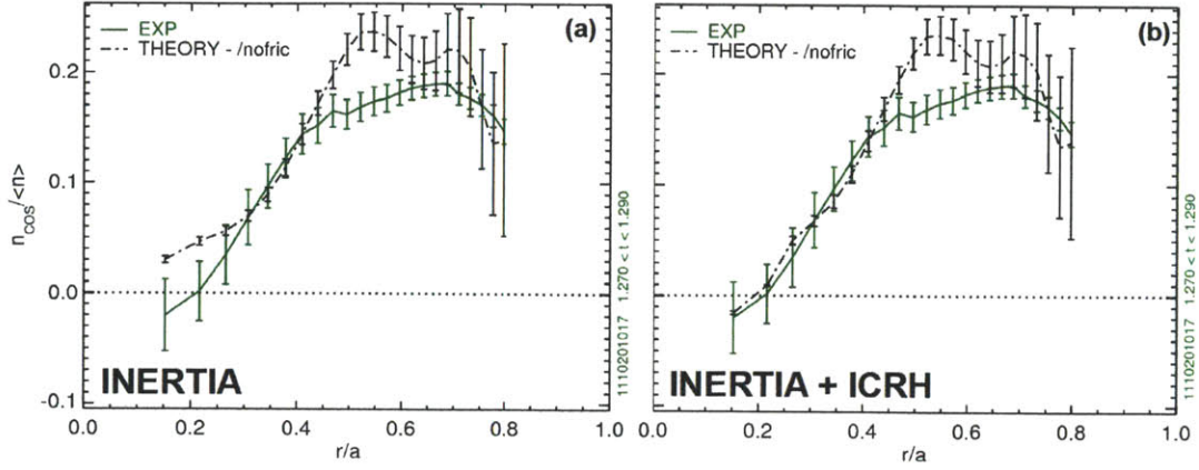
Figure 5-28: Comparison of \bar{n}_z / \langle n_z \rangle in 0.9 MA EDA H-mode to modeling using only inertia (a) and extended theory including inertia and ICRH effects (b)
