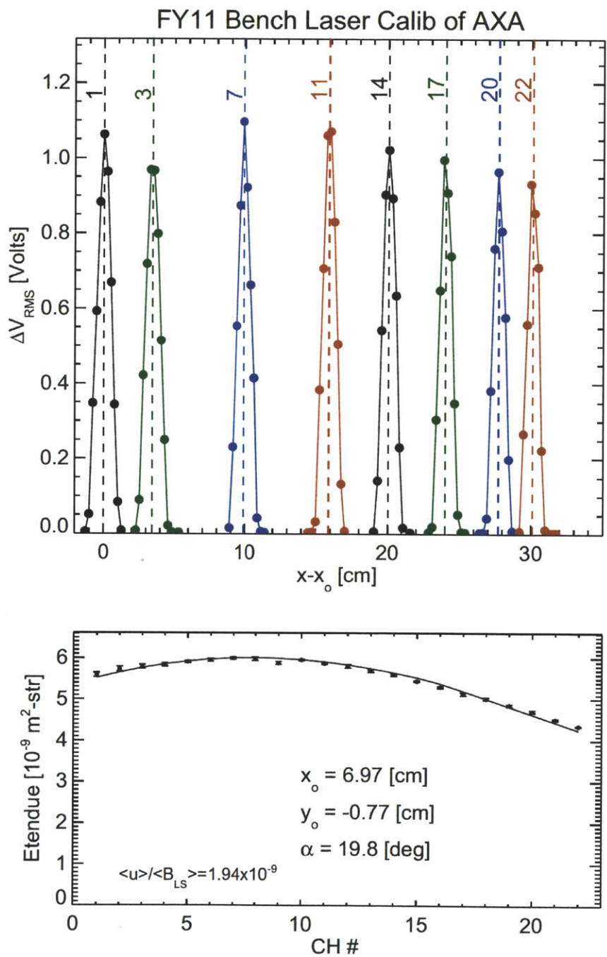
Figure B-15: Results of the AXA benchtop laser (top) and Labsphere calibrations (bottom) used to find x_0 , y_0 and \alpha
