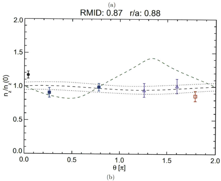
Figure 6-11: Poloidal variation in the impurity density for an EDA H-mode with strong argon radiation; AXA ( \bullet ), AXJ ( \circ ), WB2AX ( \blacksquare ), WB3AX ( \square ) and WB4AX ( \triangle )
