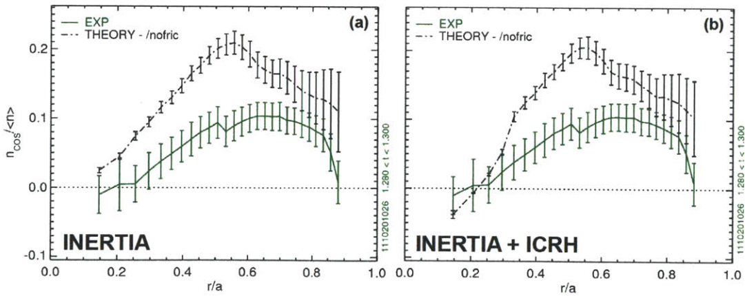
Figure 5-29: Comparison of \bar{n}_z / \langle n_z \rangle in 0.9 MA EDA H-mode to modeling using only inertia (a) and extended theory including inertia and ICRH effects (b)
