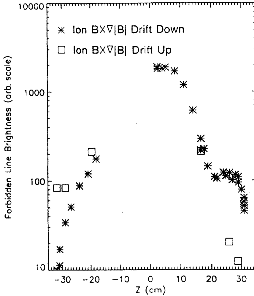
FIG. 6. Vertical brightness profiles for the forbidden line with the ion B \times \nabla|B| drift downward (asterisks) and upward (boxes).
