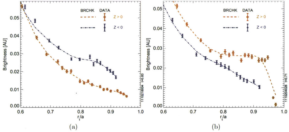
Figure D-9: Comparison of brightness profiles in similar discharges (0.8 MA, 5.4 T plasma at \bar{n}_e \sim 0.5 \times 10^{20} \text{ m}^{-3} ) in reversed (a) and forward (b) field
