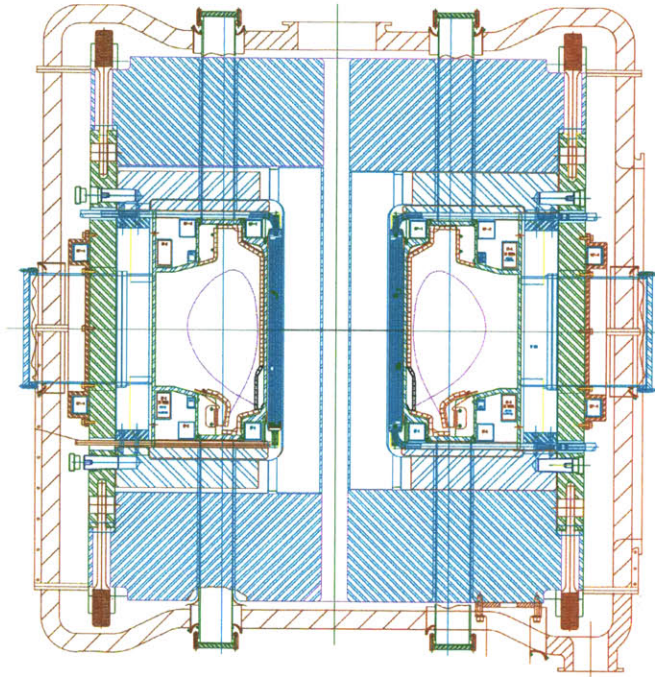
Figure 1-2: Engineering cross-section of the Alcator C-Mod tokamak
