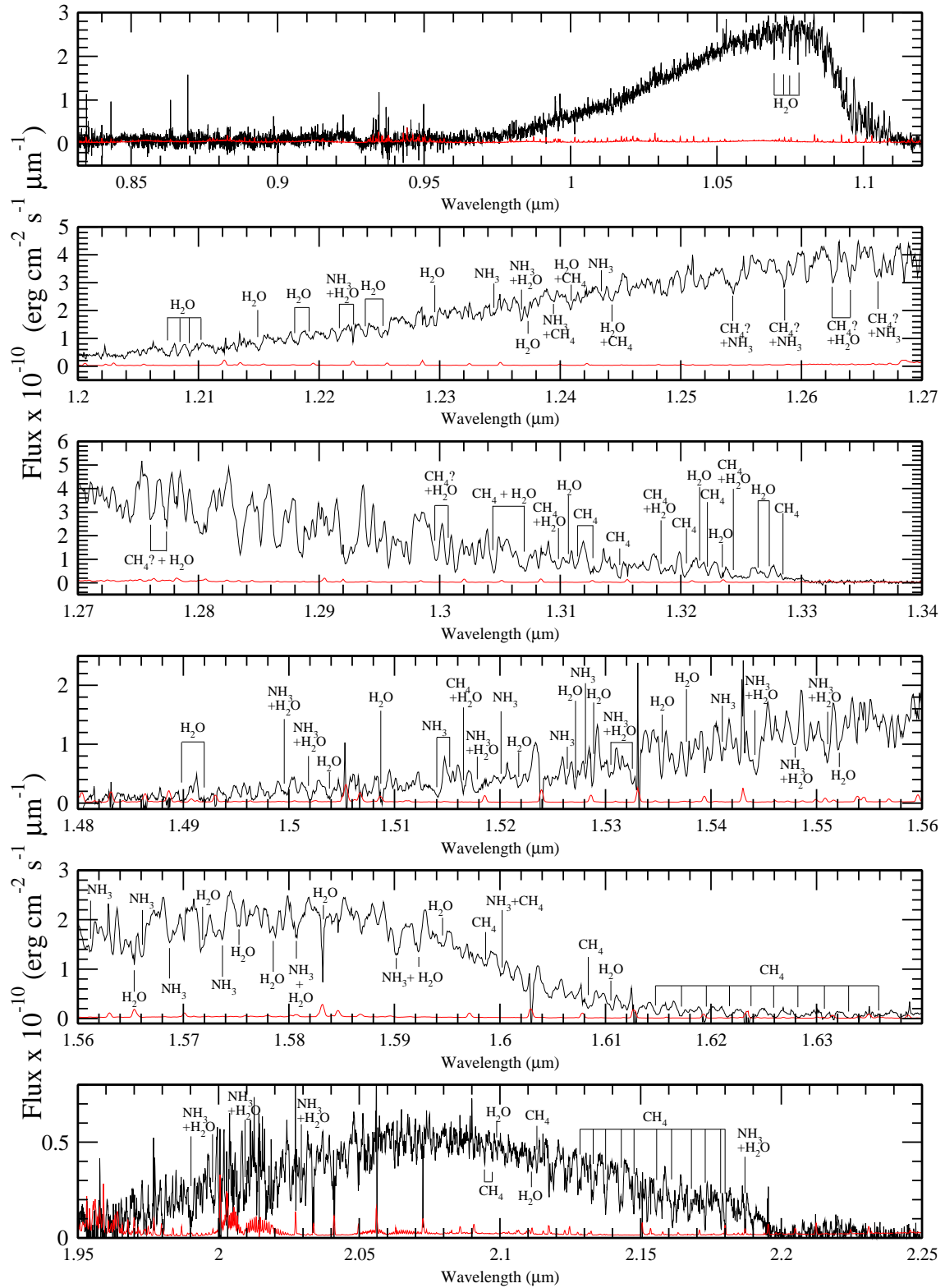
FIG. 3.— FIRE spectrum of UGPS 0722–05 (black line). The noise spectrum is shown in red. Major molecular features are labeled. Some CH 4 features are labeled with a “?” indicating regions where linelists are incomplete, but strong methane absorption has been observed (Fink & Larson 1979).
