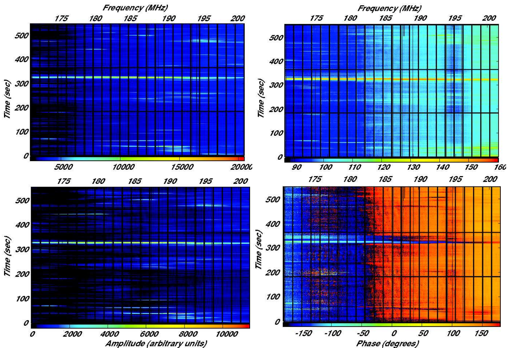
Fig. 2.— Observed visibilities as a function of frequency (XX polarization). The left panels show amplitude (arbitrary units), and the right panels phase (in degrees). The top and bottom rows correspond to baselines with projected lengths of \sim 40\lambda and \sim 196\lambda , respectively, at the band center (186.26 MHz). The frequency ( x -axis) ranges from 170.8 to 201.6 MHz; the time ( y -axis) spans 550 s starting at 04:24:53 UT on 2010 March 27. The horizontal bar below each panel shows the color coded scale and the dark vertical streaks arise from flagging of the coarse channel edges (Sec. 2).
