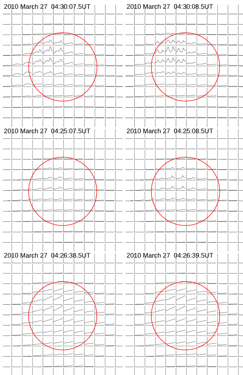
Fig. 5.— Spatially localized spectra of emission across the solar disk at several of the same times shown in Fig. 4. Celestial north is on top, and the red circle marks the size of the optical solar disc. Spectra are shown for every third pixel, where the pixel size is 100'' \times 100'' . The spectra span the entire observing bandwidth, binned into 24 frequency bands spaced 1.28 MHz apart and averaged over 0.8 MHz. The y axis ranges are (in arbitrary units): top row : 50–4996 and 50–4620, respectively; middle row : 100–6000 for both panels; bottom row : 100–1800 for both panels. Animations showing additional frames are available in the on-line journal. The frames corresponding to the bottom two rows have fixed y -axis scales; those for the top row are autoscaled.
