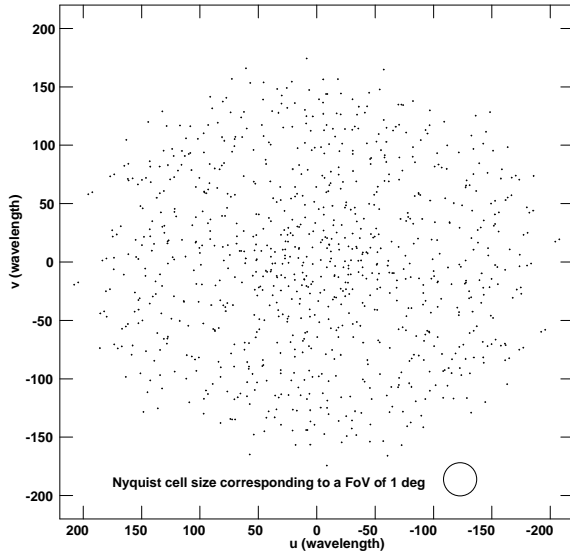
Fig. 1.— The instantaneous uv coverage for a single coarse channel centered at 186.2 MHz. The circle indicates the size of a uv -cell, corresponding to the Nyquist sampling criterion for a 1 degree FoV.
