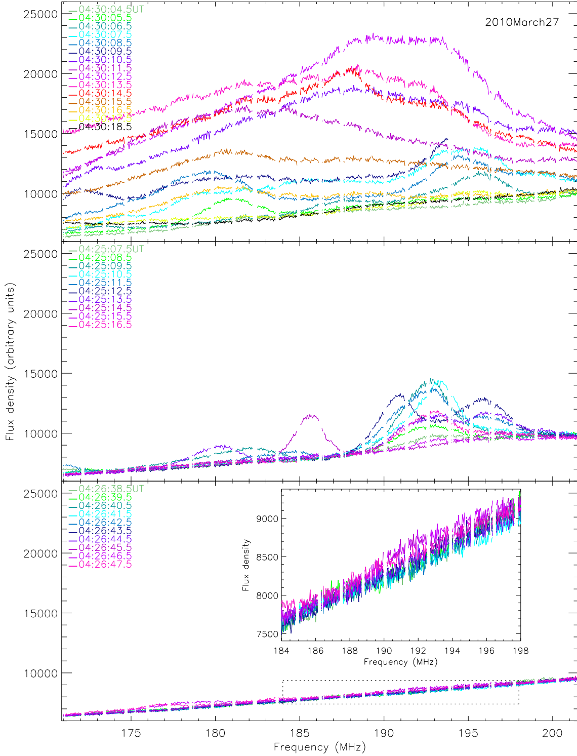
Fig. 3.— Sample autocorrelation spectra from tile 6, X polarization. Top panel: a 14 s period bracketing the most prominent “broadband” feature seen in Fig. 2. Middle panel: variations seen across 10 s for one of the numerous shorter-lived “narrowband” intensity enhancements. Bottom panel: a 10 second interval exhibiting little intensity variation. The inset in the bottom panel zooms in on a part of the band. As with Fig. 2, the data gaps reflect flagged data.
