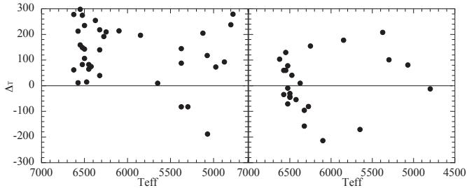
FIG. 7.— Differences between the T_{\text{eff}} derived from flux fitting and those derived from, H\alpha , H\beta , and H\gamma profiles (left), and the medium-resolution H\delta index, HP2 (right).
