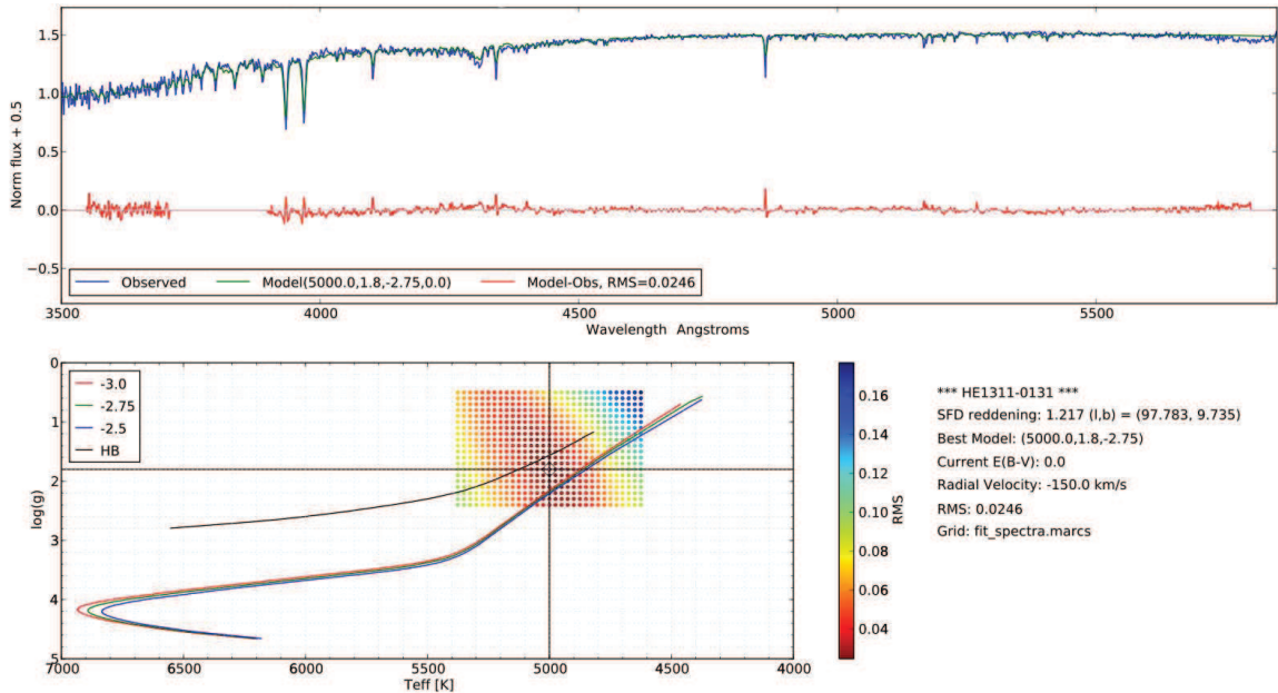
FIG. 5.— The output of fitter . In the top frame the blue line represents the observed spectrum, the green line is the best fitting model spectrum, and the red line is the difference spectrum. In the lower frame the cross-hair marks the best fitting T_{\text{eff}} and \log g and the RMS values of the fits are represented in color for the small subgrid about the initial best fitting parameters. The RMS-color palette is shown ranging from black for best to blue for worst. Any combination of parameters within the black shaded region is acceptable. The halo isochrones are drawn to assist the selection of the most likely parameters.
