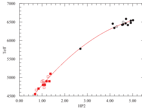
FIG. A1.— T_{\text{eff}} versus HP2 for calibrating stars. Filled black circles represent dwarfs (and one subgiant) from Casagrande et al. (2010); open black circles are dwarfs from the present work; filled red boxes are giants from Cayrel et al. (2004); and open red boxes are the average values for giants from Cayrel et al. (2004) and the present work. The red line is the fitted quadratic relation.
