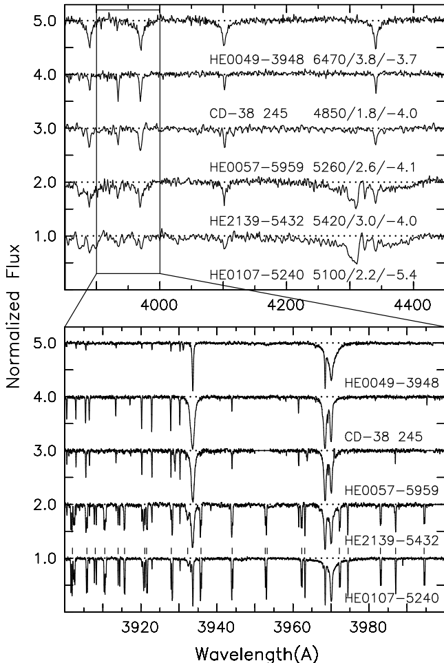
FIG. 2.— Spectra of some of the most metal-poor stars. HE 0049–3948, HE 0057–5959, and HE 2139–5432 are from the present work, while CD–38 o 245 and HE 0107–5240 derive from Bessell & Norris (1984) and Christlieb et al. (2004), respectively, and are shown for comparison purposes. The upper panel presents medium-resolution ( R \sim 1600 ) spectra obtained with the 2.3 m Telescope and cover the range 3850–4450 Å. The numbers in the panel represent T_{\text{eff}}/\log g/[\text{Fe}/\text{H}] from analyses of high-resolution, high- S/N spectra by Christlieb et al. (2004), Norris et al. (2001), the present work, and Paper II. The lower panel shows spectra of the same stars at R \sim 40000 on the range 3900–4000 Å. The reader will note that while the Ca II H & K lines (at 3968.4 and 3933.6 Å, respectively) are very weak in the most metal-poor giant, HE 0107–5240, many more lines have appeared in its spectrum. These are features of CH (the positions of which are indicated immediately above the spectrum) resulting from an extremely large overabundance of carbon relative to iron in this object. We note that HE 2139–5432 is similar to HE 0107–5240 in this respect, but not as metal-poor.
