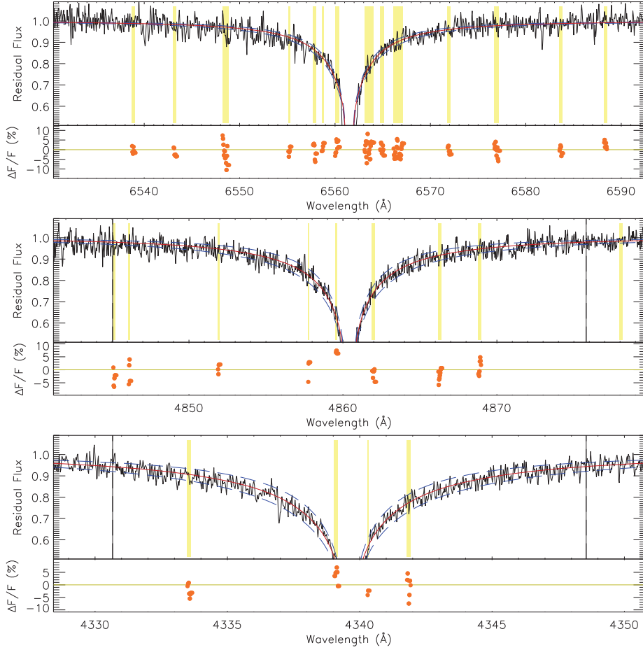
FIG. 6.— Fits to H\alpha , H\beta , and H\gamma line profiles for HE 2047–5612, T_{\text{eff}}(\text{Balmer}) = 6040 K, assuming \log g = 3.6 and [\text{Fe}/\text{H}] = -3.2 . The (black) full lines showing noise are the normalised observed spectra and the (red) smooth full lines the best fit synthetic profile (corresponding to T_{\text{eff}}=6040, 6020, 6080 K for each line, respectively). The (blue) dashed lines show the synthetic spectra calculated with models 200 K cooler and hotter than the best fit. The (yellow) shaded regions show the windows used for determining the \chi^2 statistic in the fitting, and residuals for these regions are shown in the bottom panel. The full vertical lines show the estimated limit of validity of the impact approximation in the self-broadening calculations, which is beyond the limit of the plot for H\alpha . Note that the windows outside this region are rejected in the fitting, and thus no residual is plotted.
