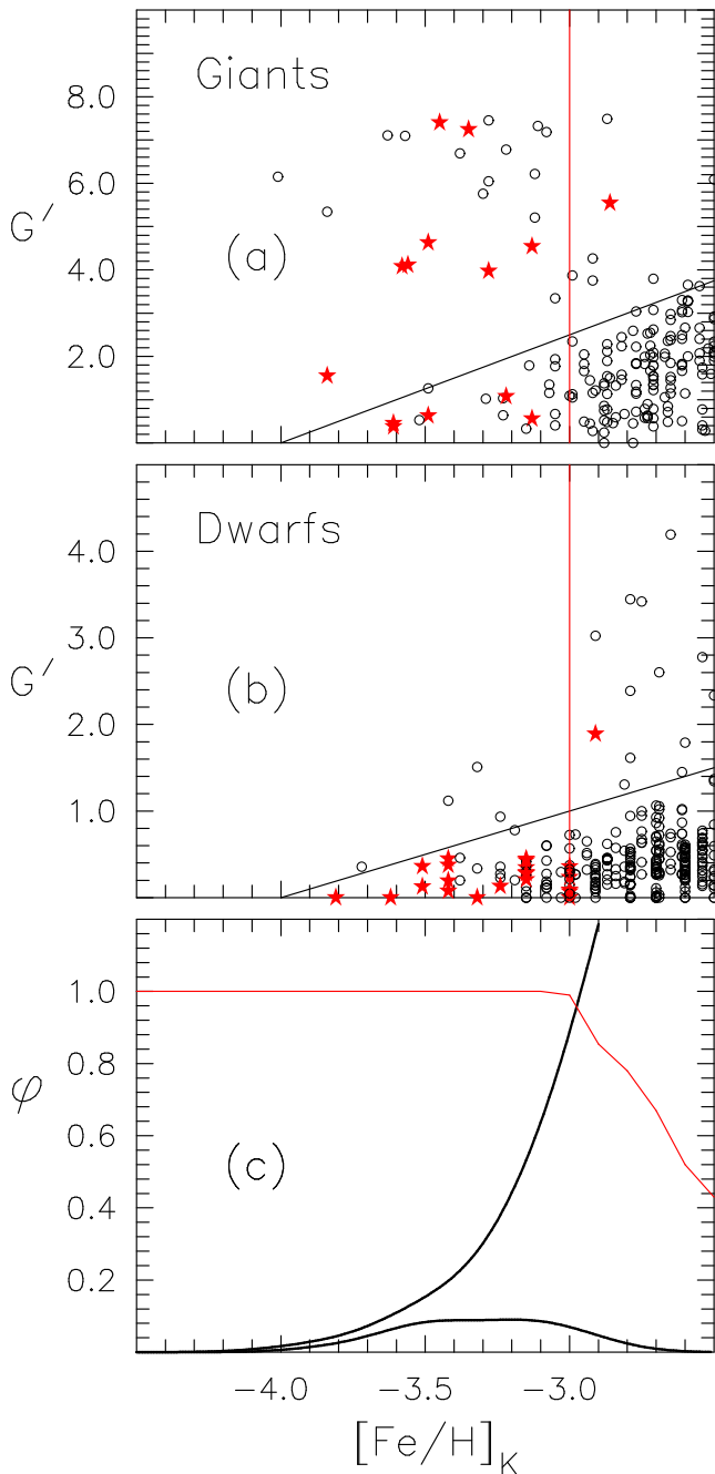
FIG. 1.— G' vs. [\text{Fe}/\text{H}]_{\text{K}} for (a) giants and (b) dwarfs in the Hamburg/ESO survey, measured on medium-resolution spectra obtained with the ANU 2.3 m Telescope. Filled (red) symbols represent stars for which high-resolution, high- S/N spectra have been obtained (in both this and other investigations). Panel (c) presents the generalized histograms (Gaussian kernel with \sigma = 0.15 ) of the MDF for stars in the medium-resolution (upper thick line) and high-resolution (lower thick line) samples. The scale of the ordinate is arbitrary, but is normalized so that the areas under the two distributions have the same proportionality to the numbers of stars in the samples. The principally horizontal, thin line represents the completeness function of the MDF obtained from medium-resolution spectroscopy of the HES, as discussed in the text. (The ordinate runs between 0. and 1.15.)
