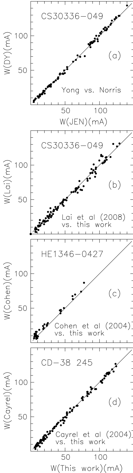
FIG. 3.— Comparison of equivalent widths (a) measured in the present work by J. E. N. and D. Y., and (b)–(d) between the present work and that of (Lai et al. 2008), (Cohen et al. 2004), and (Cayrel et al. 2004).
