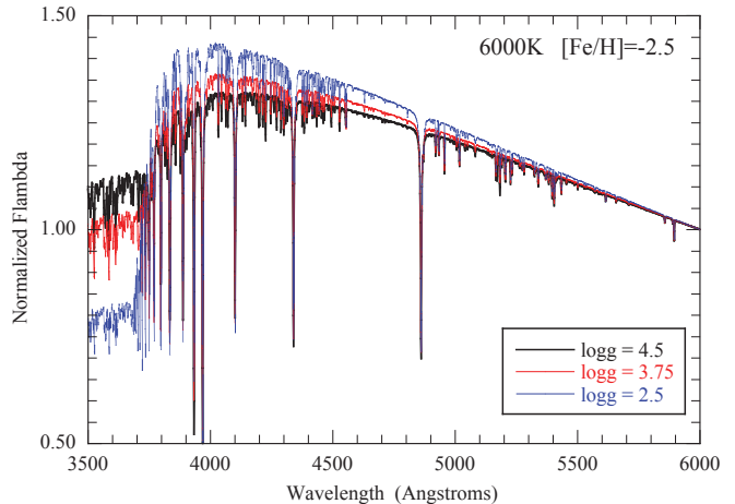
FIG. 4.— The spectrum of three MARCS models with the same T_{\text{eff}} = 6000\text{K} and metallicity [\text{Fe}/\text{H}] = -2.5 but different values of \log g corresponding to the main sequence, subgiant branch, and horizontal branch for halo stars. Note not only the different Balmer Jumps, but the different slopes redward of the Balmer Jump.
