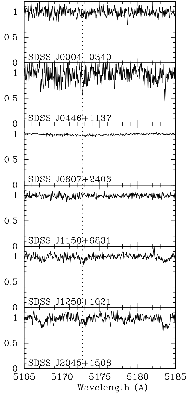
Fig. 10.— Spectra of objects not analyzed in the present work, in the region of the Mg I b lines. The line positions of the triplet are shown by vertical dotted lines.
