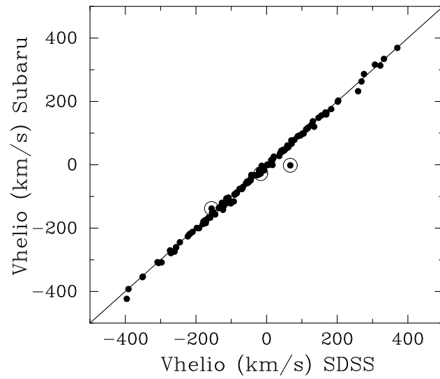
Fig. 2.— Comparison of heliocentric radial velocities measured from the Subaru spectra with those from SDSS spectra. The open circles are over-plotted for the three double-lined spectroscopic binaries. Except for these three stars, the two measurements exhibit excellent agreement.
