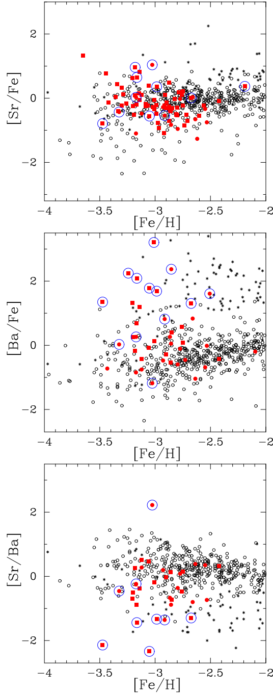
Fig. 9.— Abundance ratios of neutron-capture elements ( [\text{Sr}/\text{Fe}] , [\text{Ba}/\text{Fe}] , and [\text{Sr}/\text{Ba}] ) as a function of [\text{Fe}/\text{H}] . The filled squares and circles (red) indicate main-sequence turn-off and giant stars, respectively. CEMP stars ( [\text{C}/\text{Fe}] > +0.7 ) are over-plotted by large open circles (blue). Small open circles and asterisks indicate the abundance ratios of carbon-normal and carbon-rich stars, respectively, measured by previous studies, which are taken from the SAGA database.
