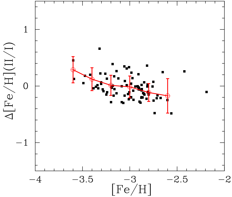
Fig. 5.— The difference of [\text{Fe}/\text{H}] derived from Fe I and Fe II for main-sequence turn-off stars (filled squares). The average and standard deviation for each 0.2 dex bin of [\text{Fe}/\text{H}] are represented by open circles and bars, respectively. The standard deviations are about 0.20 dex, which is as small as the random errors in the abundance measurements. The lowest metallicity range likely suffers from a bias, in that no Fe II line is detected for a larger fraction of stars than the less metal-poor stars. (See text for details.)
