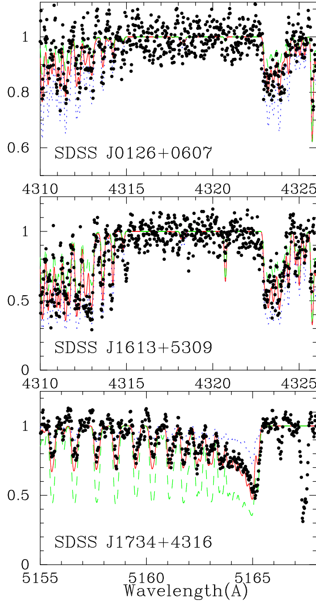
Fig. 6.— Spectra of the CH G-band/4323 Å band and the C 2 Swan band at 5165 Å, for the stars labeled in each panel (filled circles). The three synthetic spectra are calculated by changing [C/Fe] by 0.3 dex (dashed and dotted lines) around the adopted values (solid line).
