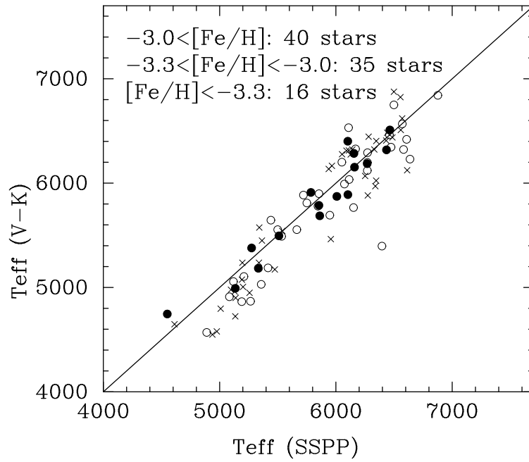
Fig. 4.— Comparison of T_{\text{eff}} , estimated by the (recent) SSPP, and those from (V - K)_0 . The sample is separated into three metallicity ranges ( [\text{Fe}/\text{H}] < -3.3 : filled circles, -3.3 < [\text{Fe}/\text{H}] < -3.0 : open circles, and -3.0 < [\text{Fe}/\text{H}] : crosses).
