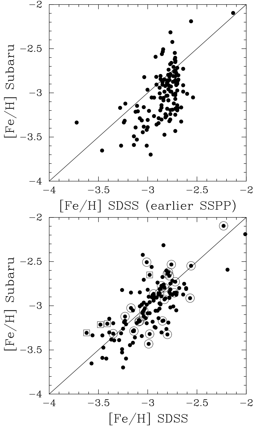
Fig. 1.— Upper panel: Comparison of [\text{Fe}/\text{H}] , based on the snapshot Subaru high-resolution spectra, with those estimated from medium-resolution SDSS spectra, based on the version of the SSPP in use prior to 2008. Lower panel: Same as the upper panel, but using estimates from the latest version of the SSPP. Large open circles and squares are over-plotted for giants and cool main-sequence stars, respectively. The level of improvement in the SSPP is clear.
