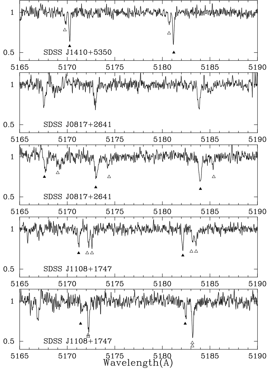
Fig. 7.— Spectra around the Mg b lines of double-lined and triple-lined spectroscopic binaries: SDSS J1410+5350 (the top panel), SDSS J0817+2641 (second and third panels), and SDSS J1108+1747 (the lower two panels). The filled triangles indicate the primary Mg I b lines for each star, while the open triangles show the secondary ones.
