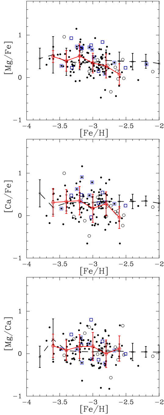
Fig. 8.— Abundance ratios of [\text{Mg}/\text{Fe}] (top panel), [\text{Ca}/\text{Fe}] (middle panel), and [\text{Mg}/\text{Ca}] (bottom panel), with respect to [\text{Fe}/\text{H}] . The filled and open circles indicate main-sequence turn-off and giant stars, respectively. CEMP stars ( [\text{C}/\text{Fe}] > +0.7 ) are shown by over-plotting open squares. Large open circles and bars, connected by a solid line (red), represent the average and standard deviation of the abundance ratios, respectively, for each metallicity bin of width 0.2 dex for our SDSS sample. The standard deviations are 0.20–0.25 dex, which are as small as the random errors in the abundance measurements. Crosses and bars, connected by a dashed line, indicate those for the SAGA sample (see text).
