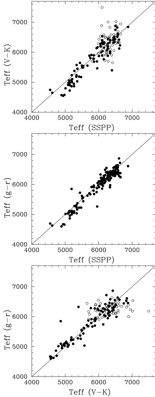
Fig. 3.— Comparison of T_{\text{eff}} estimated by the (recent) SSPP and that from (V - K)_0 (top panel) and from (g - r)_0 (middle panel). The bottom panel shows the comparison of T_{\text{eff}} between the two color indices. The open circles indicate objects with large errors in their K -band photometry.
