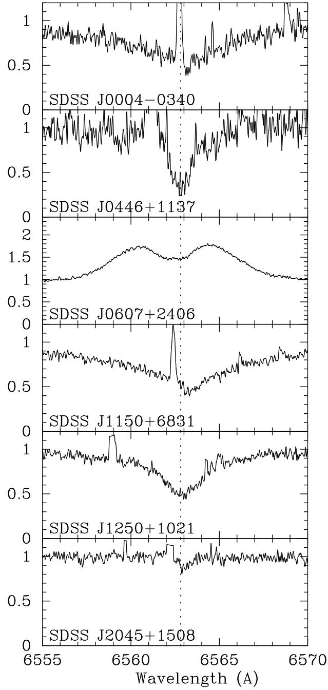
Fig. 11.— The same as Fig. 10, but for the H \alpha region. The line position is shown by a vertical dotted line. Sky emission features are not fully removed in this region.
