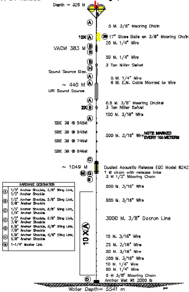
Figure G-2: Schematic drawing for Mooring B, 2005 - 2007.
