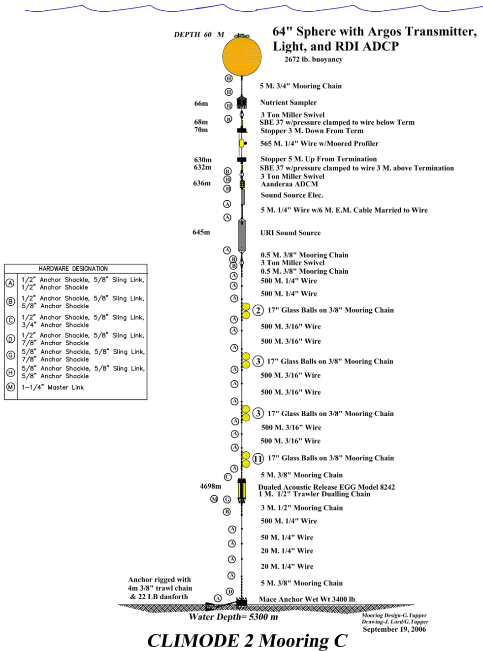
Figure G-5: Schematic drawing for Mooring C2, 2006 – 2007.
