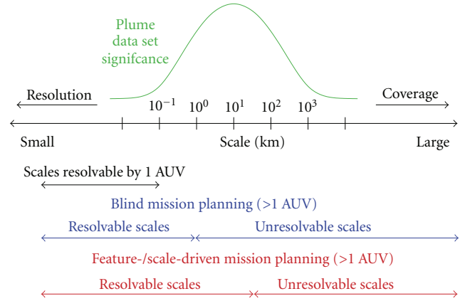
FIGURE 2: This figure depicts the characteristic length scale (in km) of an O(1 km) plume in the horizontal plane. A similar figure can be drawn for the temporal dimension based on the characteristic time scale of a plume (with units of time). If we assume a plume has an approximate Gaussian distribution over its characteristic length scale, as shown here, we must plan AUV missions, such that the collective sampling of our AUVs overlaps with the primary length scale of the plume to optimize over coverage and resolution (“feature-/scale-driven” mission planning). This will improve the range of resolvable length scales in the resulting data set over that of “blind” mission planning, especially when the AUVs’ distribution is “driven” by the characteristic spatiotemporal scales of the plume. Adapted from [12].
