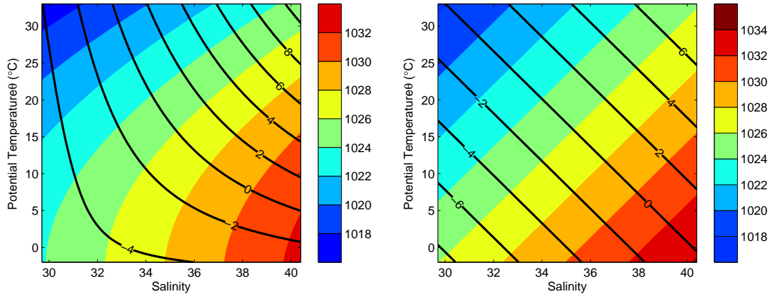
Figure 2-1: Contours of constant density (isopycnals) and constant spice are indicated by filled contours and solid lines, respectively. While the full nonlinear equation of state is used to produce the left panel, the linear approximations (Eqs. 2.31, 2.32) are shown in right panel. The spice zero-crossing is chosen as S=35 , \theta=0 .
