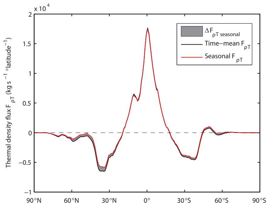
Figure 5-4: Comparison of F_{\rho T} with and without seasonal effects. Seasonal effects add a further nonlinearity which increases the global area integral of buoyancy forcing by 35 %. The greatest increases can be seen between 20^\circ and 60^\circ due to the strong seasonal cycle in that latitude band.
