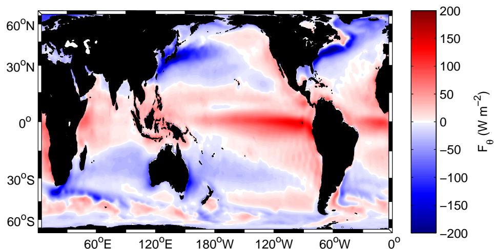
Figure 4-1: Surface heat flux F_\theta \text{W m}^{-2} . The main gradient is meridional between equators and poles. This pattern is modified by heat entering the ocean in tropical regions and along areas of coastal upwelling, such as the West Coast of Africa. Strong heat losses are also evident over all Western Boundary Currents.
