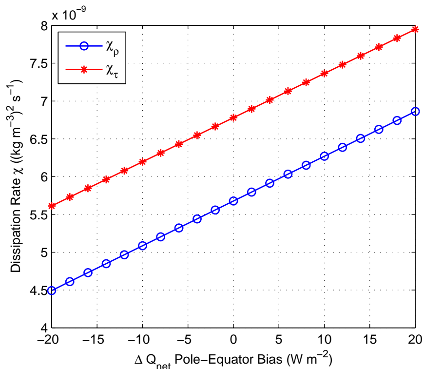
Figure 4-50: Sensitivity of \chi_\rho and \chi_\tau to a linear Q_{net} bias between 90° latitude and the equator. Positive values indicate the additional difference in forcing (in \text{W m}^{-2} between the poles and the equator. Negative values indicate that the additional difference results in greater Q_{net} at the poles and a reduced Q_{net} at the equator. The relationship is linear in both cases, with \chi_\rho being marginally more sensitive to changes in \Delta Q_{net} .
