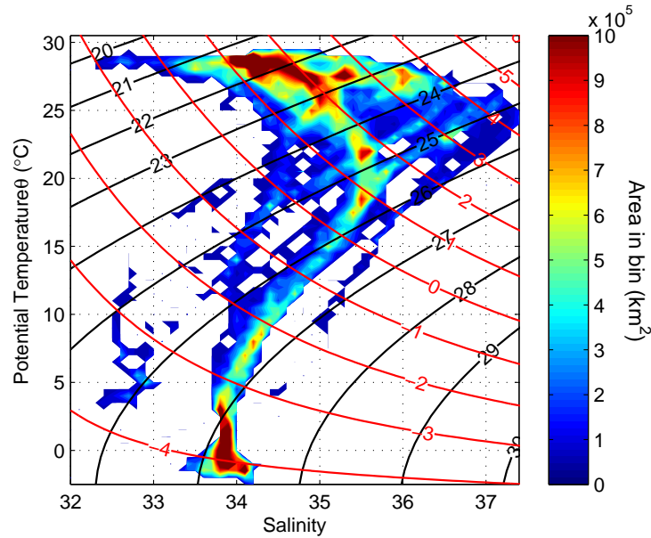
Figure 4-2: Total surface area ( \text{km}^2 ) for each potential temperature and salinity bin. The bin separation is 0.1 in salinity and 0.5^\circ\text{C} in potential temperature.
