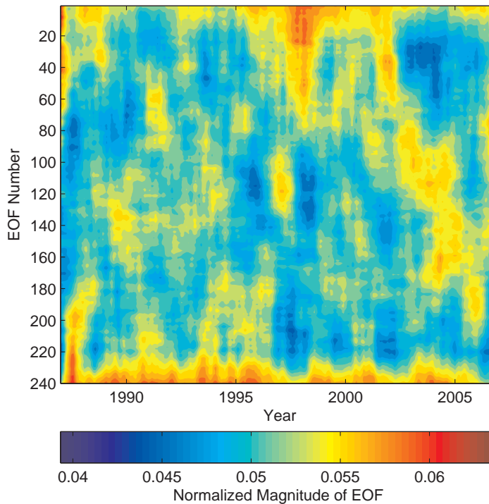
Figure 3-7: Filtered results of principal component analysis (PCA) of the OAFflux/ISCCP Q_{net} estimate. The magnitude of all PCAs (color-coded) is plotted with respect to time and the number of the PCA. In this analysis, no significant changes in patterns are observable between 1987 and 2006. An ENSO signal is evident between 1997–1998.
