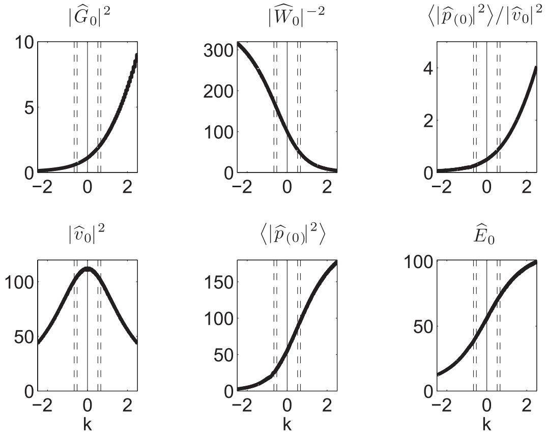
FIG. 10. Response of oceanic MRG wave to antisymmetric zonal winds with Hermite expansion coefficient X_1 = 1.5 . Figure format as in Fig. 5.
