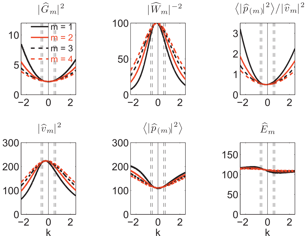
FIG. 6. Response of lowest four oceanic meridional modes to zonal winds with meridional structures characterized by constant Hermite expansion coefficients (top panel, Fig. 4). Symmetric oceanic meridional modes ( m odd) are forced by the symmetric X_s = 1.5 \sum_{n=0}^{\infty} \psi_{2n}(y) . Antisymmetric oceanic modes ( m even) are forced by the antisymmetric X_a = 1.5 \sum_{n=0}^{\infty} \psi_{2n+1}(y) . Figure format as in Fig. 5.
