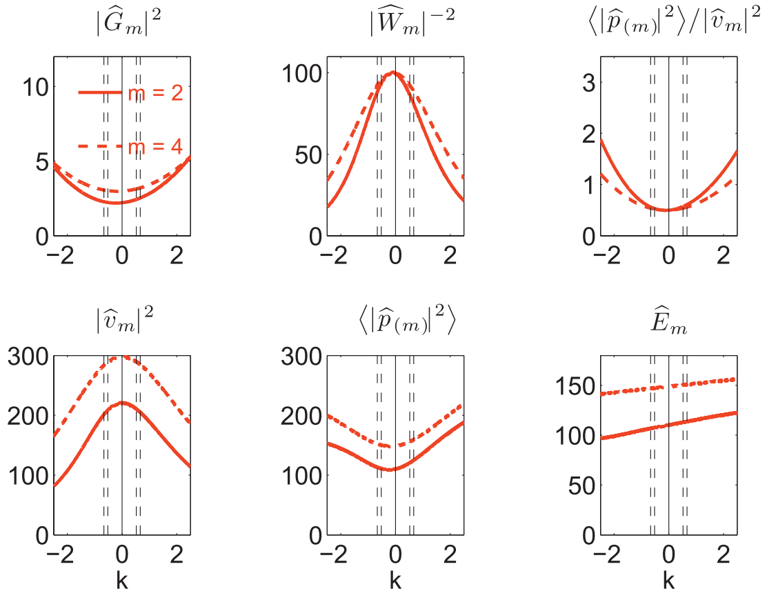
FIG. 8. Response of oceanic modes 2 and 4 to antisymmetric zonal winds: X_a = y/2 (middle panel, Fig. 4). Figure format as in Fig. 5.
