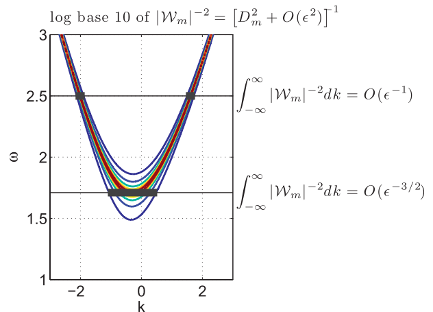
FIG. 3. Conceptual conversion from wavenumber–frequency spectrum to frequency spectrum. The integral over all wavenumbers of the inverse-square dispersion polynomial is larger at the modal frequency minimum than at higher frequencies because the band of wavenumbers that make significant contributions to the integral is largest at this frequency. Maximum resonance is found on the free-wave dispersion curve where D_m = 0 .
