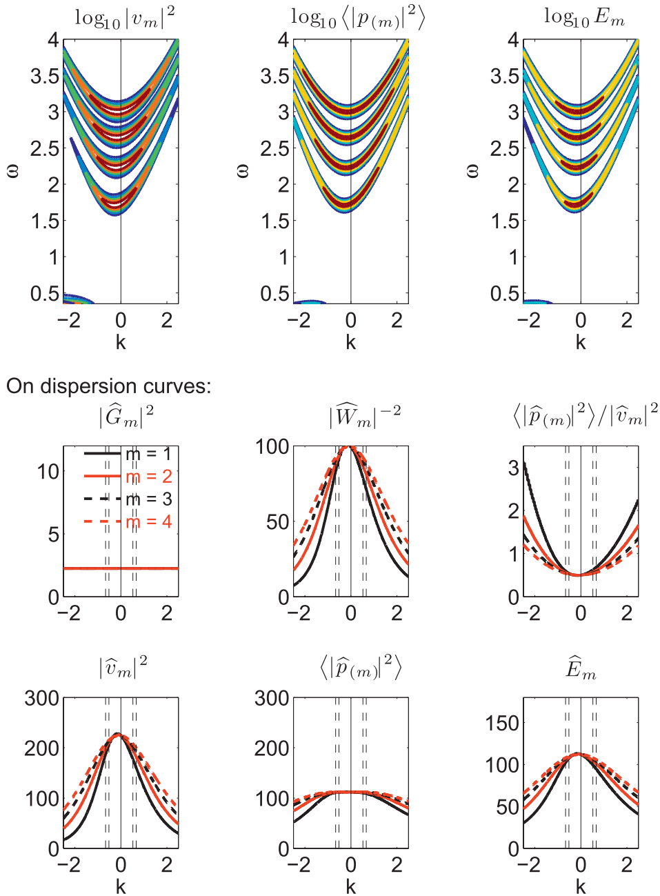
FIG. 5. Response of lowest 4 oceanic meridional modes to meridional winds with meridional structures characterized by constant Hermite expansion coefficients (top panel, Fig. 4). Symmetric oceanic meridional modes ( m odd) are forced by the antisymmetric Y_a = 1.5 \sum_{n=0}^{\infty} \psi_{2n+1}(y) . Antisymmetric oceanic modes ( m even) are forced by the symmetric Y_s = 1.5 \sum_{n=0}^{\infty} \psi_{2n}(y) . (top) Wavenumber–frequency spectra of log base 10 of (left to right) meridional velocity |v_m|^2 , integrated pressure \langle |p_{(m)}|^2 \rangle and total wave energy E_m . (middle) Wavenumber dependence of contributions to resonance solutions, calculated on the free-wave dispersion curves (at maximum resonance). (left to right) the squared forcing function |\hat{G}_m|^2 [see (40)–(41)], the inverse squared dispersion function |\hat{W}_m|^{-2} [see (46)] and the ratio of integrated squared pressure to integrated squared meridional velocity \langle |\hat{p}_{(m)}|^2 \rangle / |\hat{v}_m|^2 [see (17)–(18)]. (bottom) Wavenumber dependence of the spectra in the top row, calculated on the free-wave dispersion curves (at maximum resonance). (left to right) |\hat{v}_m|^2 , \langle |\hat{p}_{(m)}|^2 \rangle and \hat{E}_m . Mode numbers are as labeled in the middle left panel. Dashed vertical lines show the nominal Nyquist wavenumbers of the TAO/TRITON array ( \pm 1 cycle per 30^\circ longitude) for baroclinic modes 1 and 2 (nearest k = 0 ).
