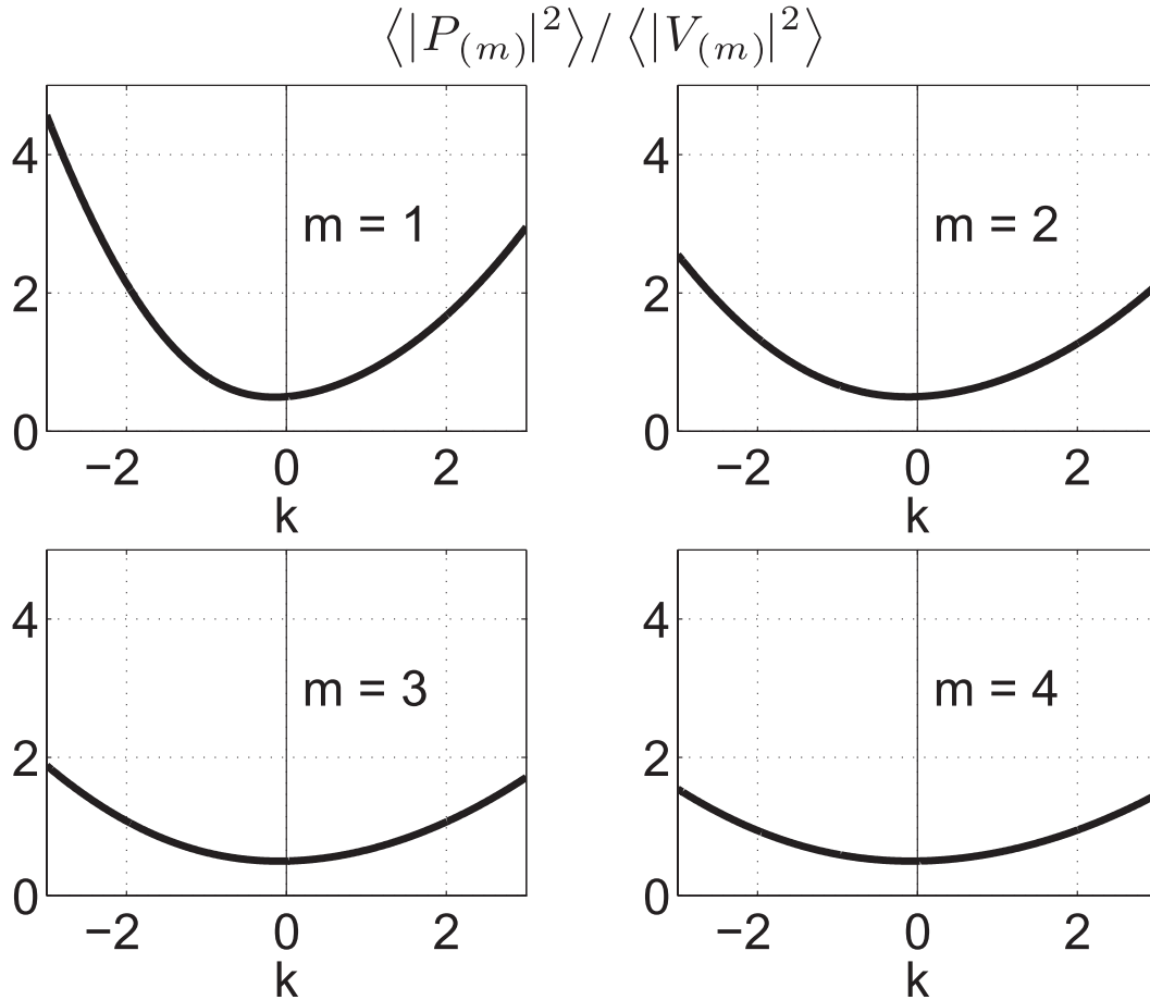
FIG. 2. Wavenumber dependence of the ratio of integrated pressure variance to integrated meridional velocity variance for the free inertia–gravity waves, where the integration is over latitude; meridional modes 1–4. This ratio is exactly the integrated variance of pressure for the “unit amplitude” wave because the integrated variance of meridional velocity is 1 by definition for this wave. We retain the ratio designation to emphasize its use as a conversion factor between forced solutions for meridional velocity and those for pressure. The minimum falls between k = 0 and the wavenumber associated with vanishing group velocity.
