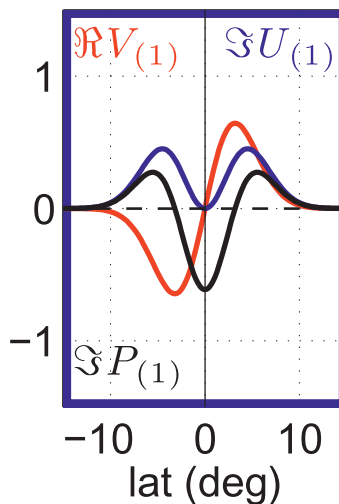
FIG. 1. (top) Dispersion curves for unforced MRG wave ( m = 0 ) and lowest four meridional modes of inertia-gravity waves. (bottom) Meridional structures of meridional mode-1, unit amplitude free-wave components. The color of the box in a bottom panel corresponds to the color of the dot on the m = 1 dispersion curve in the top panel where the wave structures were calculated. In each bottom panel, the real part of the meridional velocity is displayed in red, while the imaginary parts of the zonal velocity and pressure are displayed in blue and black, respectively. Note that the structure and amplitude of the meridional velocity do not change with wavenumber. Both the structure and the amplitude of zonal velocity and pressure are wavenumber dependent. Latitude has been scaled appropriately for baroclinic mode 1 in the central equatorial Pacific. Equivalent structures for baroclinic mode 2 are compressed toward the equator by about 20%.
