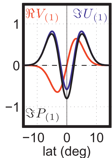
FIG. 1. (top) Dispersion curves for unforced MRG wave ( m = 0 ) and lowest four meridional modes of inertia-gravity waves. (bottom) Meridional structures of meridional mode-1, unit amplitude free-wave components. The color of the box in a bottom panel corresponds to the color of the dot on the m = 1 dispersion curve in the top panel where the wave structures were calculated. In each bottom panel, the real part of the meridional velocity is displayed in red, while the imaginary parts of the zonal velocity and pressure are displayed in blue and black, respectively. Note that the structure and amplitude of the meridional velocity do not change with wavenumber. Both the structure and the amplitude of zonal velocity and pressure are wavenumber dependent. Latitude has been scaled appropriately for baroclinic mode 1 in the central equatorial Pacific. Equivalent structures for baroclinic mode 2 are compressed toward the equator by about 20%.
