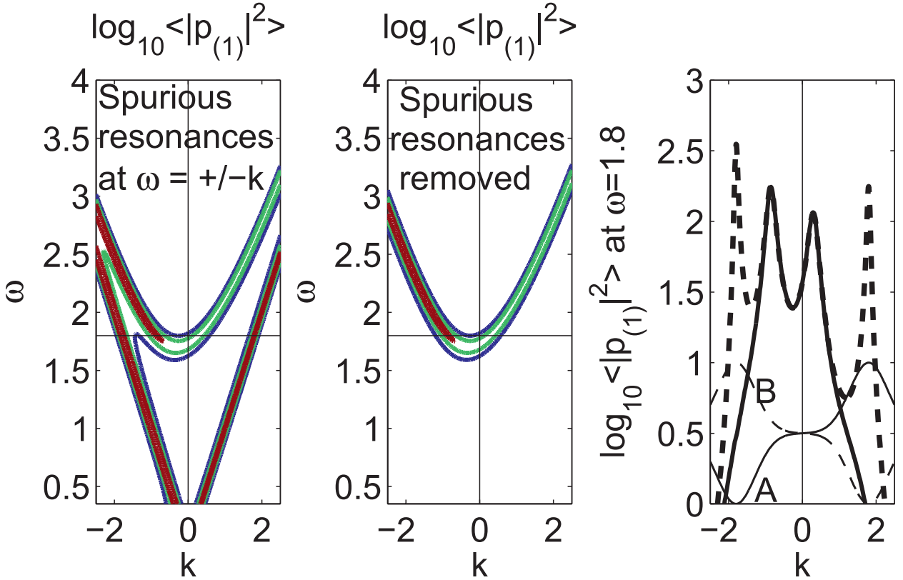
FIG. A1. Suppression of spurious resonances. Wavenumber–frequency spectra for inertia–gravity mode 1 forced by X = 1 when the forcing terms in (A18) are (left) not included and (middle) included. (right) Transect through the previous two panels at \omega = 1.8 (horizontal lines in left two panels). Displayed is \langle |p_{(1)}|^2 \rangle vs k when the forcing terms in (A18) are (solid) included and (dashed) not included. Also shown are the wavenumber dependencies of (solid) A(k, \omega) and (dashed) B(k, \omega) at \omega = 1.8 .
