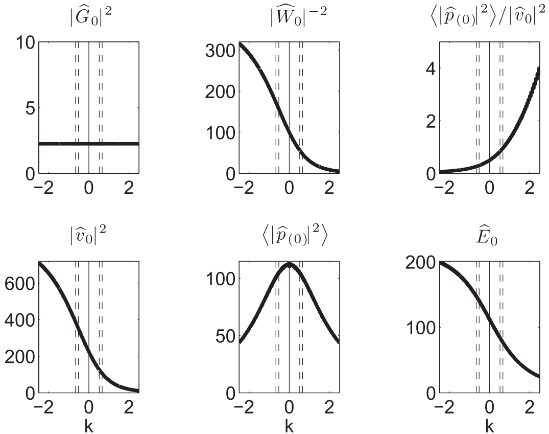
FIG. 9. Response of oceanic MRG wave to symmetric meridional winds with Hermite expansion coefficient Y_0 = 1.5 . Figure format as in Fig. 5.
