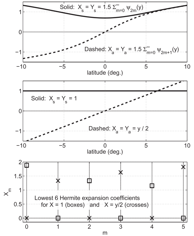
FIG. 4. Meridional structures of idealized symmetric and anti-symmetric forcing scenarios: (top) structures with constant Hermite expansion coefficients, X_s = Y_s = 1.5 \sum_{m=0}^{\infty} \psi_{2m}(y) (solid curve), and X_a = Y_a = 1.5 \sum_{m=0}^{\infty} \psi_{2m+1}(y) (dashed curve); (middle) lowest-order approximations to large-scale symmetric and antisymmetric forcing structures, X_s = 1 (solid curve) and X_a = y/2 (dashed curve). In each panel, latitude is scaled appropriately for baroclinic mode 1. (bottom) Lowest six Hermite expansion coefficients for X_s = 1 (boxes) and X_a = y/2 (crosses).
