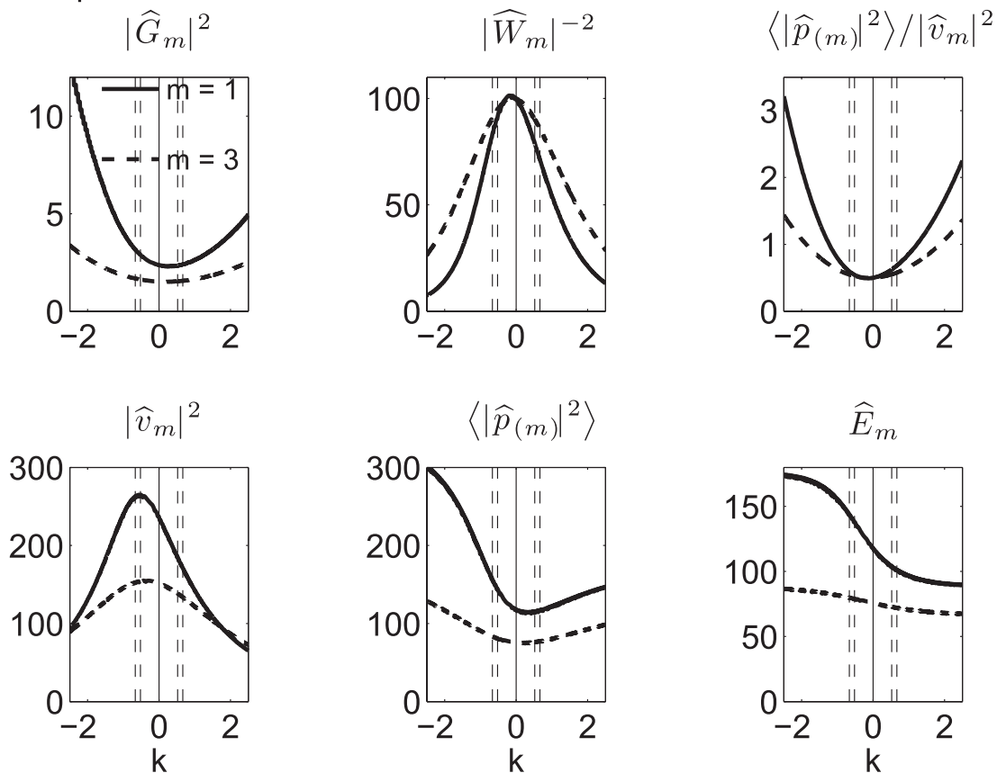
FIG. 7. Response of oceanic modes 1 and 3 to zonal winds that are uniform in latitude: X_s = 1 (middle panel, Fig. 4). Figure format as in Fig. 5.
