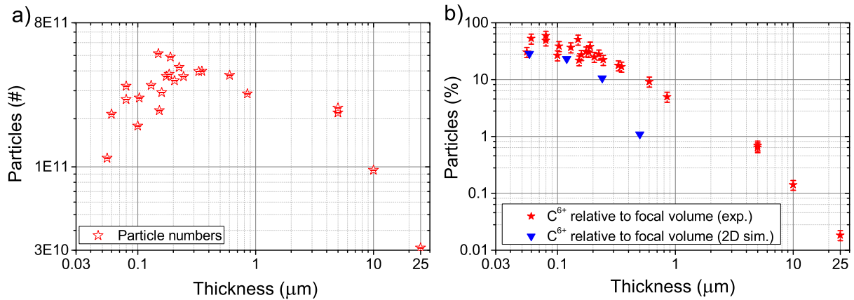
Figure 2. Measured carbon C 6+ particle numbers above the detection threshold of 33 MeV (a) as a function of target thickness and (b) as a function of laser focal volume for thicknesses of 50 nm to 25 μm encompassing BOA (<700 nm) and TNSA (>>700 nm) dominated acceleration regimes. The experimental data are represented by red stars and the simulation results by blue triangles. The laser focal volume is given by the target thickness and the focal spot area (3.8 μm radius for experimental data and 3w with w = 5.12 \mu\text{m} for simulation data). Errors for particle numbers are derived assuming a Poisson distribution and do not account for systematic errors due to rotational symmetry assumption. Error bars in (b) include uncertainty in the focus diameter.
