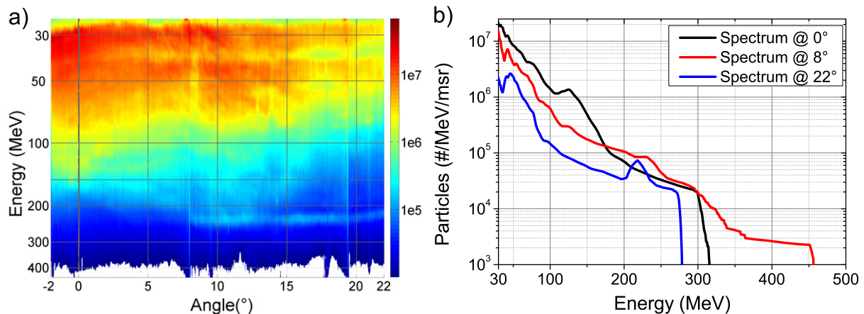
Figure 1. (a) Angularly resolved carbon spectrum measured with the iWASP in the horizontal plane of the ion beam accelerated from a 200 nm diamond target. The laser and target normal is at 0°. (b) Line-outs taken along angles 0°, 8° and 22° from the spectrum displayed in (a). The line-outs mimic spectral measurements of a Thomson parabola at these angles and show for each angle a different high-energy cutoff and different numbers of particles accelerated.
