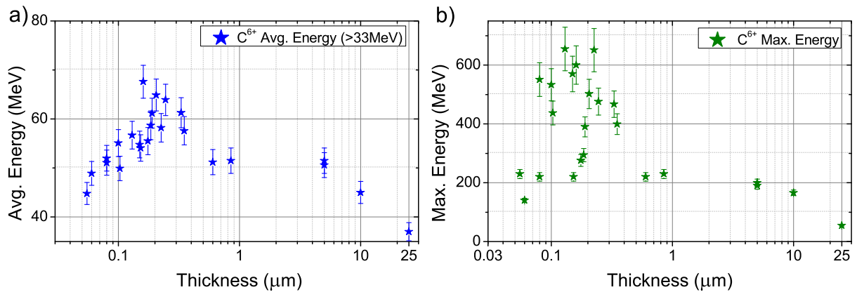
Figure 3. (a) The measured average carbon C^{6+} particle energy above the detection threshold of 33 MeV and (b) the maximum particle energy as a function of target thickness for 50 nm to 25 \mu\text{m} encompassing BOA ( <700 nm) and TNSA ( \gg 700 nm) dominated acceleration regimes. Error bars are given by the resolution limit of the iWASP (see [31] for details).
