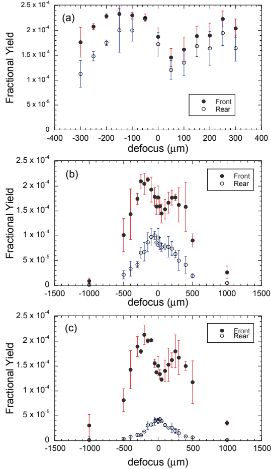
FIG. 3: (Color online) K\text{-}\alpha fractional yields for front (solid disks) and rear (open circles) spectrometers as a function of defocus for a) 10\ \mu\text{m} , b) 25\ \mu\text{m} and c) 50\ \mu\text{m} Ti foils. Positive defocus means the focus is in front of the target. Error bars are standard deviations. Note the different spatial scale for the 10\ \mu\text{m} case.
