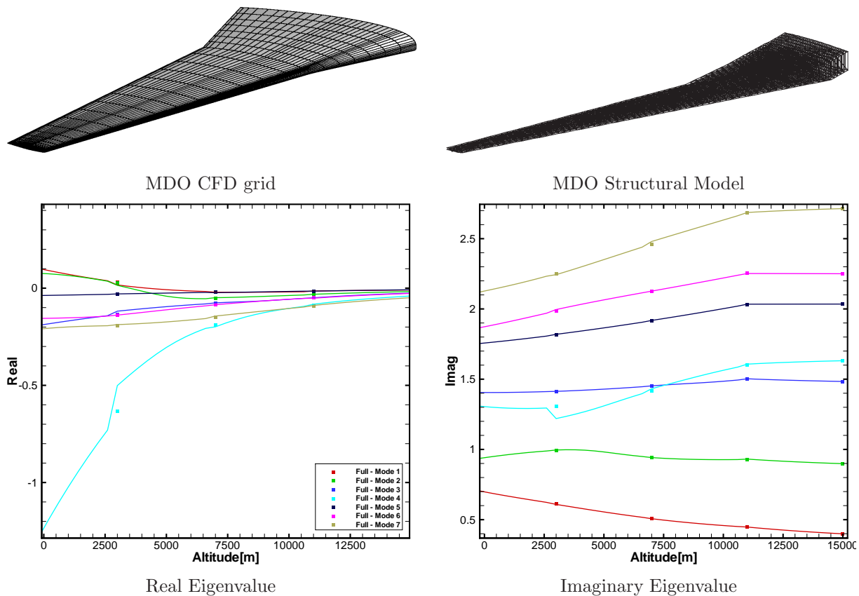
Figure 5. MDO Wing
