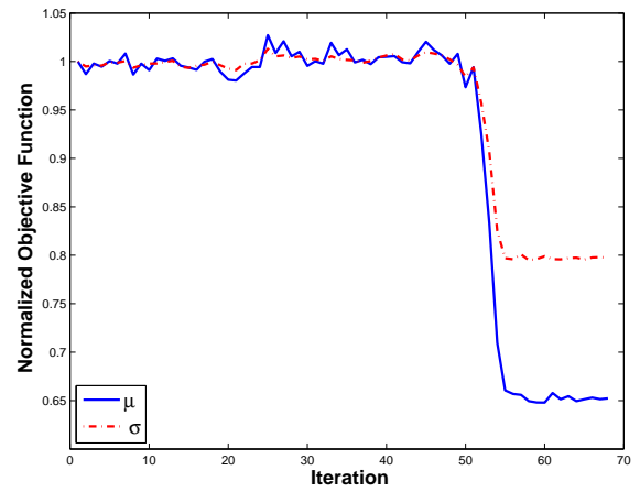
(b) Optimization Convergence - Std. Dev. bias
