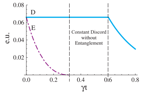
FIG. 2 (color online). Dynamics of entanglement (violet dash-dotted line) and quantum discord (blue solid line) as a function of \gamma t for c_1(0) = 1 , c_2(0) = -c_3 , and c_3 = 0.3 .
