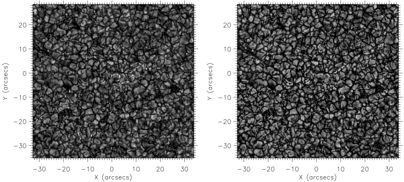
Figure 1. Simultaneous ROSA images acquired through G -band (left) and 4170 \text{ \AA} continuum (right) filters at 14:06:21 UT on 2009 May 28. Axes are in heliocentric arcseconds. Note the abundance of MBPs, particularly visible as intensity enhancements in the G band.
