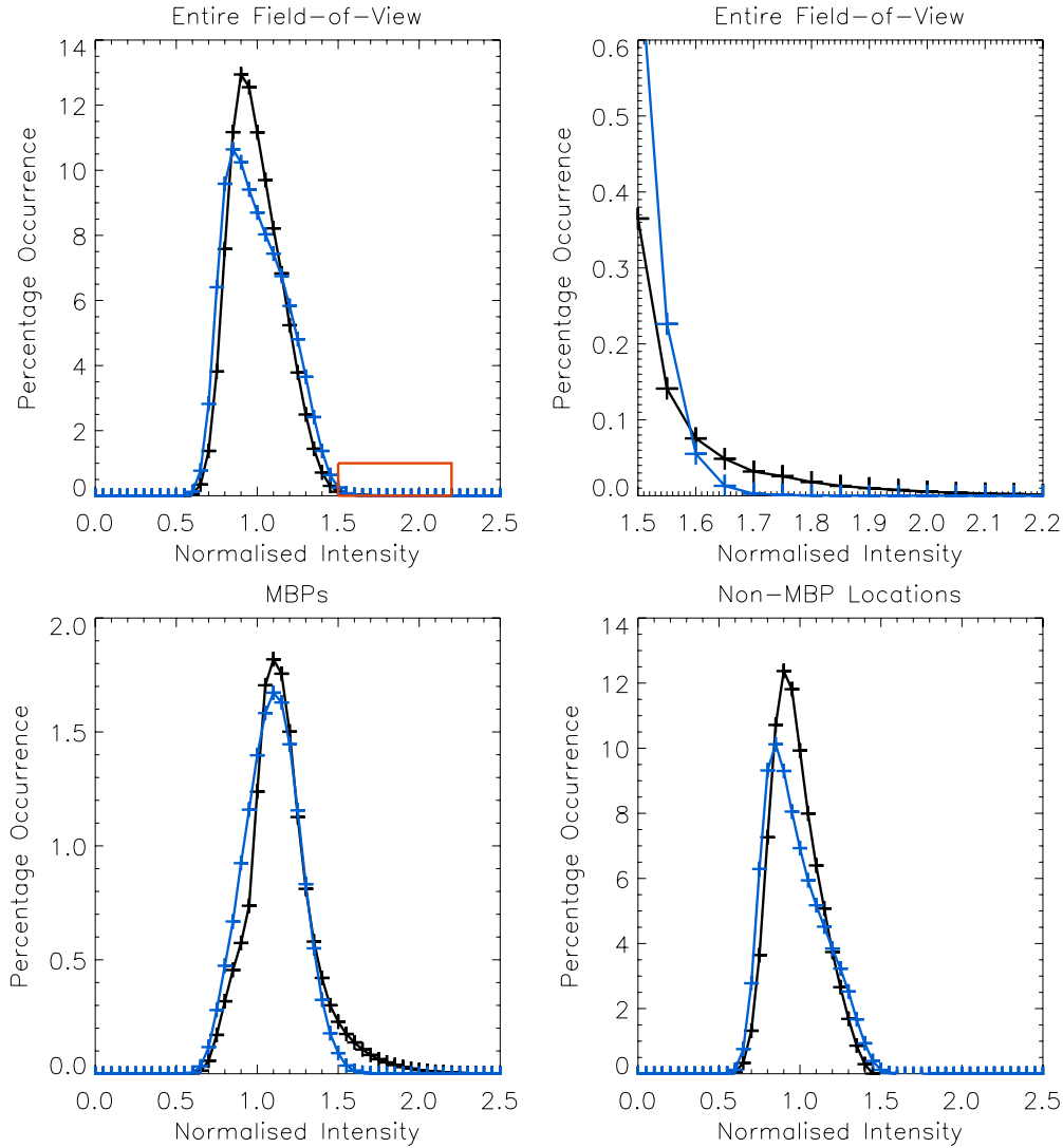
Figure 2. Upper left: histograms of the number of pixels, as a percentage of the total number of pixels, vs. their normalized intensity in the G -band (black) and 4170 \text{ \AA} continuum (blue) filtergrams, evaluated over the entire 61 minute duration of the data set ( 7.0 \times 10^9 individual pixels). Upper right: a zoom-in of the intensity occurrences contained within the red box in the left panel. G -band intensities display an extended tail, well above the 4170 \text{ \AA} continuum maximum, as a result of the presence of MBPs. Lower left: occurrence of intensities for isolated MBP structures, clearly displaying excess high-intensity measurements for G -band observations, also apparent in the upper-right panel. Lower right: intensity histograms for regions of the field of view not containing MBP structures. A narrowing of the 4170 \text{ \AA} continuum profile near its maximum occurrence, caused by the removal of MBP intensities, directly results in the reduction of its positive transmission skewness.
