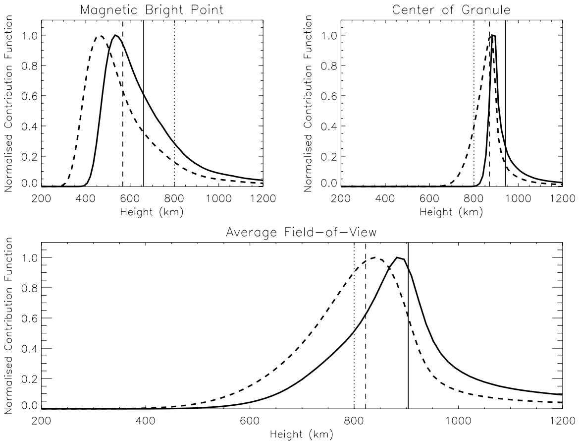
Figure 5. Normalized filter contributions as a function of atmospheric height for G -band (solid line) and 4170 \text{ \AA} continuum (dashed line) bandpasses. The upper-left panel displays the contribution functions for a typical MBP, with the upper-right panel presenting contributions arising from the center of a granular cell. The bottom panel represents the contribution functions following a spatial averaging of the entire simulated field of view. A peak separation is clearly visible in the MBP case, while a peak overlap is present for the granular cell. However, due to an extended tail in all G -band contribution functions, a measurement of the center-of-gravity separation still yields a height difference in the case of a granular cell, even when the contribution peaks overlap. The atmospheric heights corresponding to the center of gravity of the G -band and 4170 \text{ \AA} continuum contribution functions, in addition to the location of the visible solar surface, are represented in each panel by solid, dashed, and dotted vertical lines, respectively. A two-dimensional representation of these methods are shown in Figure 6.
