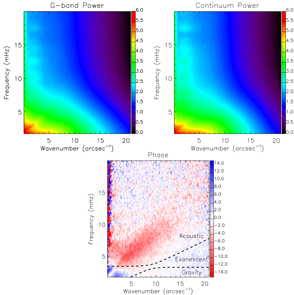
Figure 7. Power spectra of the G -band (upper left) and 4170 \text{ \AA} continuum (upper right) observations as a function of frequency and spatial wavenumber. The color scale represents the power (in orders of magnitude) above the quiescent background. The lower panel shows the phase delay between the G -band and 4170 \text{ \AA} continuum oscillations as a function of frequency and spatial wavenumber. The color scale is in degrees, where positive and negative values indicate that the G band leads, and trails, the 4170 \text{ \AA} continuum, respectively. Limiting curves for acoustic- and gravity-wave regimes are displayed as dashed lines, with an evanescent region sandwiched between the acoustic and gravity regimes. A similar figure, only for the simulated time series, is shown in Figure 8.
