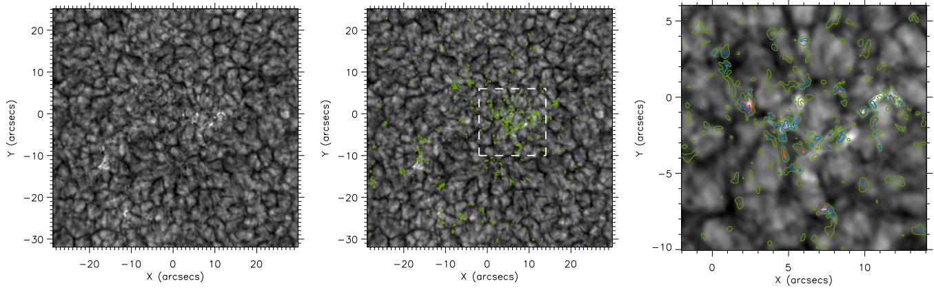
Figure 3. G -band intensity image, averaged over the entire 61 minute duration of the time series (left). Green contours (middle and right panels) highlight the locations where waves are observed to propagate (i.e., a non-zero phase shift) between the G -band and 4170 Å continuum bandpasses. These contours are generated irrespective of oscillation frequency, and so cannot be used to pinpoint where particular periodicities exist. Dashed white lines outline a sub-field, which is magnified in the right panel. Blue and red contours in the right panel represent propagating wave power which is four and six orders of magnitude, respectively, above the background. A preferential existence of propagating waves is found in locations of increased magnetic field strength, such as MBPs.
