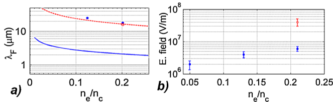
FIG. 2 (color online). (a) Comparison between the experimental spatial period of the filaments with Eqs. (3) (blue solid line) and (4) (red dashed line). (b) Modulation of the electric field across the filamented region as a function of the background electron density with (blue full circles) and without (red empty circle) the insertion of a RPP.
