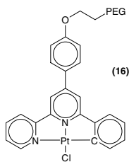
Fig. 16 An example of a Pt(II) complex with sensing properties for protein surfaces
