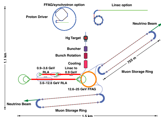
Figure 1: The IDS Baseline Neutrino Factory Design.
