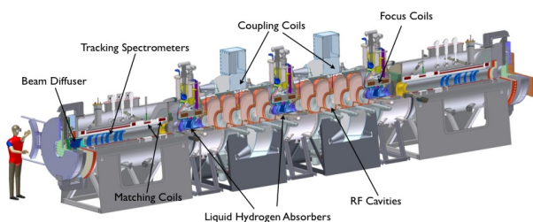
Figure 2: The Muon Ionisation Cooling Experiment, MICE.
