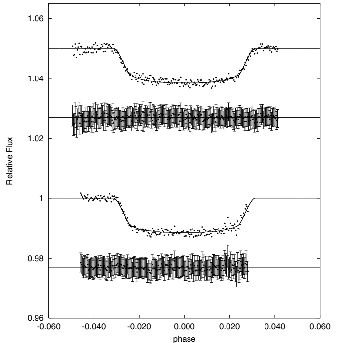
Fig. 1. RISE light curves of WASP-3 taken on 18 May 2008 ( upper , offset by 0.05) and 4 Sep. 2008 ( lower ) shown in 1 min bins with the best fit model from the MCMC analysis overplotted. Residuals are shown offset along with their error bars after rescaling so \chi_{\text{red}}^2 = 1 and to account for red noise.
