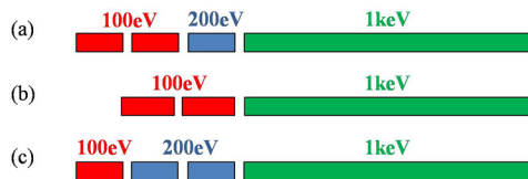
Figure 1: Schematic of the three alternative modulator configurations considered for FEL-3.
