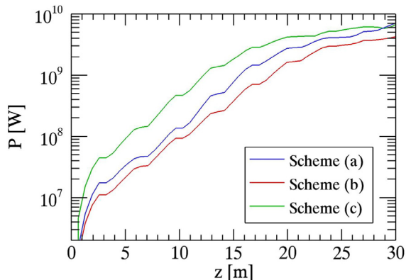
Figure 2: Radiation power as a function of distance through the radiator for time-dependent Genesis 1.3 simulations of the three modulator configurations
