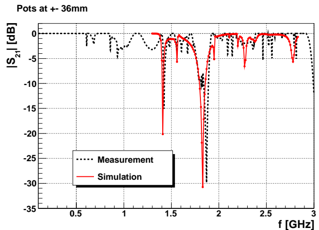
Figure 3: Modulus of the transmission scattering parameter S_{21} as measured and simulated with HFSS, for a RP retracted position at 36 mm from the wire (i.e. form the beam)
