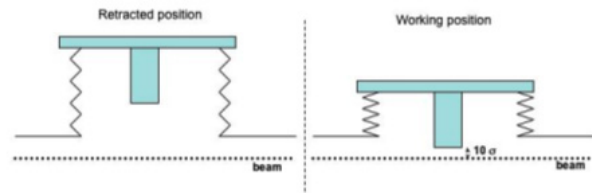
Figure 1: Roman pot detector concept.
