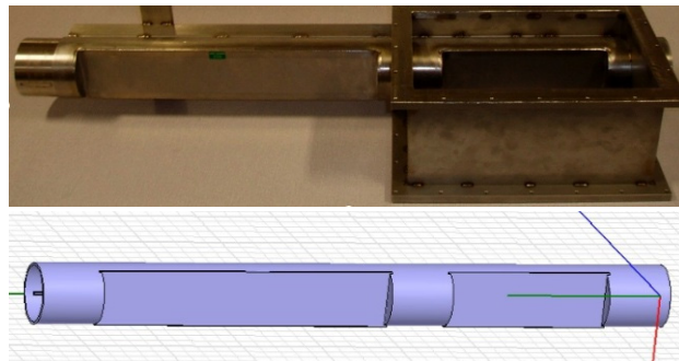
Figure 1: FP420 double-pocket prototype.
