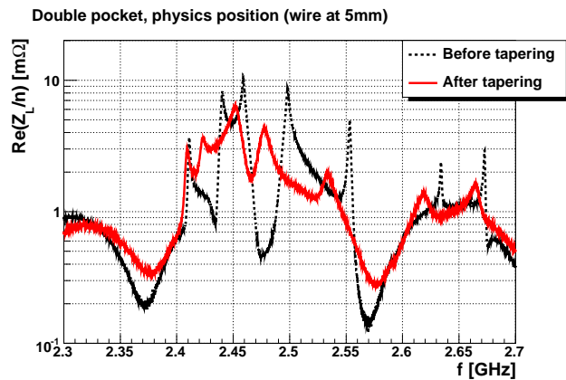
Figure 3: Longitudinal impedance of a FP420 double-pocket pipe in data taking position, as measured with and without copper tapering (see text).
