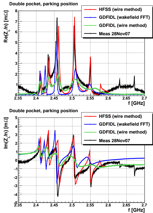
Figure 2: Longitudinal impedance of a FP420 double-pocket pipe in parking position calculated with simulations (HFSS and GDFIDL) and compared to laboratory experiments.
