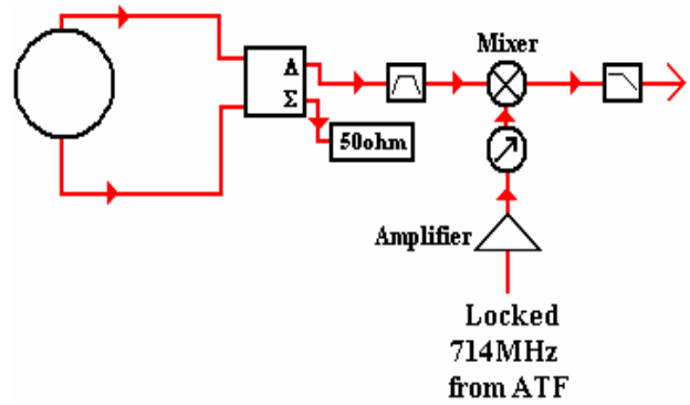
Figure 3: Schematic of BPM signal processor.
