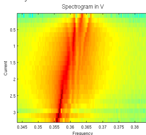
Figure 4: Head-Tail modes as a function of current in the vertical plane (see text for explanation).
