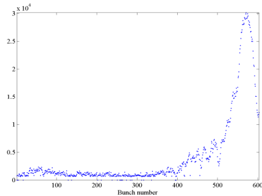
Figure 6: Amplitude of vertical oscillations along the bunch train.
