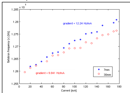
Figure 7: Tuneshift with current with ID open and in-vacuum IDs closed to 7 mm gap. Horizontal plane.
