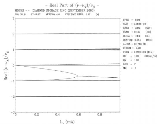
Figure 3: Single bunch TMCI in the vertical plane as simulated by MOSES.
