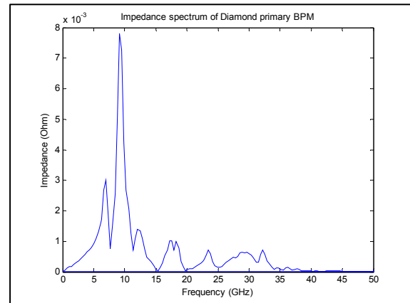
Figure 8: Longitudinal impedance at the primary BPM block.
