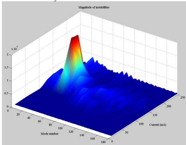
Figure 5: Colour plot of the vertical mode excitation vs current for a 2/3 fill, chromaticity two in both planes.
