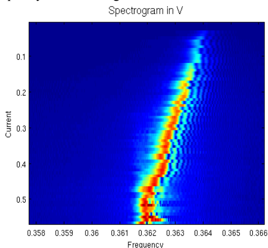
Figure 2: Vertical tunes with current and TMCI detected in the vertical plane.
