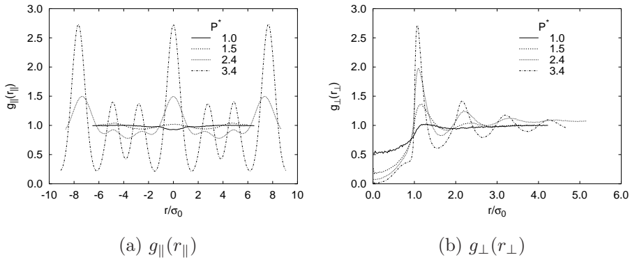
Figure 10: Pair correlation functions g_{\perp}(r_{\perp}) and g_{||}(r_{||}) resolved parallel and perpendicular to the director for PHGO model particles with elongation k = 5 .
