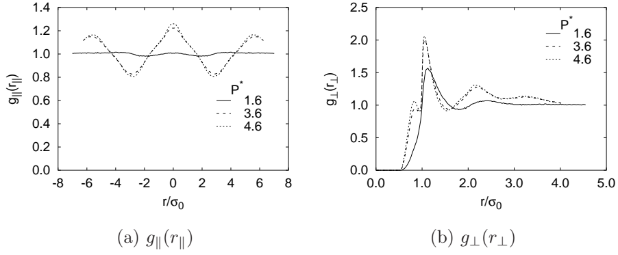
Figure 9: Pair correlation functions g_{\perp}^{\text{mol}}(r_{\perp}) and g_{||}^{\text{mol}}(r_{||}) resolved parallel and perpendicular to the molecular orientation for PHGO particles with elongation k = 4 .
