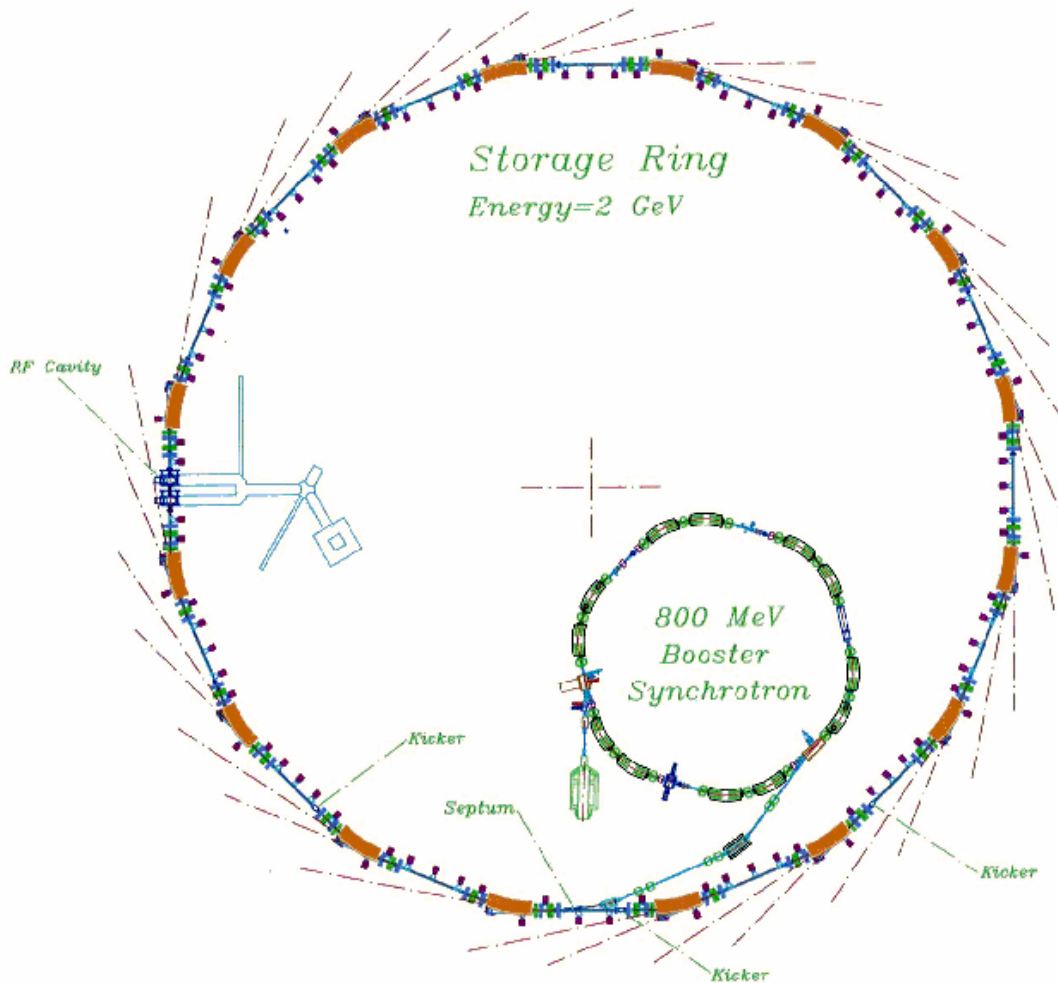
Figure 3: arrangement of the storage ring of SESAME machine
