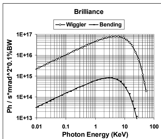
Figure 4: Brilliance of the synchrotron radiation emitted from the stored beam in the bending and wigglers.
