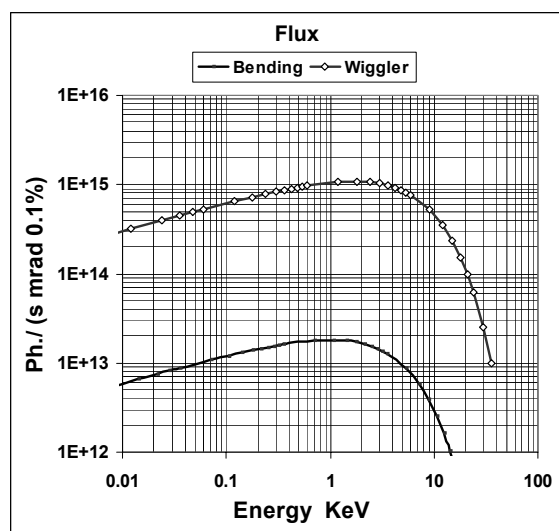
Figure 3: Flux of the synchrotron radiation emitted from the stored beam in the bending and wigglers.
