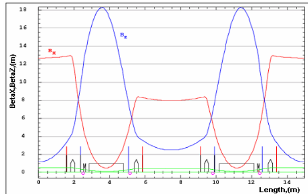
Figure 1: Optical functions of SESAME lattice, The green line represents dispersion. Horizontal and vertical correctors are represented by red and blue respectively.
